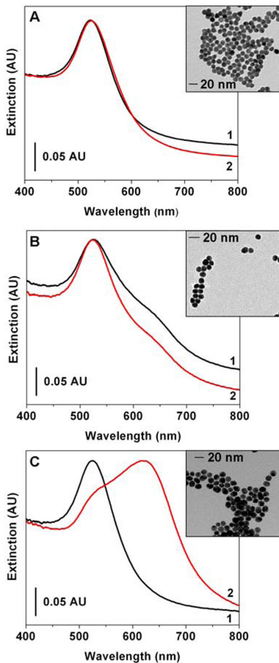
Figure 1. Characterization of gold nanoparticles using LSPR spectroscopy and TEM (inset) (A) Au@citrate ( d = 13.3 \pm 0.6 nm) have an extinction maximum located at (1) 523.3 nm in water and (2) 524.8 nm in buffer. (B) Au@COOH ( d = 10.9 \pm 1.8 nm) have an extinction maximum located at (1) 521.5 nm in water and (2) 522.3 nm in buffer with a slight shoulder located \sim 625 nm in both spectra. (C) Au@NH 2 ( d = 13.8 \pm 2.0 nm) have an extinction maximum located at (1) 524.0 nm in water and (2) 617.5 nm with a shoulder at the original extinction maximum \sim 525 nm in buffer. In all buffer spectra, 10 mM tetraborate buffer (pH = 9.3) is used.
