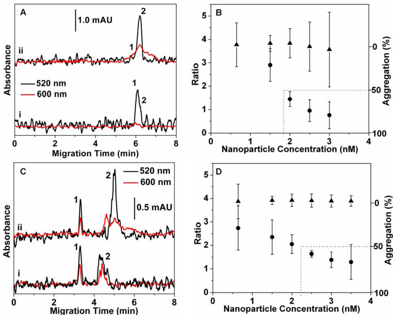
Figure 2. Dual-wavelength PDA detection of nanoparticles in a capillary
