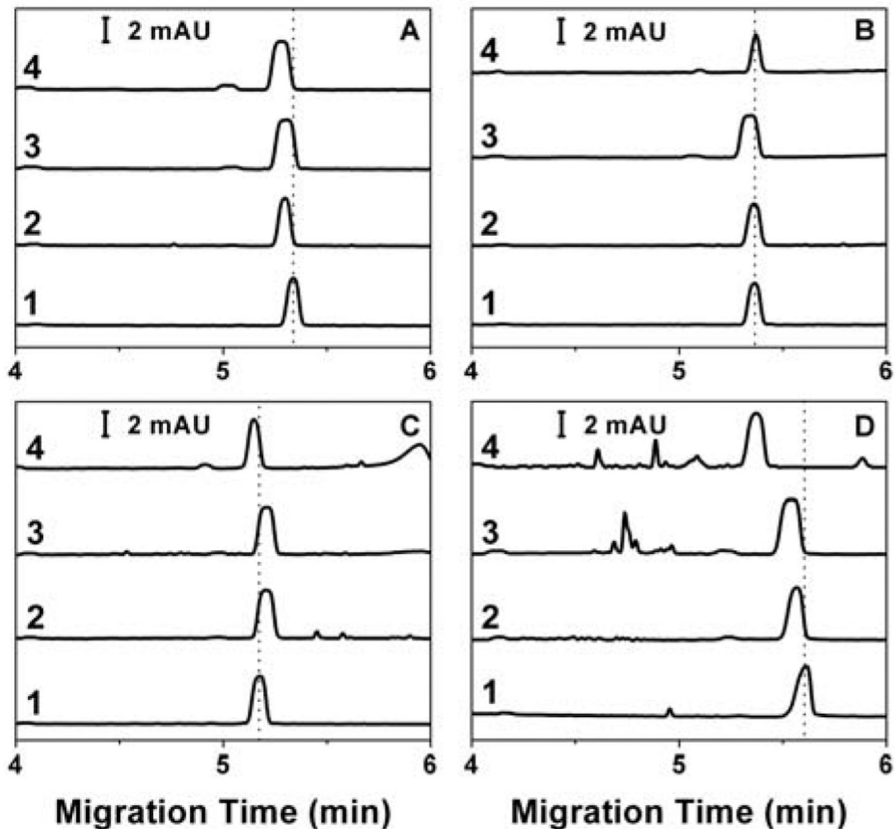
Figure 3. Evaluation of trends in the migration time of pyrocatechol as a function of nanoparticle concentration
