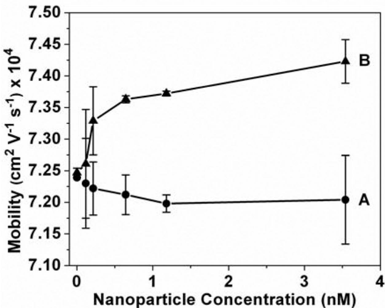
Figure 4. Comparison of dopamine mobility versus nanoparticle concentration
