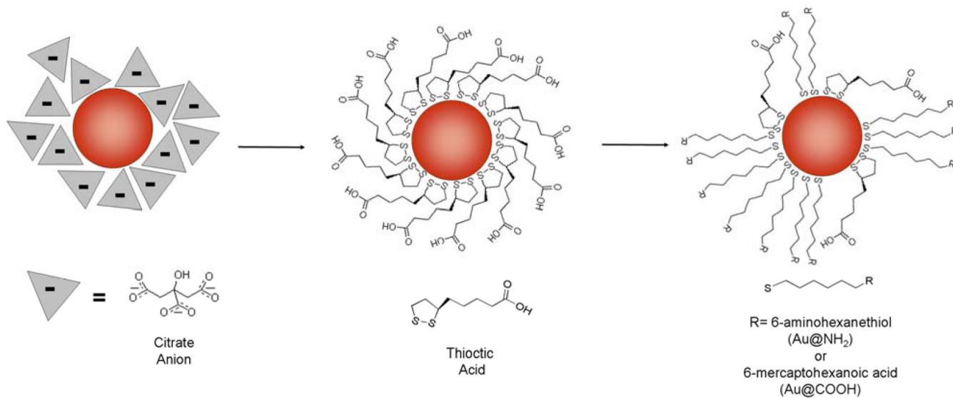
Scheme 1. Ligand exchange reaction on gold nanoparticles
