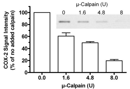
Figure 7 COX-2 degradation by \mu -calpain in vitro . Control cells were treated with LPS/IFN for 24 h to induce COX-2. Extracts were then mixed with the indicated units of porcine \mu -calpain, in calpain reaction buffer, incubated 30 min, and then denatured for western blotting. A representative blot of COX-2 is shown. Bars represent the average COX-2 signal intensity \pm SE of 3 independent cultures for each point, as a percent of the value without added calpain.
