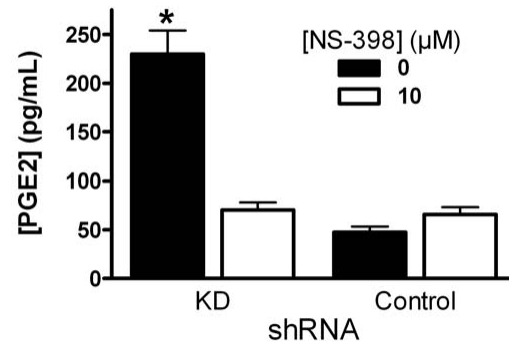
Figure 2 Effect of PIN1 knockdown on prostaglandin E2. COX-2-dependent prostaglandin E2 (PGE2) production was measured in cells treated with LPS, IFN, 20 \mu M arachidonic acid and 1 \mu M SC-560, with or without 10 \mu M NS-398. Bars represent mean + SE concentration of prostaglandin E2 in medium for 5 cultures in each group. *:p < 0.05 for between KD and Control cells treated in the same way.
