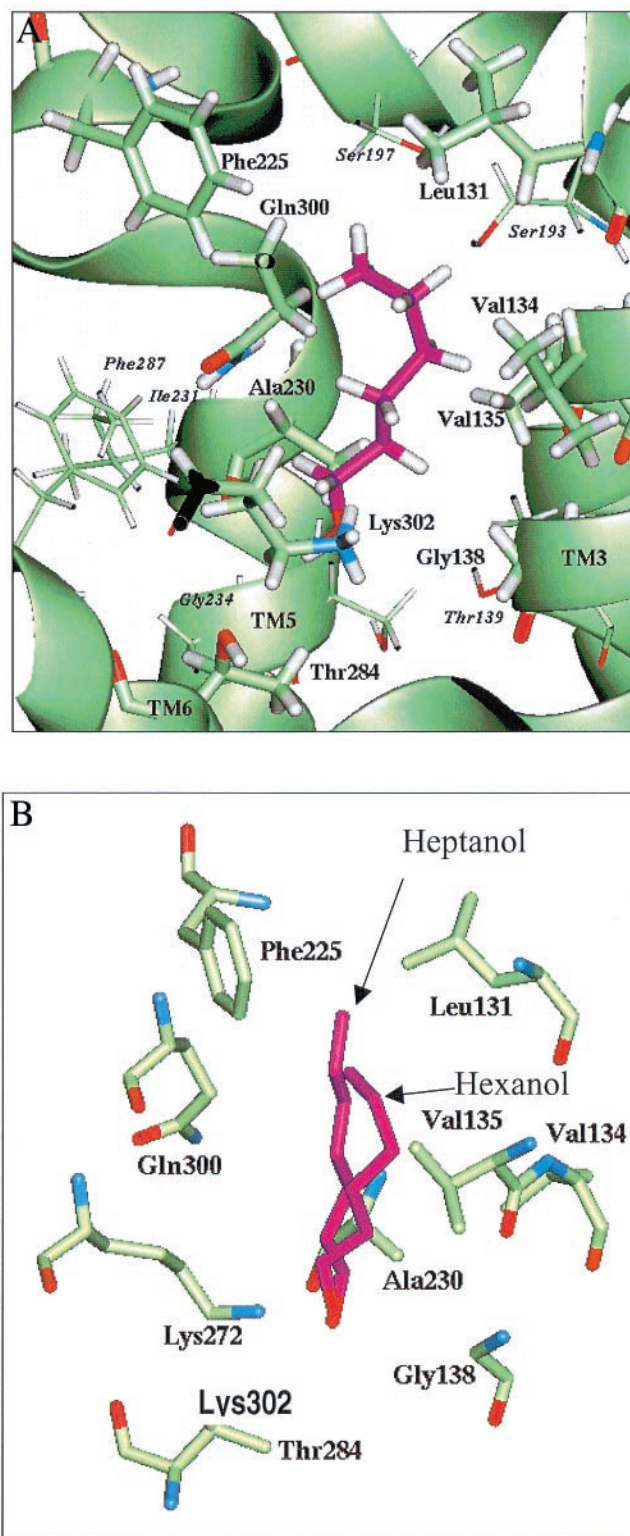
Fig. 3. Predicted recognition site for hexanol and heptanol in mouse OR S25. Residues within 3 Å of the ligand (hexanol in purple) are displayed as thicker with labels in bold font. Residues within 3–5 Å of the ligand have labels in italics. Lys-302 forms a weak hydrogen bond to the hydroxyl group of the alcohols. Phe-225 and Leu-131 seem to limit the chain length suitable to the binding site. TM 3–7 have residues directly involved in binding. (A) Longitudinal view. (B) Detail view. Hydrogen atoms were suppressed.
