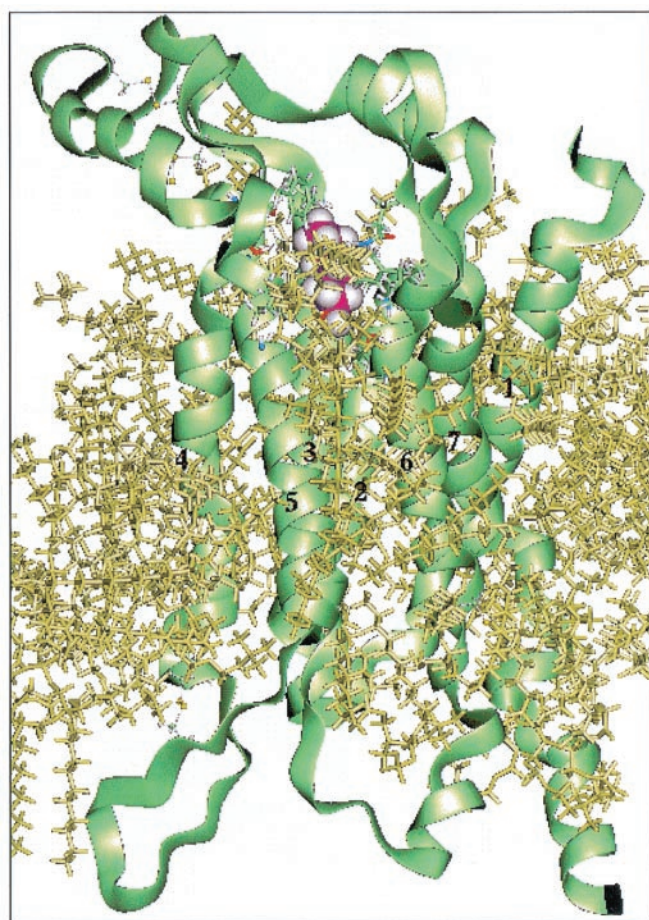
Fig. 1. Predicted structure for mouse OR S25 with predicted binding site for hexanol (purple). The membrane is represented by a barrel of dilauroylphosphatidyl choline bilayers (yellow) surrounding the TMs 1–7. The disulfide bonds were assigned between Cys-107 to Cys-209, Cys-132 to Cys-192, Cys-199 to Cys-219, and Cys-157 to Cys-171.
