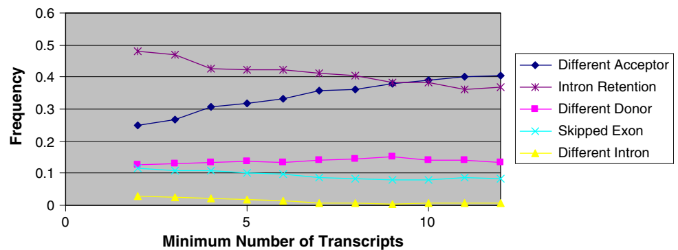
Fig. 10 Relative frequencies of different types of alternative splicing events. The frequencies of different alternative splicing events were computed from the alignment of 563,251 transcripts with corn genomic sequences. 289,608 mapped transcripts are from Ceres libraries, the other 273,643 transcript sequences were downloaded from GenBank
