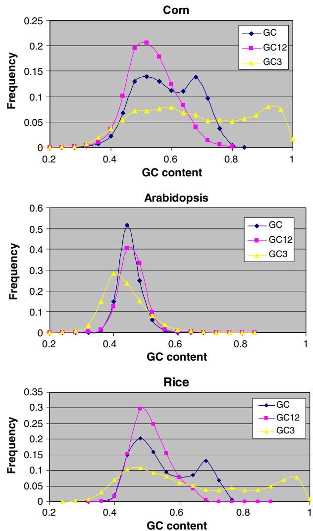
Fig. 3 Distribution of GC in the coding region of corn, Arabidopsis and rice. The GC content in the coding region of corn cDNAs is bimodal and the high GC content can be explained by the abundance of GC in the third position of the codons. A similar result is observed for rice but Arabidopsis is unimodal. GC indicates the ratio of GC versus AT. GC12 represent the ratio of GC versus AT in the 1st and 2nd positions of the codons. GC3 represents the ratio of GC versus AT in the 3rd position of the codons
