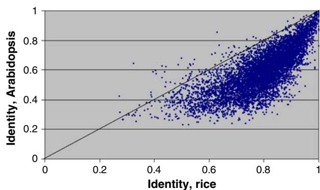
Fig. 15 Corn proteins are more similar to rice than to Arabidopsis. The few exceptions are due to genes missed in the rice annotation, random fluctuations and possible contamination of corn cDNA clones by cDNAs from other organisms. 10,084 corn proteins, TAIR Arabidopsis genome annotation and TIGR rice annotation were used for comparison. Only matches with P -value \leq 1.e-10 , covering at least 70% of the protein length are shown in the plot
