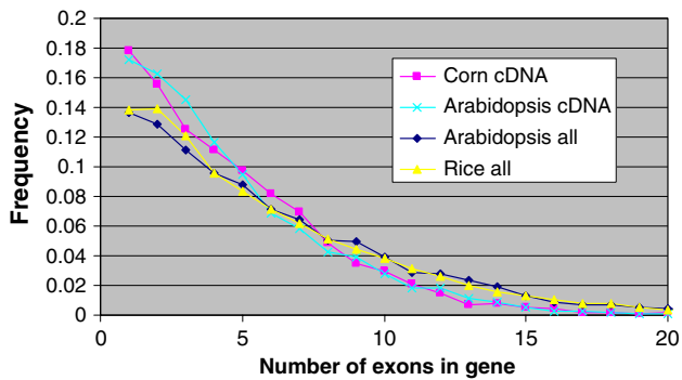
Fig. 6 Distribution of the exon number in corn, Arabidopsis and rice genes. 2793 of 10,084 full-length corn clones were mapped to corn genomic sequences of >20,000 bps to ascertain the number of exons. This subset is biased towards shorter genes which may overestimate frequencies of genes with a smaller number of exons and underestimate frequencies of genes with a larger number of exons. This effect can be seen in the distributions for Arabidopsis genes: one was obtained using Arabidopsis cDNA clones produced by a similar technology (Arabidopsis cDNA) and the other derived from all genes in the TAIR genome annotation having mRNA support (Arabidopsis all). Distribution of exons in rice genes were obtained from 23,721 genes with mRNA support from TIGR rice genome annotation, release 6 and are shown for comparison
