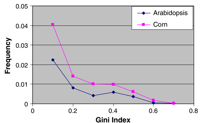
Fig. 9 Gini index for corn and Arabidopsis introns. 96% of Arabidopsis introns and 92% of corn introns have a Gini index equal to 0 meaning that there are no variants (the data point is not shown). A larger Gini index in corn means that corn transcripts are more variable
