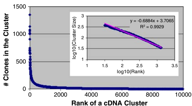
Fig. 1 Distribution of the number of clones (5' ESTs) among clusters represented by a set of 10,084 full-length corn cDNA clones. Relatively few genes have many ESTs whereas many have only one or few ESTs. The distribution can be approximated by a power function (inset; linear function in log scale)
