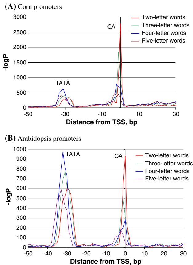
Fig. 12 The most significant words in corn (a) and in Arabidopsis (b) promoters. The analysis is performed on a subset of 5,200 corn promoters and 5,050 Arabidopsis promoters that have TSS predicted by at least four 5' ESTs. For Corn, there is a prominent CA peak at the TSS and a smaller TATA motif at position -30. This is in sharp contrast to Arabidopsis where TATA is more frequent than CA
