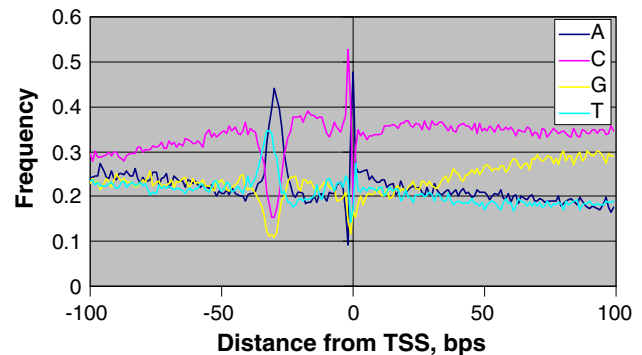
Fig. 11 Distribution of nucleotides around the Transcription Start Site of corn based on 5,200 promoters that have TSSs predicted by at least four 5' ESTs. There is a peak of A/T at position -30 and a peak of C/A just prior to the TSS
