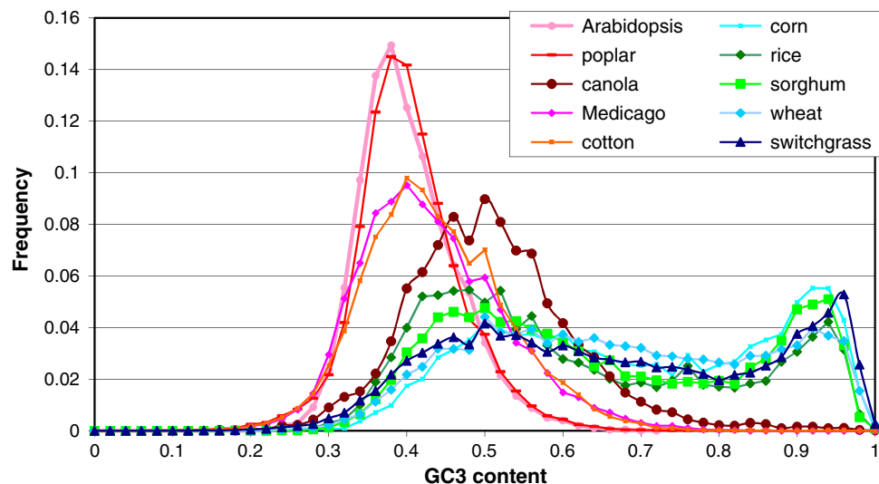
Fig. 4 Distribution of the GC content in the third codon position of CDSs of different plant species. All grasses have a broad distribution with two peaks whereas the dicots have a unimodal distribution. All CDS sequences except corn (we used sequences described in this paper) and Arabidopsis (we used TAIR annotation) were downloaded
