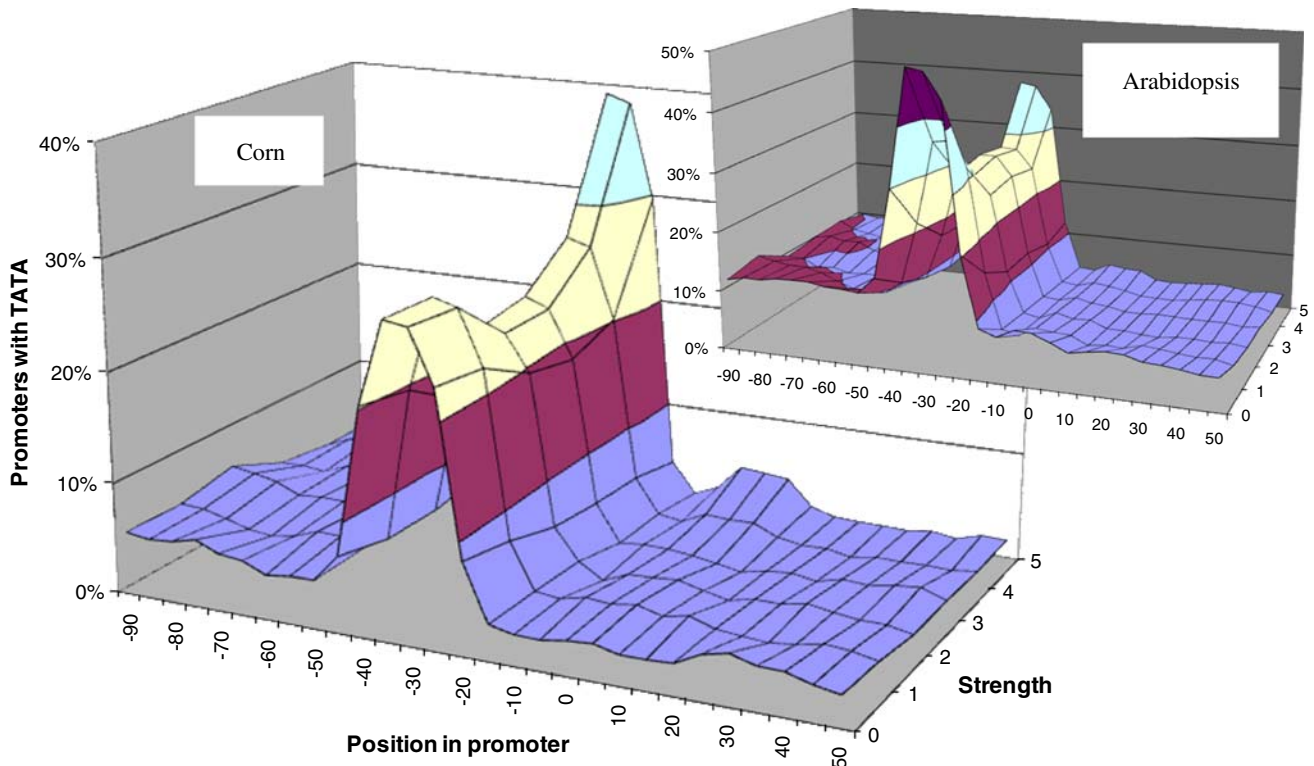
Fig. 13 Frequency of a TATA box in promoters of different strengths. Strong and weak promoters have a TATA box more often than genes with average expression. In corn, TATA boxes are more
