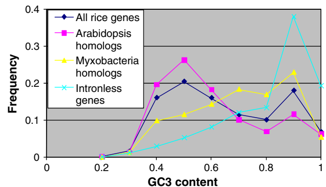
Fig. 5 Distribution of the GC content in the third codon position among different groups of rice genes. Only those genes which have mRNA evidence in TIGR version 5 annotation (total 23,721 genes) were considered. GC3 distribution of these genes has two peaks at about 0.5 and 0.9. Genes without introns (4,452) are more prevalent in the high GC3 peak. Genes sharing similarity with Arabidopsis (blast P -value < 1.e-50 , best reciprocal hit, 7,924 genes) are mostly in the lower GC3 peak whereas genes (1,664) similar to Myxobacteria (blast P -value < 1.e-3 and not matching Arabidopsis) are mostly in the high GC3 peak. 17,100 known protein sequences of the order Myxococcales from GenBank were used for comparison
