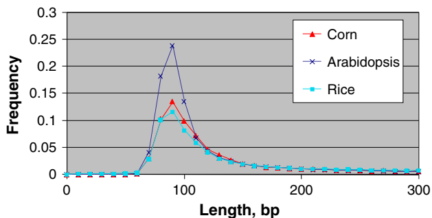
Fig. 7 Intron length distribution in corn, Arabidopsis and rice. Introns in both the coding and non-coding parts of the mRNA were used in this analysis. All three species have similar modes for intron length, although corn and rice genes have longer introns in average
