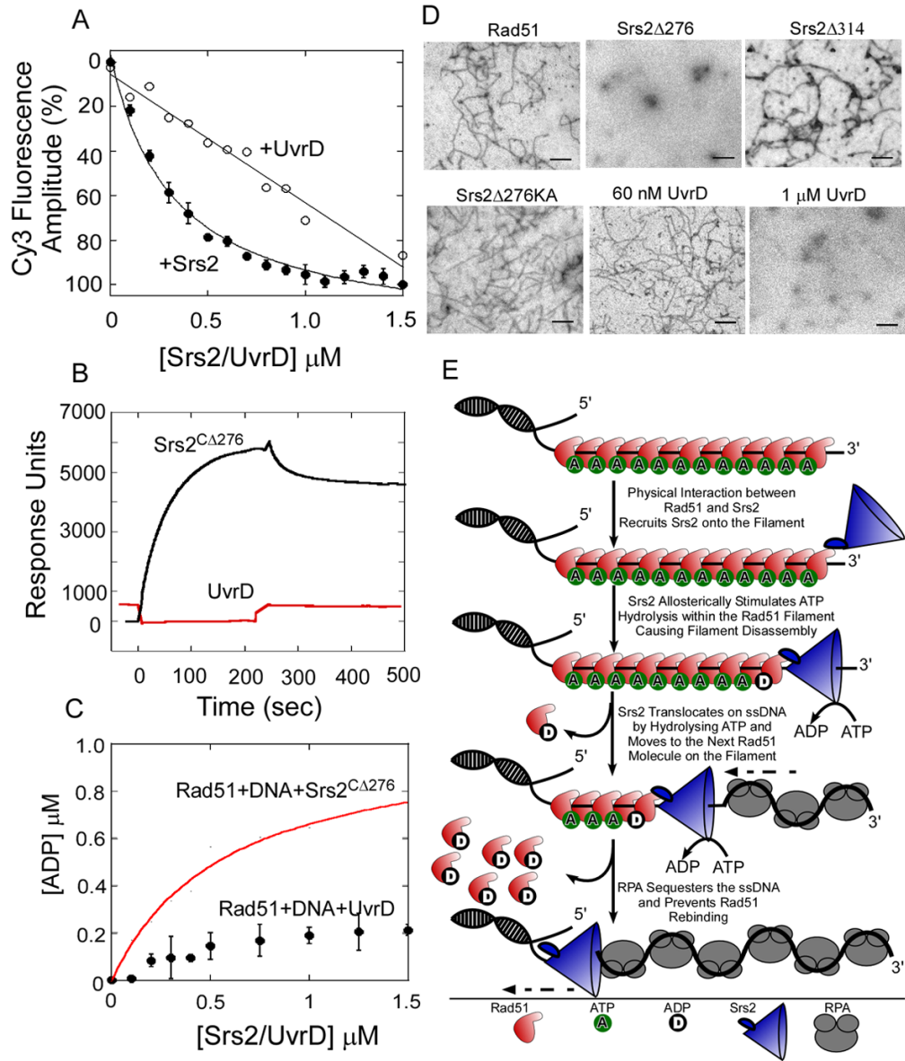
Figure 7. Mechanism of Clearing Rad51 Filaments by Srs2
