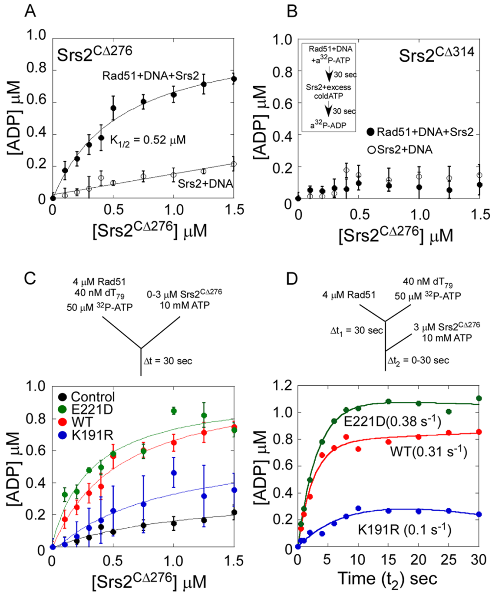
Figure 6. Srs2 AllostERICALLY Stimulates ATP Hydrolysis within the Rad51 Filament Thereby Promoting Filament Disassembly (A) Srs2^{C\Delta 276} stimulates the ATP hydrolysis within a Rad51-DNA filament. Preformed Rad51-DNA- ^{32}P -ATP filaments were mixed with increasing concentrations of Srs2^{C\Delta 276} and excess unlabeled ATP and the amount of ^{32}P -ADP formed was measured. A stimulation of ATP hydrolysis is observed within the Rad51 filament ( \bullet ), and the Srs2^{C\Delta 276} dependence of this stimulation yields a K_{1/2} = 0.53 \pm 0.13 \mu M . The control experiment done in the absence of Rad51 ( \circ ) shows the background level of ^{32}P -ATP hydrolyzed by Srs2 when a 500-fold excess of unlabeled ATP is present. (B) Srs2^{C\Delta 314} does not stimulate ATP hydrolysis within a Rad51-DNA filament. The insert shows a schematic representation of the ATPase assays described in A and B. (C) Rad51 filaments were formed on ssDNA ( dT_{79} ) with either wild-type Rad51 (red), Rad51-K191R (blue), or Rad51-E221D (green) proteins in the presence of radiolabeled ATP. Srs2^{C\Delta 276} stimulates the rate of ATP hydrolysis when added to these filaments along with excess unlabeled ATP. The Srs2^{C\Delta 276} dependence of this stimulation
