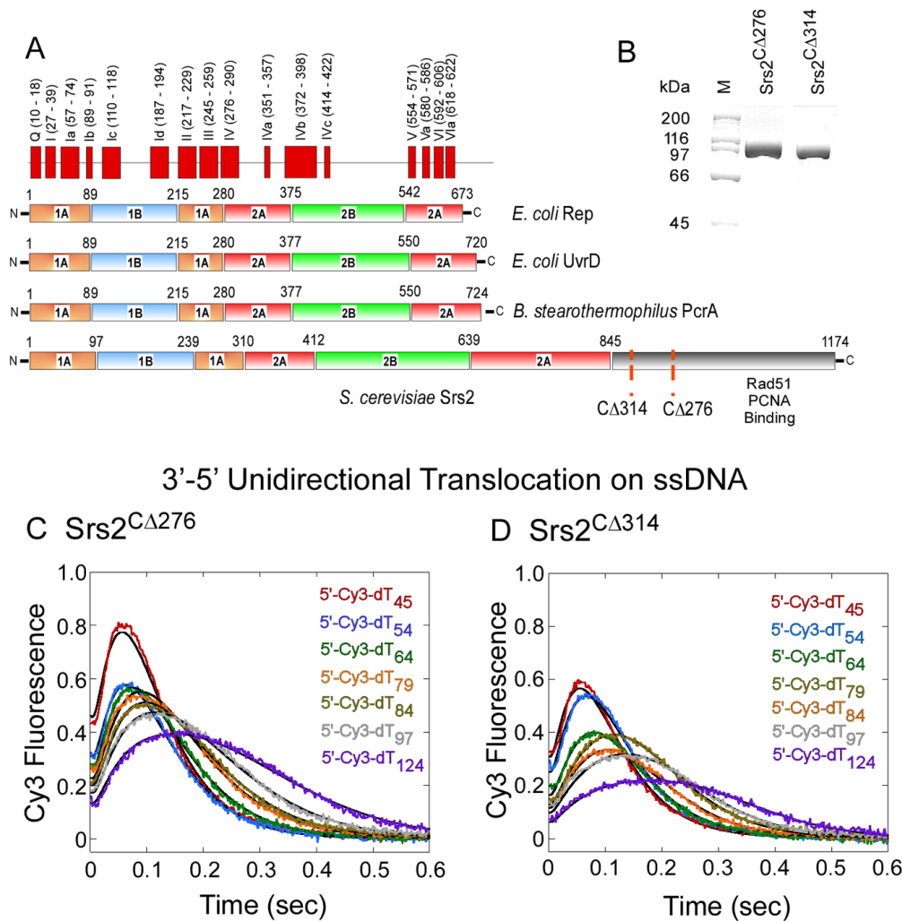
Figure 1. Srs2 Translocates Unidirectionally on ssDNA
