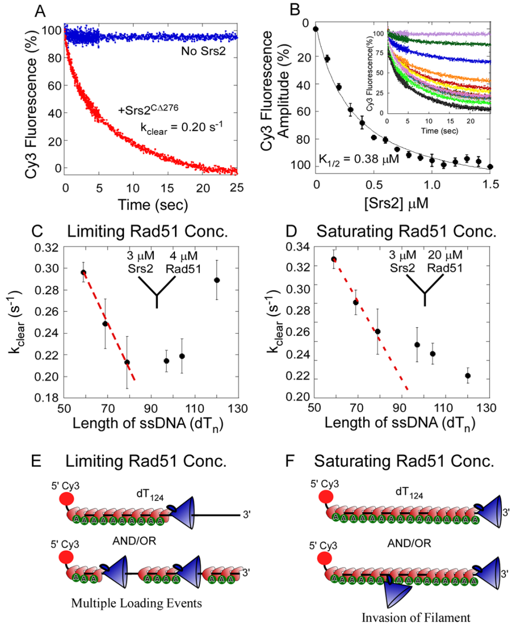
Figure 3. Srs2 Clearing of Rad51 Filaments
