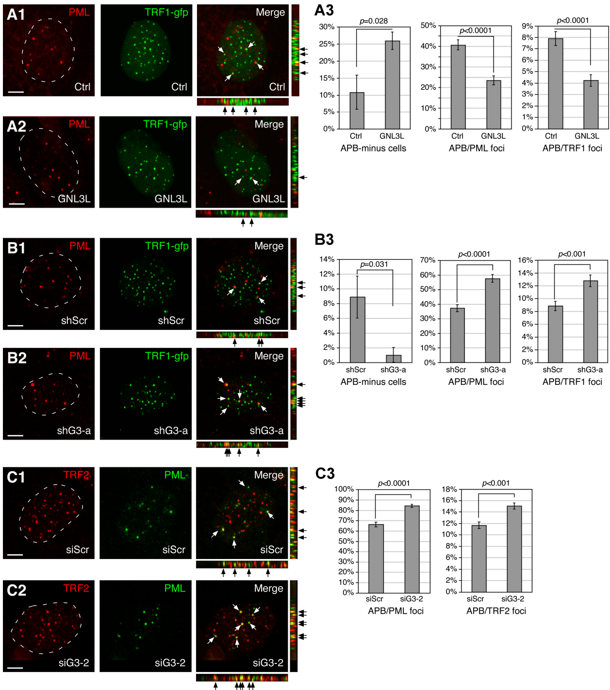
Figure 4. GNL3L negatively regulates APB formation in U2OS cells. (A) APB formation in U2OS cells was scored by colocalization of TRF1-gfp and PML bodies in the control (A1) or GNL3L-overexpression U2OS cells (A2). Serial confocal images of 1- \mu m thickness were collected at 0.5- \mu m intervals and reconstructed along the X-Y, X-Z, and Y-Z planes for individual cell. Arrows indicate overlapped spots. (A3) Coexpression of GNL3L increases the percentage of APB-minus cells, and decreases the ratios of APB/PML bodies and APB/TRF1 + foci. (B) Colocalization of TRF1 + foci and PML bodies was measured in control (shScr, B1) or GNL3L knockdown (shG3-a, B2) U2OS cells. (B3) GNL3L knockdown increases colocalization of TRF1 foci and PML bodies. (C) GNL3L knockdown by siG3-2 promotes APB formation in U2OS cells, as scored by colocalization of TRF2 + foci and PML bodies.
