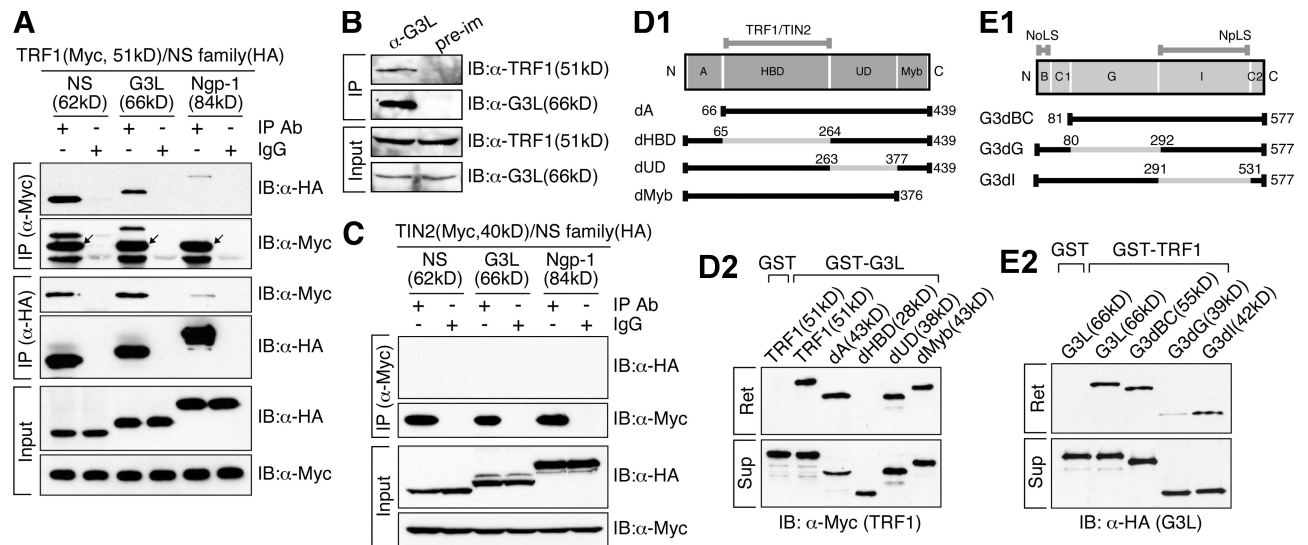
Figure 1. Interaction between TRF1 and GNL3L is mediated by the homodimerization domain of TRF1 and the GTP-binding domain of GNL3L. (A) Cell lysates were extracted from HEK293 cells cotransfected with Myc-tagged TRF1 and HA-tagged nucleostemin (NS), GNL3L (G3L), or Ngp-1. Protein complexes were immunoprecipitated (IP) by anti-tag antibodies and immunoblotted (IB) by the indicated antibodies. TRF1 interacts with NS and GNL3L, but not with Ngp-1. Arrows mark the precipitated TRF1. (B) Endogenous coIP confirmed that TRF1 and GNL3L co-reside in the same protein complex immunoprecipitated by anti-GNL3L antibody ( \alpha -G3L) from HeLa cell lysates. Pre-im: preimmune serum. (C) None of the NS family proteins interacts with TIN2. (D1, E1) Diagrams of TRF1 and GNL3L deletion mutants. Gray lines mark the deleted regions; numbers indicate amino acid positions. Domain abbreviations: A, acidic; HBD, homodimerization; UD, undefined; B, basic; C1 and C2, coiled-coil-1 and -2; G, GTP-binding; I, intermediate. GST pull-down assays demonstrated that the HBD domain of TRF1 (D2) and the G domain of GNL3L (E2) are required for the interaction of these two proteins. Agarose-retained (Ret) and supernatant fractions (Sup) are indicated.
