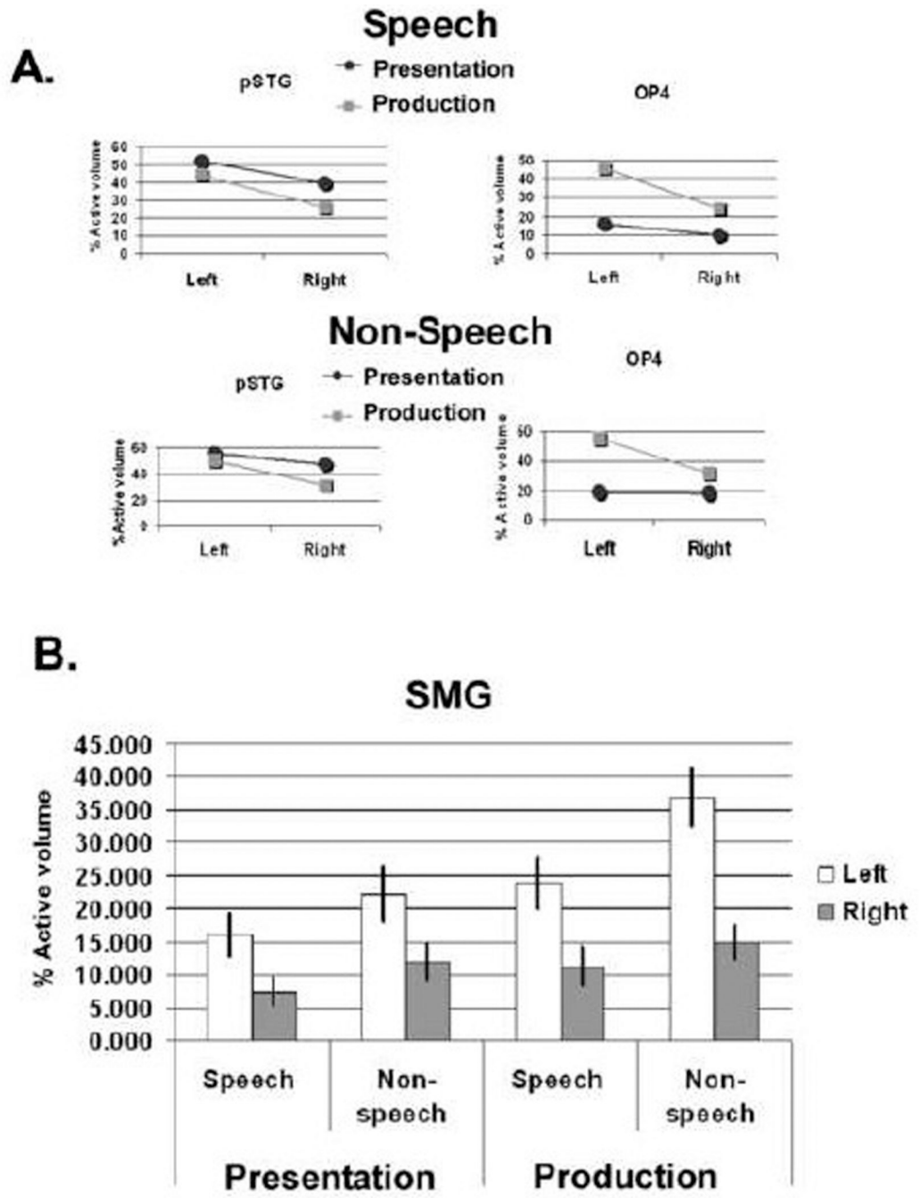
Figure 7. Mean volume of activation across ROIs for speech versus nonspeech conditions for target presentation and production. The differences were all significant at p=.01 . Error bars depict standard error of the mean.
