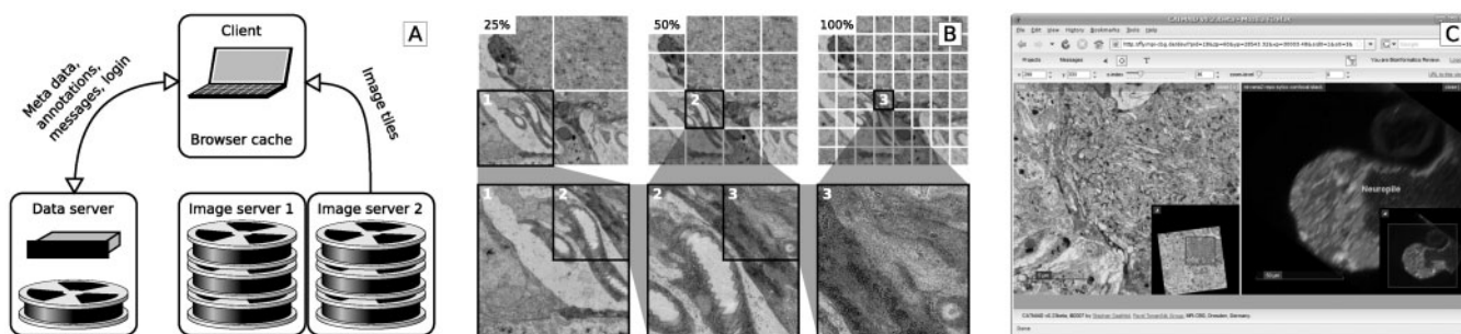
Fig. 1. (A) Sketch of the information flow between the three components of CATMAID: the central data server, the client-side user interface and several image servers. (B) Visualization of the multi-scale tiling of images. In the upper row, an exemplary ssTEM section is overlaid with the tiling grid at 25%, 50% and 100% scale. Below, exemplary tiles at the respective scale are shown (1–3). The location of a tile in the section and in lower scale tiles is indicated with the corresponding number. (C) The user interface in the synchronous navigation mode with an ssTEM dataset on the left and a relatively registered confocal stack on the right.
