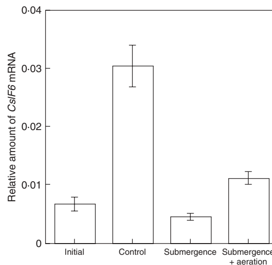
FIG. 3. Change in relative amount of CsIF6 mRNA under water. The relative amount of CsIF6 mRNA to ACT1 mRNAs in the seedlings was measured by quantitative RT-PCR. Treatments are as described in Fig. 2. Values are means \pm s.e. of triplicate assays.
