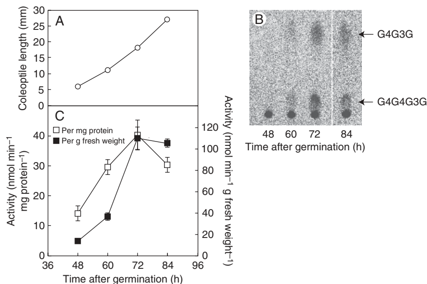
FIG. 1. Detection of \beta -1,3:1,4-glucan synthase activity in rice seedlings grown in air. (A) Length of rice coleoptiles at various growth stages. (B) \beta -1,3:1,4-glucan synthase activity in microsomes prepared from the rice seedlings grown in air was assayed using a reaction mixture containing UDP-[ 14 C]Glc as the substrate. The diagnostic oligosaccharides G4G3G and G4G4G3G are indicated, released from the \beta -1,3:1,4-glucan product by the action of lichenase followed by paper chromatographic separation. (C) \beta -1,3:1,4-glucan synthase activities per mg protein and per g fresh weight, determined based on the radioactivity of G4G3G and G4G4G3G. Values are means \pm s.e. of triplicate assays.
