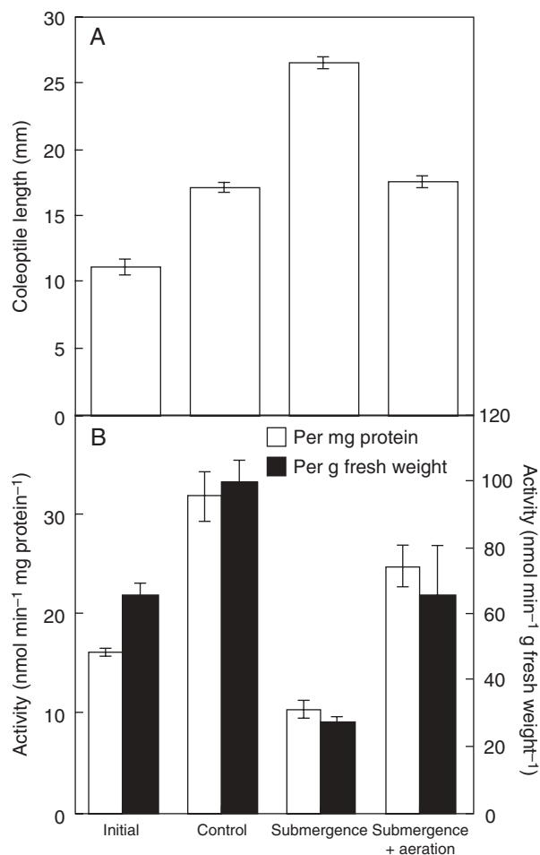
FIG. 2. Effects of submergence on \beta -1,3:1,4-glucan synthase activity. (A) Length of coleoptiles before the submergence treatment (initial), grown for 12 h under water without aeration (submergence), with aeration (submergence + aeration) and in air (control). (B) \beta -1,3:1,4-glucan synthase activities per mg protein and per g fresh weight in the seedlings. Values are means \pm s.e. of triplicate assays.
