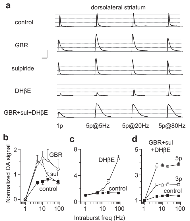
Fig. 4. The frequency-dependence of DA signals in the dorsolateral striatum in response to inhibition of DATs, dopamine D_2 -type receptors, and \beta_2^* nAChRs. a, example DA traces evoked by 1p or by 5p trains at stimulus frequencies of 5, 20, or 80 Hz. The DA signal was evoked under the following conditions: no inhibition (control), inhibition of DATs with GBR 12909 (GBR, 2 \mu\text{M} ), inhibition of D_2 -type receptors with sulpiride ( 2 \mu\text{M} ), inhibition of nAChRs with DH \beta E ( 0.1 \mu\text{M} ), and in the presence of all three antagonists (GBR + sul + DH \beta E). Scale bars, 1 \mu\text{M} DA and 5 s, except in GBR, where the y scale represents 2 \mu\text{M} DA. b, GBR ( \diamond ) and sulpiride ( \Delta ) enhanced the relative DA signal (normalized to the DA signal evoked by 1p) at low frequencies compared with the control ( \blacksquare ). c, DH \beta E ( \circ ) elicited robust facilitation of the DA signal at higher frequencies compared with control. d, combining GBR, sulpiride, and DH \beta E led to an increased DA signal that was comparable in size across stimulus frequencies using either 3p ( \square ) or 5p (plus-box) compared with control ( n = 4 –12).
