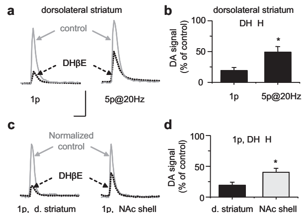
Fig. 6. Inhibition of \beta_2^* nAChRs with DH \beta E (0.1 \mu\text{M} ) altered DA signals. a, example DA signals evoked by 1p and by a 5p train given at 20 Hz within the dorsolateral striatum in the absence (control) or presence of DH \beta E. Scale bars, 0.5 \mu\text{M} DA and 0.5 s. b, the average DA signal evoked by 1p and 5p at 20 Hz in the presence of DH \beta H normalized to the control response as 100%. c, the DA signal evoked by 1p in the dorsolateral striatum and NAc shell in the absence (control) or presence of DH \beta E. The DA signals are normalized to 1p using different y-scale bars: 0.5 \mu\text{M} DA for the dorsolateral striatum, and 0.1 \mu\text{M} DA for the NAc shell and 0.5 s. d, the average DA signal evoked by 1p in the dorsolateral striatum and by the NAc shell in the presence of DH \beta H normalized to the control response as 100%.
