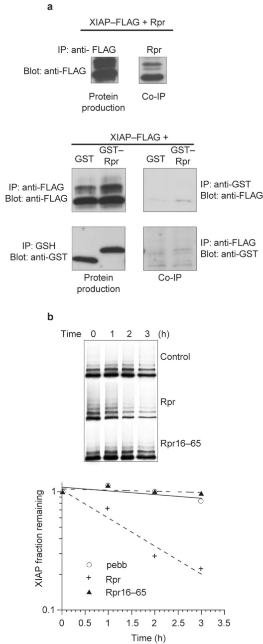
Figure 3. An unblocked Rpr N terminus is required for IAP binding and stabilization a , HEK 293T cells were transfected with Rpr, GST alone or GST—Rpr and FLAG-tagged XIAP protein. Proteins were precipitated with anti-FLAG or anti-Rpr antibodies and blotted with anti-FLAG. Proteins were precipitated with glutathione—Sepharose or anti-FLAG, and detected by immunoblotting with anti-GST or anti-FLAG. Although GST—Rpr and XIAP failed to coprecipitate, the untagged Rpr control clearly coprecipitated with XIAP protein. b , A pulse-chase experiment was performed as in Fig. 1c, using either wild-type Rpr (Rpr) or untagged Rpr lacking its first 15 amino acids (Rpr 16-65 ). The results were then quantified.
