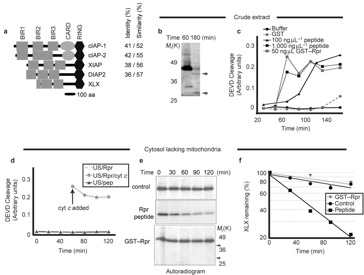
Figure 2. XLX, a X. laevis XIAP homologue, is destabilized by Rpr peptide, but not by GST-Rpr a , A domain map drawn to the scale of XLX with three human IAPs: cIAP1, cIAP2, and XIAP, and D. melanogaster DIAP2 is shown. Grey boxes represent BIR domains, ovals represent caspase recruitment domains (CARD), and hexagons represent C-terminal RING domains. The percentage identity and similarity between residues of each protein to XLX are indicated. BLAST alignment of XLX to proteins in the non-redundant public database yielded chicken and human XIAP as the most similar clones. XLX has a similar domain structure to XIAP and DIAP2. b , GST-Rpr and radiolabelled XLX were added to crude Xenopus egg extract. Samples were resolved by SDS-PAGE and autoradiography at the indicated times. Arrowheads denote the ~40K and 30K XLX cleavage products. Molecular weight markers are shown for reference with e below. c , GST-Rpr, GST, Rpr peptide or peptide vehicle were added to crude Xenopus egg extract. Caspase activity was monitored by cleavage of the colorimetric peptide substrate DEVD-pNA. d , GST-Rpr (Rpr) or Rpr peptide (Pep) were added to Xenopus egg extract depleted of mitochondria by centrifugation (US). At 60 min, human cytochrome c was added to an aliquot of the extract containing GST-Rpr (arrow). Caspase activity was monitored as in c above. e , Rpr peptide, peptide vehicle (control) or GST-Rpr were added together with radiolabelled XLX into Xenopus egg extract depleted of mitochondria. Samples were taken at the indicated times and XLX protein levels were analysed by SDS-PAGE and autoradiography. Molecular weight markers are shown for comparison with b and arrows indicate the approximate position of expected XLX cleavage fragments (which are absent). Equal loading was verified by Coomassie blue staining of gels (data not shown). f , The autoradiogram in e was quantified using a phosphorimager.
