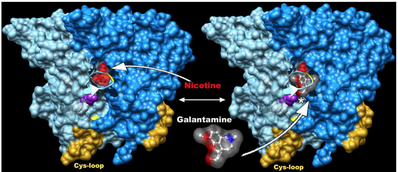
FIG. 7. Regulation of nAChRs by nontraditional ligands. In this illustration, an agonist-binding \alpha subunit (light blue) and a structural \beta subunit (dark blue) are shown with a solid surface looking from the extracellular side with either nicotine alone ( left ) or nicotine and galantamine ( right ). Photoaffinity labeling studies carried out using [ ^3\text{H} ]physostigmine and mapping of the epitope of the monoclonal antibody FK1 revealed that the region flanking the amino acid Lys-125 on the nAChR \alpha subunit contains essential elements of the physostigmine-binding site and is highly conserved among different \alpha subunits and across species (372,413,415). The galantamine-binding region is close to, but distinct from, the classical agonist-binding region. The galantamine-binding region is highly hydrophobic. As described in the text, elements that appear essential for binding of galantamine to the AChBP include the tryptophan residues 147 and 149, the tyrosine residue 93 or 55, and to a lesser extent the tyrosine residue 195. It has also been proposed that the dipole between the carbonyl group of the tryptophan residues and the protonated nitrogen of galantamine may be strengthened by the anionic side chain of the residue aspartate 89 (207). The crystallographic study of the AChBP-galantamine complex also revealed that some of the residues that contact galantamine in the complex are conserved among non- \alpha nAChR subunits, suggesting that galantamine may bind to both \alpha - and non- \alpha interfaces (207).
