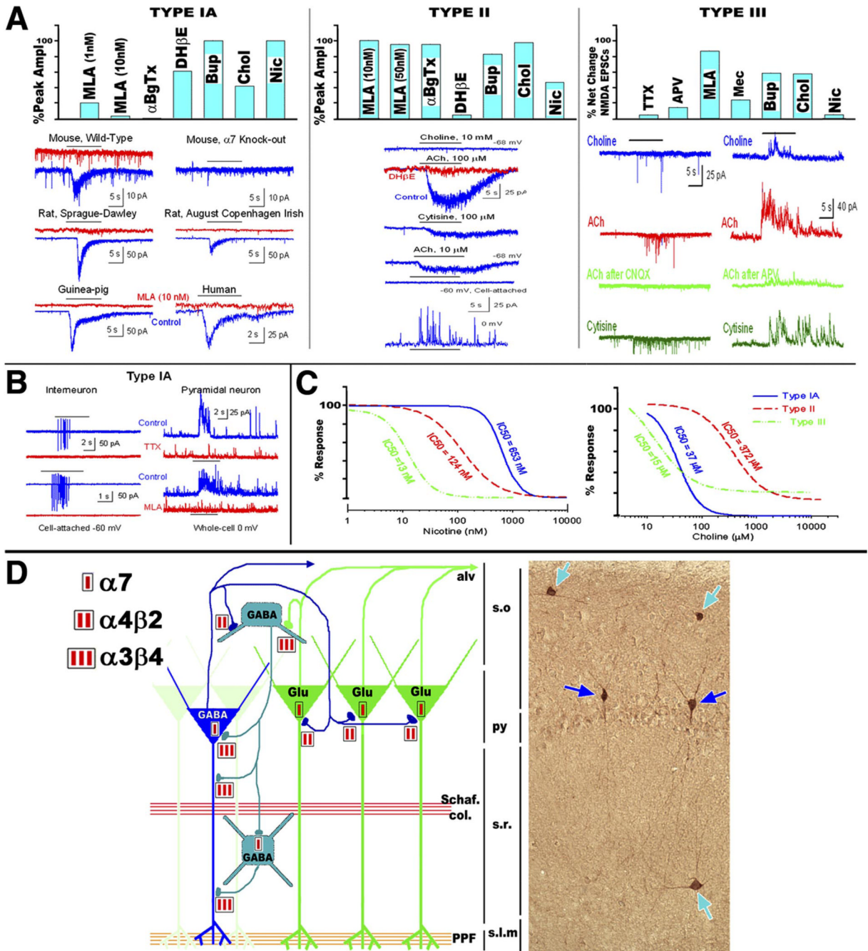
FIG. 4. Nicotinic receptor modulation of hippocampal inhibitory circuitry. A : choline (10 mM) induces type IA currents in hippocampal interneurons of different species of animals and in human cortical interneurons. Type IA current results from activation of \alpha 7 nAChRs because it is sensitive to blockade by nanomolar concentrations of methyllycaconitine (MLA) or \alpha -bungarotoxin ( \alpha -BGT). Type IA current is not blocked by bupropion (1 \mu M) or nicotine (100 nM), but is partially inhibited by DH \beta E (10 \mu M) or choline (50 \mu M). Nicotinic responses with these characteristics are not detected in neurons of mice with a null mutation in the gene that encodes the \alpha 7 nAChR subunit. In the presence of MLA (10 nM), ACh but not choline induces type II current in the interneurons. The poor efficacy of cytisine to induce type II current and
