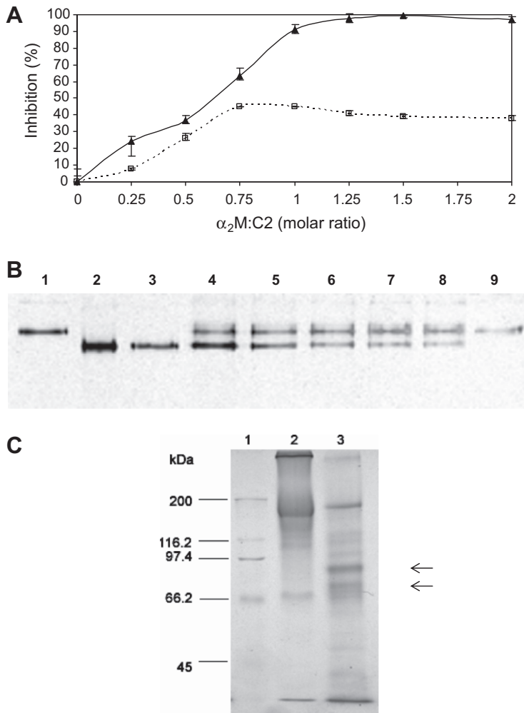
Figure 1. The interaction of the recombinant catalytic domain of congopain (C2) with bovine \alpha_2M . (A) The effect of increasing amounts of \alpha_2M on the activity of C2 against hide powder azure (▲) and Bz-Pro-Phe-Arg-pNA (□). Different concentrations of \alpha_2M were incubated with C2 (100 pmol for hide powder azure assay; 20 pmol for Bz-Pro-Phe-Arg-pNA assay) at molar ratios of 0.25:1, 0.5:1, 0.75:1, 1:1, 1.25:1, 1.5:1 and 2:1 for 20 min at 37 °C. Proteolytic activity was determined by the extent of hydrolysis of substrate compared to that of a C2 control with no \alpha_2M (100% activity), and expressed as a percentage inhibition. Error bars represent the \pm SEM ( n = 3 ). (B) Non-denaturing PAGE (5% gel) analysis of the interaction between bovine \alpha_2M and activated C2. Lanes 1 and 9 500 ng \alpha_2M ; lanes 2–8, \alpha_2M (500 ng) was incubated with increasing amounts of C2 (11–91 ng), corresponding to molar ratios of \alpha_2M:C2 of 0.25:1, 0.5:1, 0.75:1, 1:1, 1.25:1, 1.5:1 and 2:1 in the respective lanes. Proteins were silver stained. (C) Reducing SDS-PAGE (7.5% gel) after reaction of bovine \alpha_2M with activated C2. Lane 1, Bio-Rad molecular weight markers consisting of myosin (200 kDa), \beta -galactosidase (116.2 kDa), phosphorylase b (97.4 kDa), bovine serum albumin (66.2 kDa), and ovalbumin (45 kDa); lane 2, \alpha_2M (10 \mu g); lane 3, C2- \alpha_2M complex (10.372 \mu g). Proteins were stained with Coomassie blue R-250. Arrows represent bands at 95 and 85 kDa.
