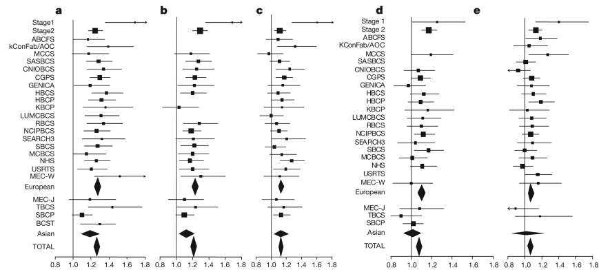
Figure 2. Forest plots of the per-allele odds ratios for each of the five SNPs reaching genome-wide significance a, rs2981582; b, rs3803662; c, rs889312; d, rs13281615; and e, rs3817198. The x-axis gives the per-allele odds ratio. Each row represents one study (see Supplementary Table 2), with summary odds ratios for all European and all Asian studies, and all studies combined. The area of the square for each study is proportional to the inverse of the variance of the estimate. Horizontal lines represent 95% confidence intervals. Diamonds represent the summary odds ratios, with 95% confidence intervals, based on the stage 3 studies only.
