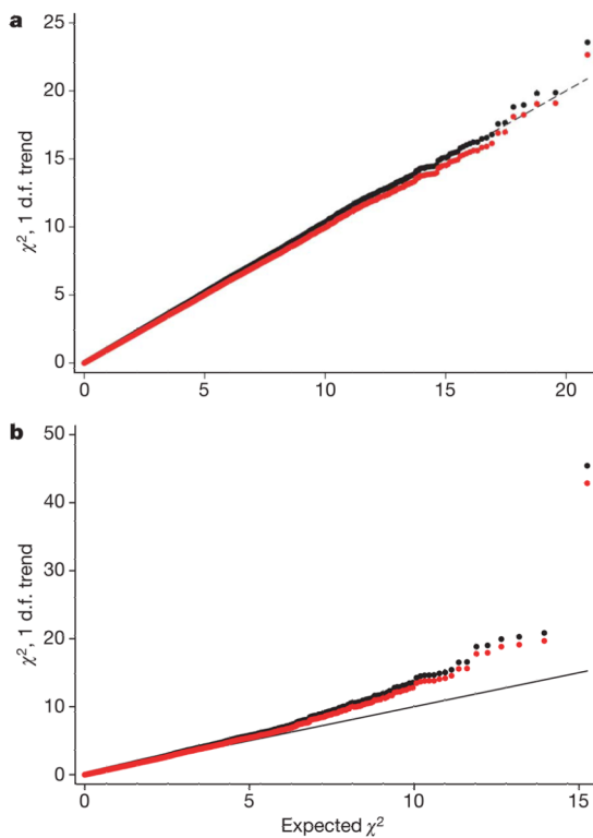
Figure 1. Quantile–quantile plots for the test statistics (Cochran-Armitage 1 d.f. \chi^2 trend tests) for stages 1 and 2 a. Stage 1; b. stage 2. Black dots are the uncorrected test statistics. Red dots are the statistics corrected by the genomic control method ( \lambda=1.03 for stage 1, \lambda=1.06 for stage 2). Under the null hypothesis of no association at any locus, the points would be expected to follow the black line.
