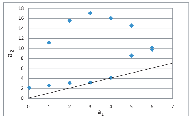
Figure 4 Confidence region based on the inversion of the likelihood ratio test for the Weibull two-changepoint model. The straight line is the 45-degree diagonal. Any points below the diagonal would imply that a second changepoint is located earlier than the first changepoint. No such points were within the confidence region. This figure shows the 95% confidence region for the two-changepoint model.
