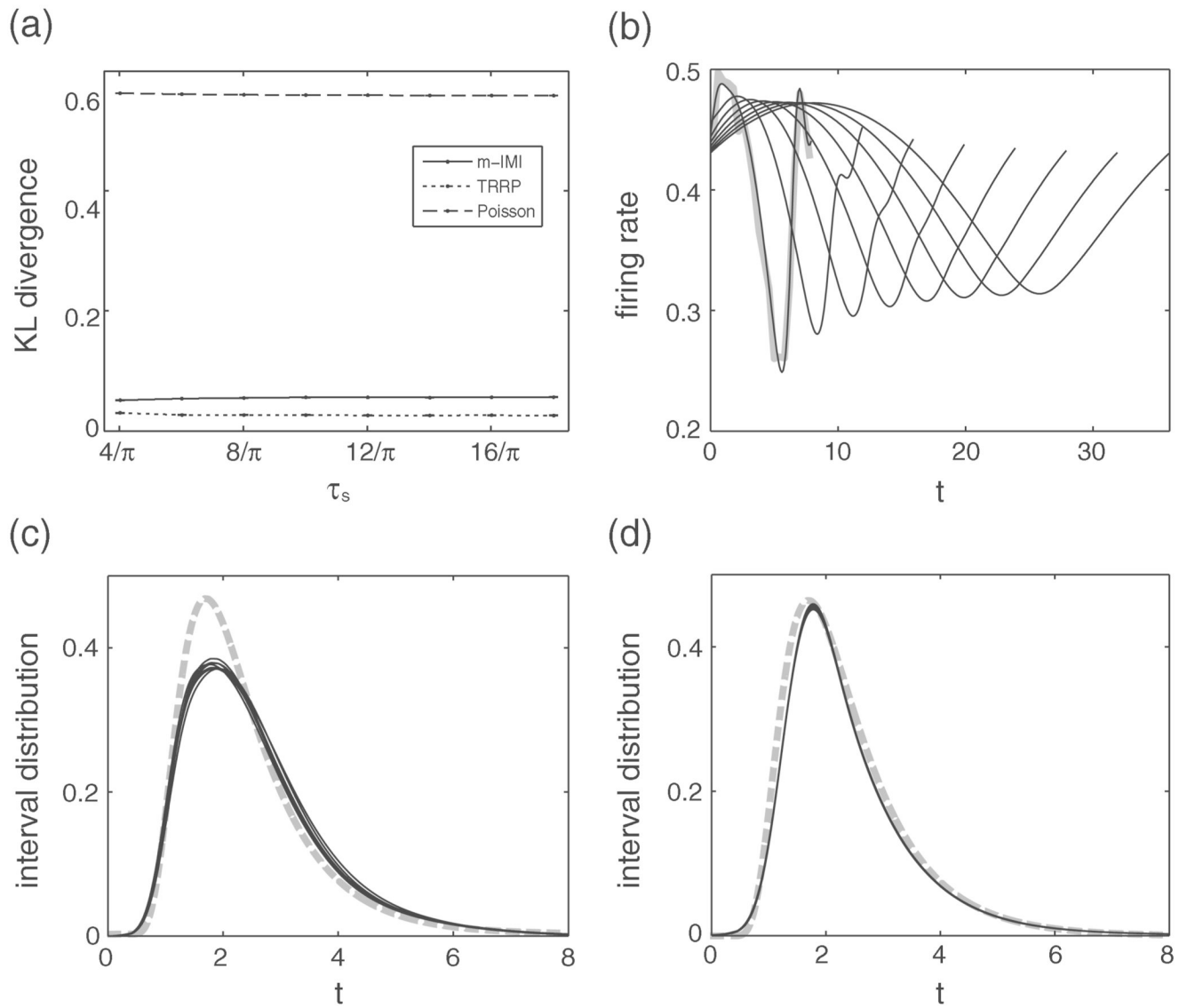
Figure 6. Results for the various values of the time constant of the time-varying variance of the input, \tau_s . (a–d) The same as Figure 5. Only the raw trace of the firing rate for \tau_s = 4/\pi is shown in b .
