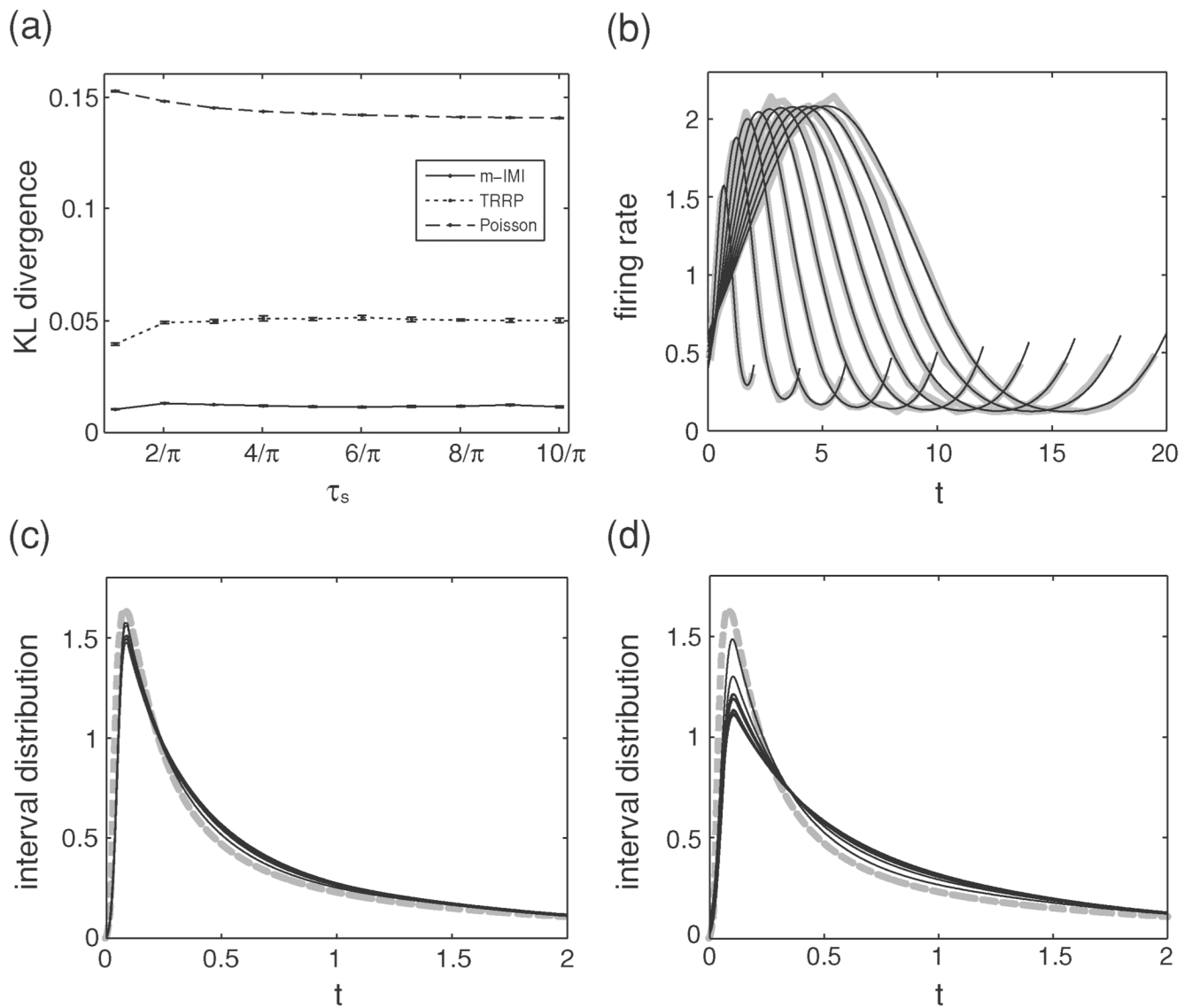
Figure 2. Results for various values of the time constant of the time-varying mean input, \tau_s . (a–d) The same as Figure 1.
