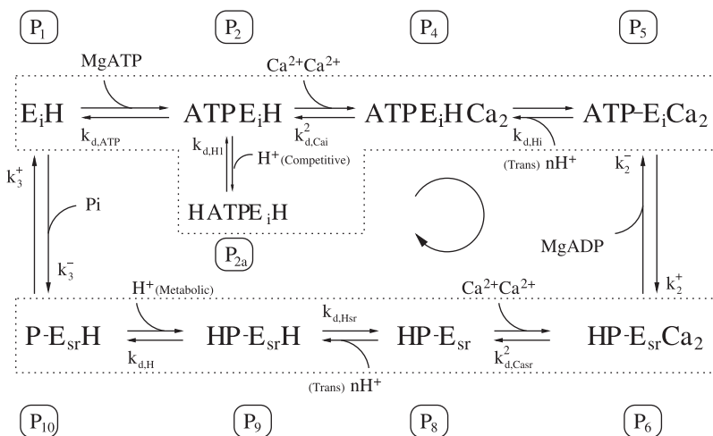
FIGURE 10 Application of the rapid equilibrium assumption to the ATP binding step reduces the forward and back binding constants (between states P1 and P2) to a single dissociation constant, K_{d,ATP} . The ATP binding step becomes lumped with the \text{Ca}^{2+} and \text{H}^+ binding steps as outlined by the top dotted box.
