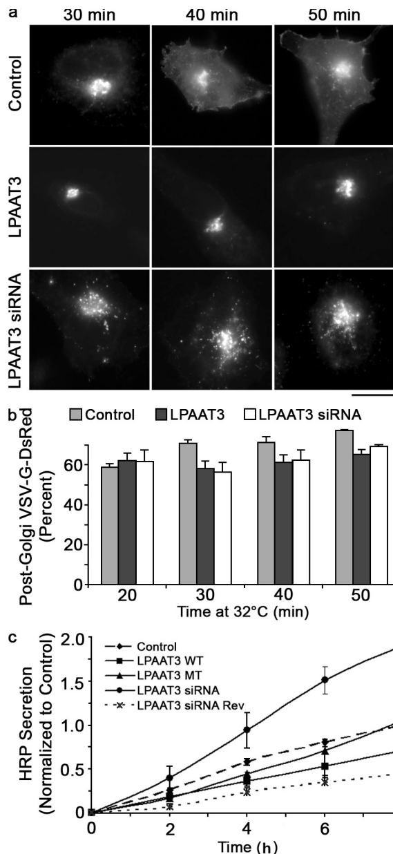
Figure 5. LPAAT3 and TGN trafficking. (a) Cells overexpressing LPAAT3 or knocked down for LPAAT3 were transfected with tsO45 VSV-G-DsRed and incubated at 40°C for 18 h, then released to 32°C for various time points. Bar = 20 \mu m. (b) The amount of tsO45 VSV-G-DsRed fluorescence in the Golgi complex was subtracted from the total fluorescence to determine the amount of post-Golgi transport of tsO45 VSV-G. Error bars represent SD for three independent experiments ( n = 100 ). (c) Cells were transfected with a secretable form of horseradish peroxidase (ssHRP). Media and lysates were tested every 2 h for HRP activity. Error bars represent three independent experiments.
