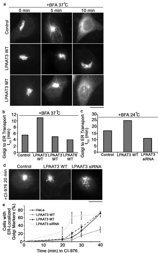
Figure 3. LPAAT3 overexpression slows BFA and CI-976-stimulated Golgi retrograde trafficking to the ER. (a) HeLa cells and cells transfected with LPAAT3 WT or LPAAT3 MT were treated with 10 \mu\text{g/ml} BFA and analyzed by immunofluorescence with GPP130 as a Golgi marker. Control cells, LPAAT3 MT cells, and LPAAT6 cells formed Golgi membrane tubules from 2 to 5 min after addition of BFA and were completely relocalized to ER membranes within 10 min, whereas LPAAT3 WT cells were slower. Bar = 20 \mu\text{m} . (b) The t_{1/2} of Golgi loss due to BFA tubulation was 5.5, 5.0, and 4.0 min for HeLa cells, LPAAT3 MT cells, and LPAAT6 cells, respectively, and 11 min for LPAAT3 WT cells. (c) To measure LPAAT3 knockdown cells treated with BFA, the experiment above was repeated at 24°C where the t_{1/2} values for cells was 18 min for control cells, 25 min for cells overexpressing LPAAT3 WT, and 11.2 min for LPAAT3 knockdown cells. Data are representative of three independent experiments. (d) Control cells, LPAAT3 WT cells, LPAAT3 MT cells, and LPAAT3 siRNA knockdown cells were treated with 50 \mu\text{M} of the LPAT inhibitor CI-976 for 30 min. Cells expressing LPAAT3 WT were slower at forming Golgi membrane tubules, whereas knockdown cells were considerably faster. Bar = 20 \mu\text{m} . (e) Quantification of the CI-976 results. All error bars are SD for three independent experiments ( n = 300 ).
