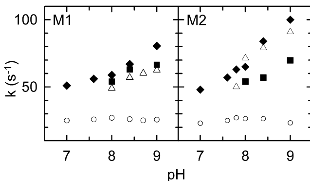
FIGURE 5 pH dependence of first-order rate constants of manganese oxidation in the M1 ( left panel ) and M2 ( right panel ) mutants. The rate constants were determined by the exponential decomposition of the kinetics recorded in the presence of 100 \mu\text{M} \text{Mn}^{2+} and in the absence of any anion ( open triangles ), in the presence of 15 \text{ mM} bicarbonate ( solid diamonds ), and in the presence of 100 \text{ mM} acetate ( solid squares ). The rate constants for P^+Q_A^- \rightarrow PQ_A ( open circles ) are also shown. Conditions as in Fig. 2.
