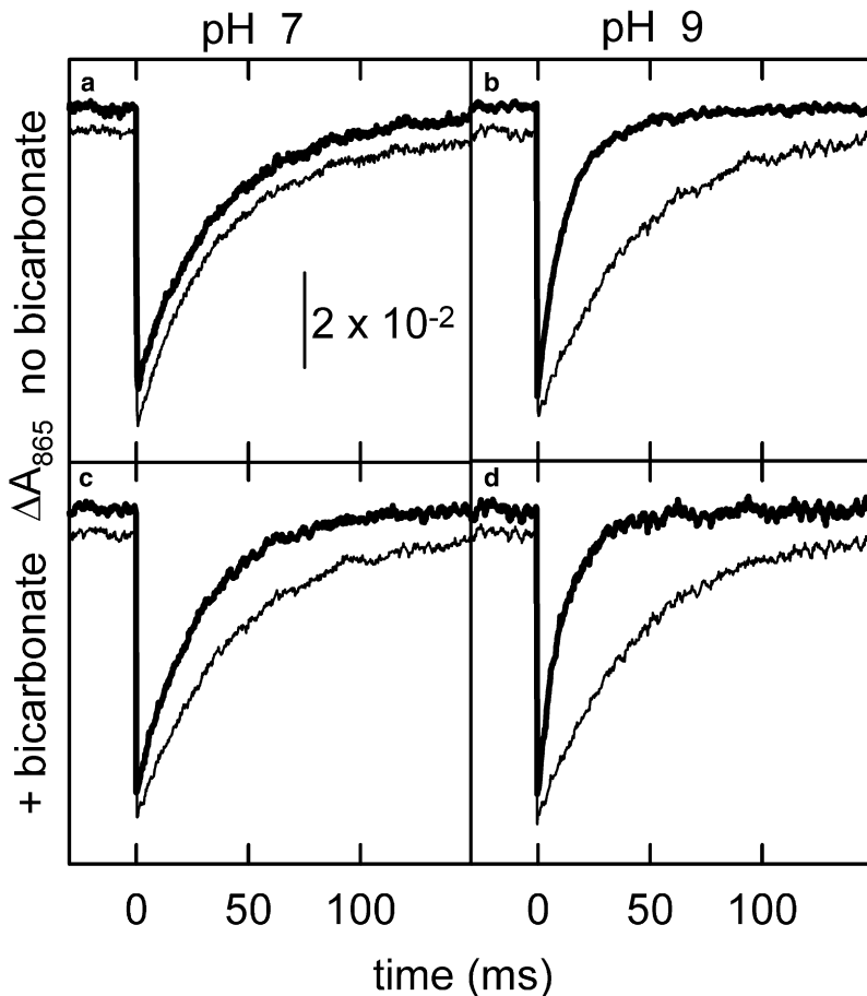
FIGURE 4 Kinetic traces of P^+ reduction in the presence of 100 \mu\text{M} terbutryne monitored at 865 \text{ nm} in the M2 mutant after a saturating laser flash excitation at pH 7 ( a and c ) and at pH 9 ( b and d ) in the absence ( a and b ) and in the presence ( c and d ) of 15 \text{ mM} bicarbonate, respectively. The kinetics were recorded after a saturating laser flash. The traces with thin lines were recorded without any added manganese and could be fitted with single exponentials representing the kinetics of P^+Q_A^- \rightarrow PQ_A charge recombination with rate constants of 23\text{--}24 \text{ s}^{-1} . The traces with thick lines, which are vertically shifted for better comparison, were recorded in the presence of 100 \mu\text{M} \text{Mn}^{2+} ions, and, except in panel a , the P^+ decay could be resolved into two kinetic components. The faster component was assigned to the P^+ reduction by \text{Mn}^{2+} and the slower to the P^+Q_A^- \rightarrow PQ_A charge recombination. The kinetic analysis resulted in the following rate constants and the relative amplitudes: 24 \text{ s}^{-1} (100%) for panel a ; 23 \text{ s}^{-1} (13%) and 91 \text{ s}^{-1} (87%) for panel b ; 24 \text{ s}^{-1} (38%) and 48 \text{ s}^{-1} (62%) for panel c ; and 23 \text{ s}^{-1} (8%) and 100 \text{ s}^{-1} (92%) for panel d . Conditions as in Fig. 1.
