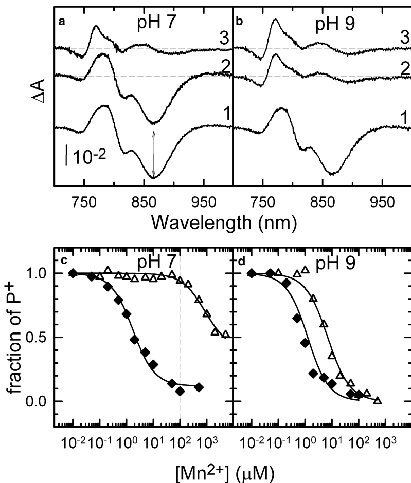
FIGURE 1 (a and b) Light-minus-dark difference optical spectra of the M1 mutant at pH 7 and pH 9 in the absence of either manganese or bicarbonate ions (trace 1), in the presence of 100 \mu M manganese (trace 2), and in the presence of both 100 \mu M manganese and 15 mM bicarbonate ions (trace 3). (c and d) Fraction of P + as a function of the added Mn 2+ concentration measured in the M1 mutant at pH 7 and pH 9 in the absence (open triangles) and in the presence of 15 mM bicarbonate (solid diamonds). The data points were taken from the light-minus-dark difference spectra recorded at various manganese concentrations as the absorbance changes at 865 nm as indicated, with the double-headed vertical arrow on panel a. The solid lines are the best fits to the data points using Eq. S2 with the following dissociation constants: 853 \mu M and 1.5 \mu M at pH 7, and 6.2 \mu M and 1.0 \mu M at pH 9 in the absence and in the presence of 15 mM bicarbonate, respectively. The vertical dashed lines in panels c and d drawn at 100 \mu M manganese concentration indicate the condition at which the spectra on panels a and b were recorded. Conditions: 1.5 \mu M BRC in 0.03 Triton X-100, 100 \mu M tertbutryne, 15 mM HEPES (pH 7), or Ches (pH 9).
