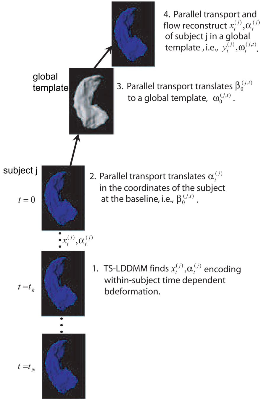
FIG. 1. A schematic for studying time dependent shape changes.
