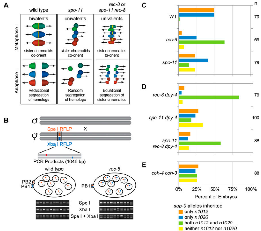
Figure 2. Sister chromatids separate equationally during meiosis I of rec-8 and spo-11 rec-8 mutants, while homologs segregate randomly in spo-11 mutants. (A) Model of meiotic chromosome segregation in wild-type, spo-11 , and rec-8 mutant worms as shown by RFLP analysis in B. Three chromosomes are shown (green, blue, and red); homologs are indicated by different shades of the same color. The Aurora B kinase AIR-2, thought to mark REC-8 for destruction, is depicted in yellow. Arrows indicate the direction of MT-dependent forces exerted on chromosomes. In wild-type zygotes, sister chromatids co-orient. AIR-2 accumulates between homologs, which separate during meiosis I. Sister chromatids also co-orient in spo-11 mutants, SCC is protected during meiosis I, and sisters remain together while homologs segregate randomly in meiosis I. spo-11 zygotes inherit zero, one, or two copies of each chromosome, resulting in aneuploidy. In rec-8 mutants, sister chromatids biorient. AIR-2 localizes between sisters, which separate equationally when SCC is removed prematurely during anaphase I. Zygotes inherit a chromatid from each homolog. Because extrusion of the second polar body fails (Fig. 3), fertilization by a wild-type sperm would produce a viable triploid. (B) Strategy for examining meiotic chromosome segregation with ChrII-RFLPs. This assay, together with knowledge of the number of polar bodies extruded (Fig. 3) and whether or not sister chromatids remain together in prophase II (Fig. 1G), allows unambiguous determination of the pattern of chromosome segregation in meiosis I and II, as explained in Supplemental Table S2. Trans -heterozygous mothers [genotype sup-9(n1012)/sup-9(n1020) ] are mated with wild-type males. n1012 and n1020 introduce a SpeI RFLP and an XbaI RFLP, respectively (de la Cruz et al. 2003). The lesions are amplified in a single PCR product. The cross progeny of an n1012/n1020 hermaphrodite and a wild-type male inherit a single sup-9 allele from their mother and a wild-type copy from their father. The progeny of n1012/n1020, rec-8 mutant worms mated with wild-type males inherit both ChrII-RFLPs and the wild-type sup-9 allele. ChrII-RFLPs are revealed by a doublet in SpeI or XbaI digests. An uncut product in SpeI/XbaI double digests reveals the wild-type allele. The alleles partitioned into polar bodies are not detected. (C) During wild-type meiosis, zygotes inherit a single ChrII-RFLP. In contrast, most rec-8 mutant embryos inherit both ChrII-RFLPs. The four possible outcomes of meiosis (inheritance of an n1012 allele, an n1020 allele, both alleles, or neither allele) occur at similar levels in spo-11 embryos. (D) Most progeny of spo-11 rec-8 mutants inherit both ChrII-RFLPs. The dpy-4 mutation was used in the construction of the spo-11 rec-8 double mutant. (E) Chromosome segregation in coh-4(tm1857) coh-3(gk112) embryos resembles that of spo-11 mutants.
