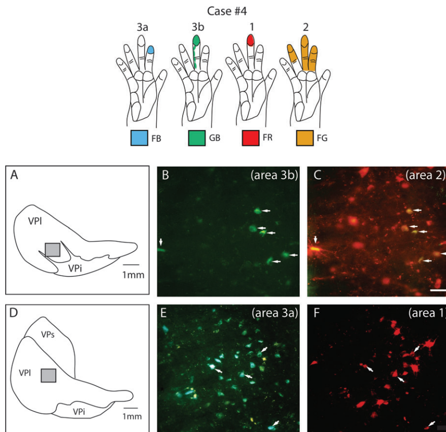
Figure 11. Photomicrographs of coronally sectioned portions of the dorsal thalamus that contain double-labeled cells (B, C, E, and F) resulting from injections into electrophysiologically defined locations in areas 3a, 3b, 1, and 2 in case no. 4. The illustration at the top depicts the receptive field locations for neurons at the center of each injection site. In this figure only, the color of the receptive field corresponds to the color of the fluorescing labeled cell bodies, rather than to the area injected. The precise location of these cells in VPI is illustrated in (A) and (D) (shaded box). Double-labeled cells (white arrows in B and C) were observed in VPI following injections of fluorescent GB in area 3b and FG in area 2. Double-labeled cells were also observed in VPI following injections of FB in area 3a and FR in area 1. These photographs were taken from sections intervening between those reconstructed in Figures 9 and 10 from this same case. Scale bar for photographs = 100 µm. See Table 1 for abbreviations. Conventions as in previous figures.
