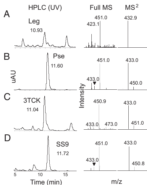
Fig. 4. Targeted chemical validation of Photobacterium profundum NAB pathways. LCMS analysis of NuO sugars isolated from purified LPS of Leg (A) or Pse (B) or from cultures of P. profundum genome strain (C) 3TCK or SS9 (D). Different HPLC retention times enable differentiation between Leg and Pse and reliable identification of NuO in 3TCK and SS9. MS and MS 2 analyses provide additional confirmation of the expected mass for Leg and Pse for both standards and unknowns. In all cases, MS data are shown from 400–500 m/z .
