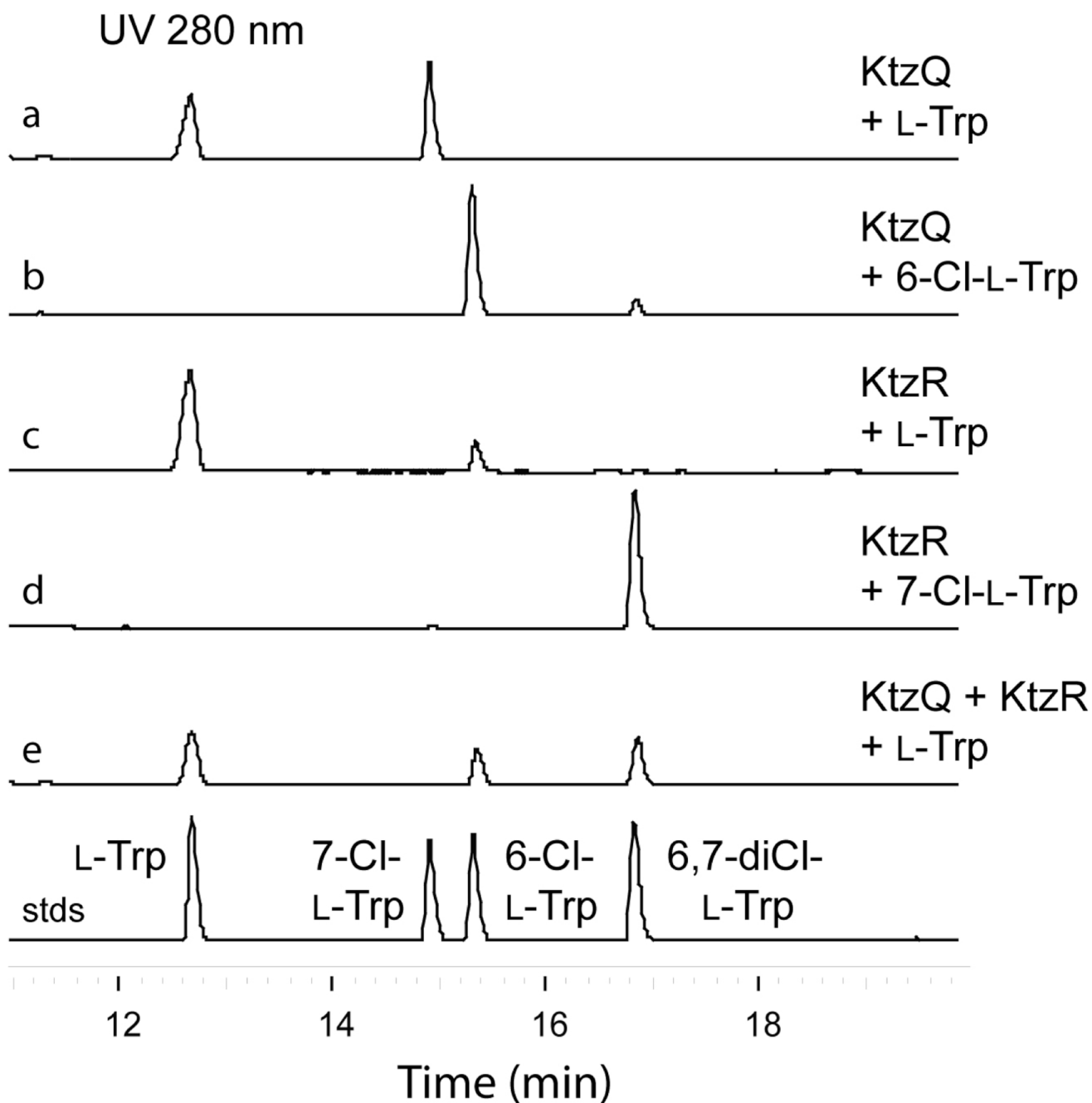
Figure 2. HPLC analysis of the KtzQ and KtzR catalyzed halogenations. (a) KtzQ incubated with L-Trp (b) KtzQ incubated with 6-Cl-L-Trp (c) KtzR incubated with L-Trp (d) KtzR incubated with 7-Cl-L-Trp (e) KtzQ and KtzR incubated with L-Trp
