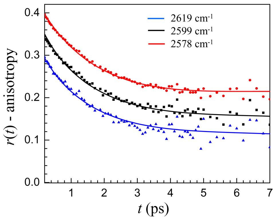
Figure 6. Anisotropy decays and two component model fits for the w_0 = 25 AOT reverse micelle. Three frequencies in the interfacial region are shown. Red circles = 2578 \text{cm}^{-1} . Black squares = 2599 \text{cm}^{-1} . Blue triangles = 2619 \text{cm}^{-1} . The top and bottom data and fits are offset up and down by 0.05 so that the fits can be seen clearly.
