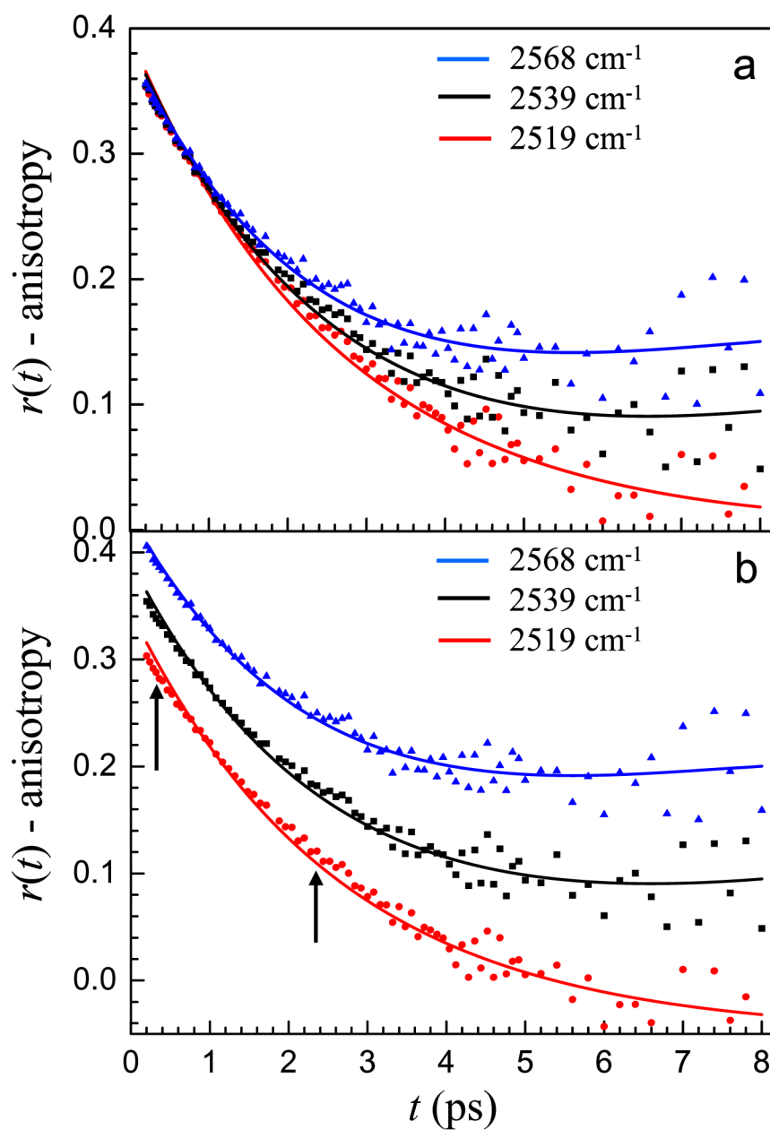
Figure 7. Anisotropy decays and two component model fits for the w_0 = 46 reverse micelle at frequencies outside of the interfacial spectral region. Red circles = 2519 \text{ cm}^{-1} . Black squares = 2539 \text{ cm}^{-1} . Blue triangles = 2568 \text{ cm}^{-1} . a. Unshifted data and fits to clearly show how the decay slows as the frequency increases. b. The top and bottom data and fits are offset up and down by 0.05 so that the results can be seen clearly. The fit is quite good at 2568 \text{ cm}^{-1} but begins to miss at early and intermediate times at lower frequencies as marked by the arrows.
