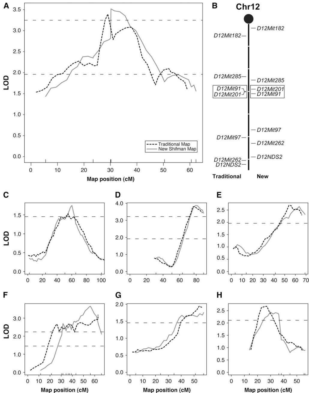
FIGURE 4.—QTL With changes in peak shape. Seven QTL were found where the peak shape was altered due to subtle differences between the original and the revised Shifman maps. (A) The QTL for femoral BMD on chromosome 12 in the NZBxRF cross appears as a double peak when analyzed using the Mouse Genome Database (MGD)/traditional genetic map (dashed line), suggesting the presence of two closely linked QTL. When reanalyzed using the new genetic map, this double peak is collapsed into a single peak (solid line). (B) This double peak is the result of two flipped neighboring markers. Seven markers were typed in this cross for chromosome 12. The markers are placed on the centimorgan scale (center line) in relation to the MGD/traditional map (left) and the new genetic map (right). Note the difference in spacing of the markers when comparing the two maps. The other QTL with a change in peak shape were found for: (C) B6xCAST on chromosome 2, (D) B6xC3H on chromosome 2 for vBMD, (E) NZBxRF on chromosome 4 for vBMD, (F) B6xCAST on chromosome 14, (G) B6xCAST on chromosome 18, and (H) NZBxSM on chromosome 19.
