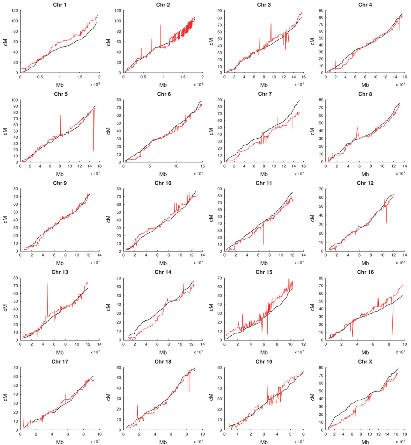
FIGURE 3.—Physical and genetic positions of markers. Genetic marker positions (in centimorgans) are plotted against their physical positions (in megabases) for the MGI genetic map (red) and the revised Shifman map (black). Marker-ordering errors in the MGI map are indicated by non-monotone fluctuations. In contrast, the curves for the revised map are smooth and monotone.
