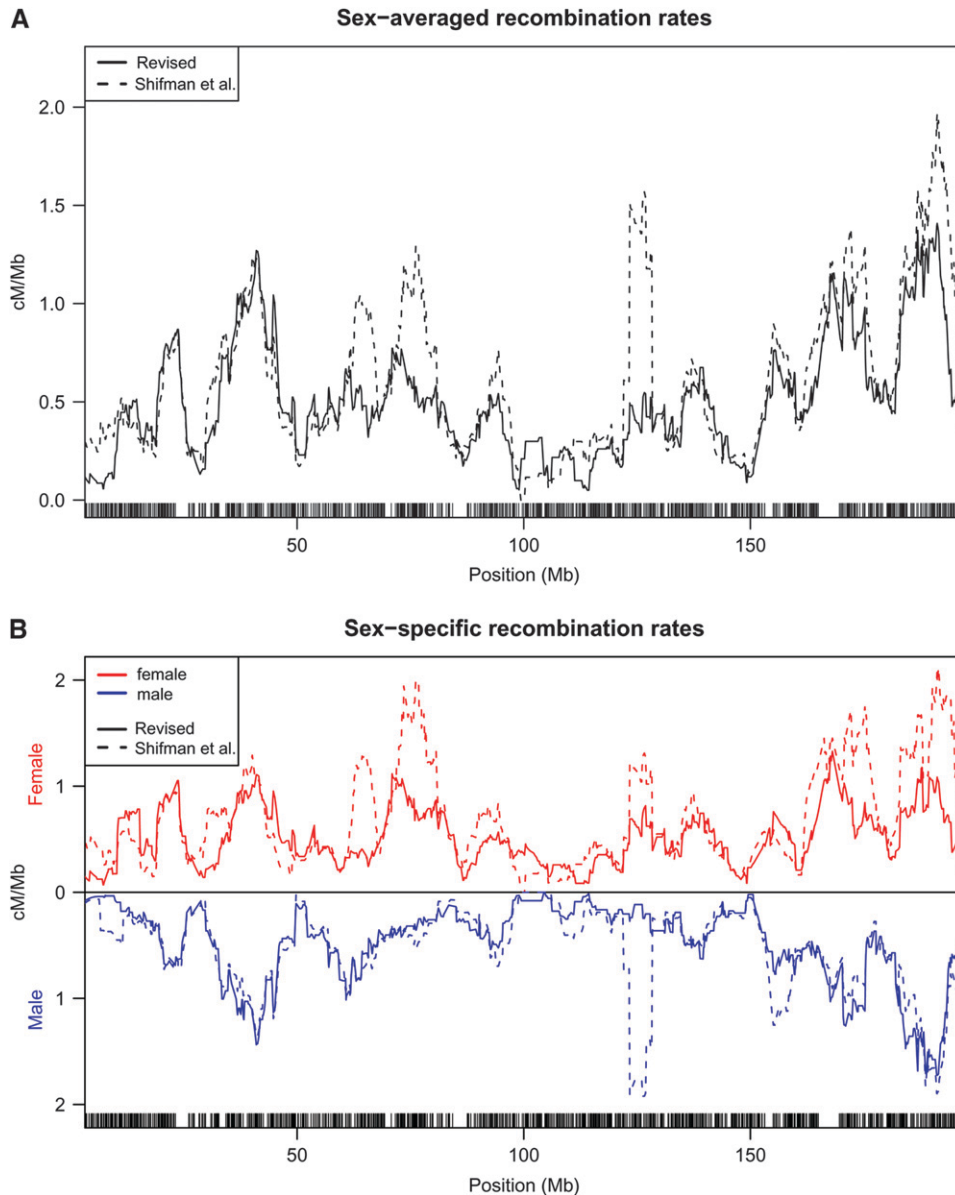
FIGURE 1.—Comparison of the original and revised genetics maps. Sex-averaged recombination rates (A) and sex-specific recombination rates (B) for the original and revised genetic maps of chromosome 1. Maps are based on data from SHIFMAN et al. (2006) as described in MATERIALS AND METHODS. Figures showing all chromosomes can be found in Figure S1.
