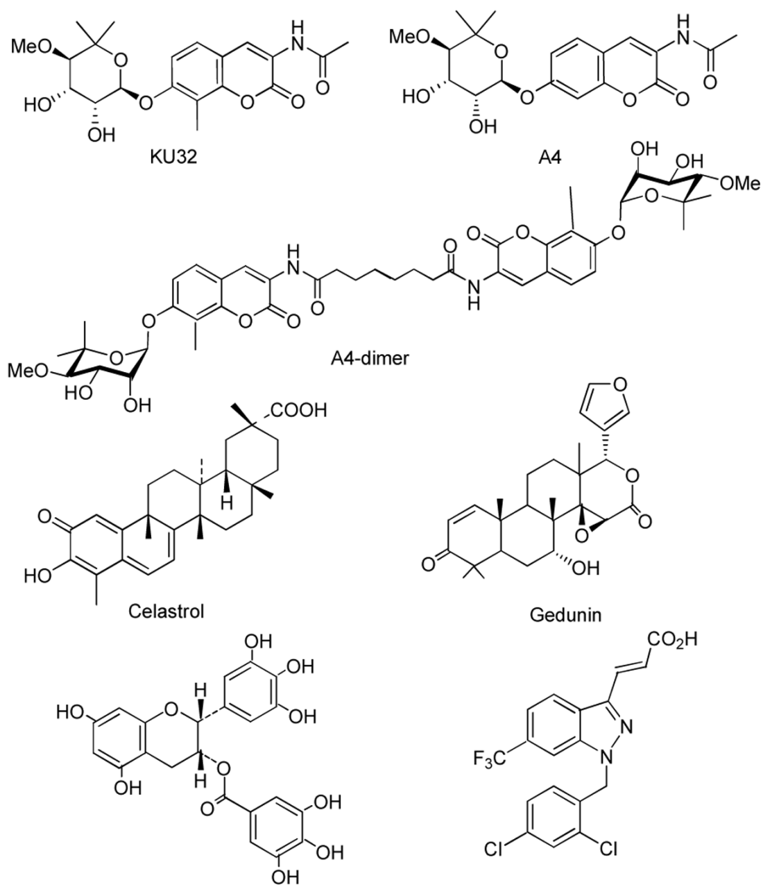
Figure 2. Structure of novobiocin analogues A4, A4-dimer, KU32 and other Hsp90 inhibitor
