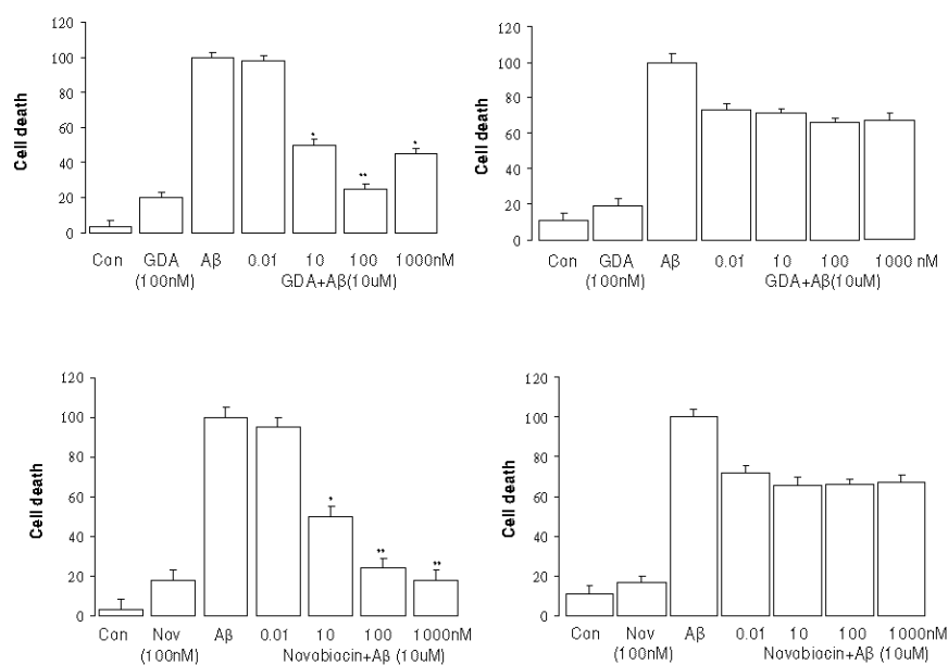
Figure 4. Dose dependent GDA and novobiocin protection against A \beta_{25-35} toxicity. (Left, without retinoic acid; Right, with retinoic acid). * p<0.05 and ** p<0.01 vs A \beta Control
