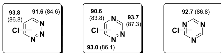
Figure 9. C-Cl BDEs of 6-membered heterocycles using G3B3 (bold) and B3LYP (parentheses); energies in kcal/mol.
