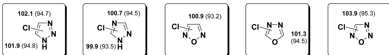
Figure 7. C-Cl BDEs of 5-membered heterocycles with 3 or 4 heteroatoms using G3B3 (bold) and B3LYP (in parentheses), in kcal/mol.
