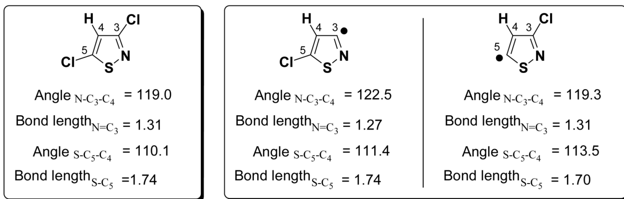
Figure 6. Bond angle and bond length analysis of G3B3 calculated structures of chloroisothiophene and its radicals.
