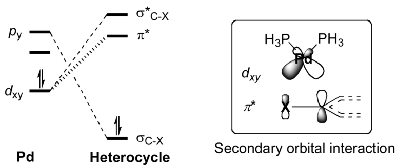
Figure 1. FMO interactions between PdLL' and Ar-X in an oxidative addition.
