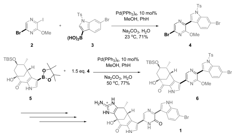
Scheme 1. Regioselective cross-coupling reactions in the total synthesis of (+)-Drugmacidin F.
