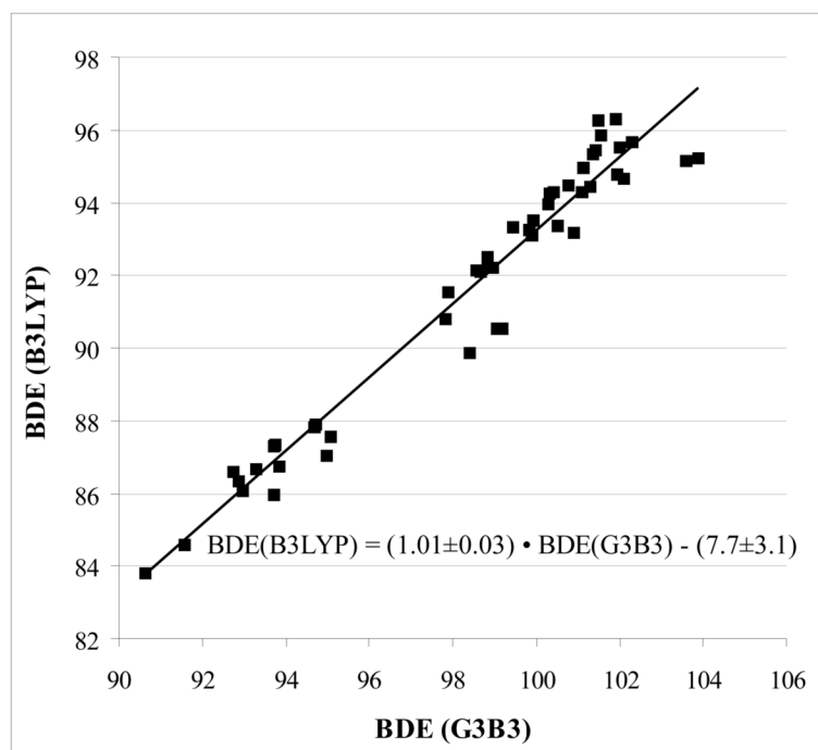
Figure 2. Comparison of BDEs computed using UB3LYP/6-31G(d) and G3B3 (kcal/mol). The correlation coefficient is R^2 = 0.975 \pm 0.007 .
