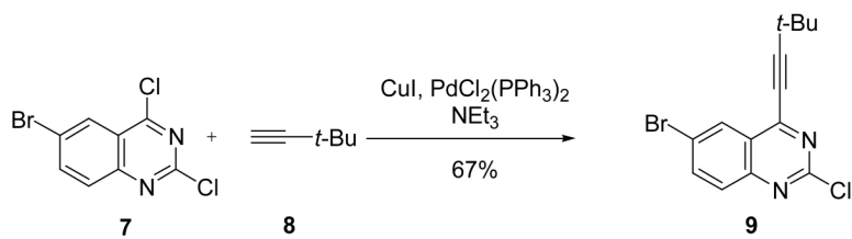
Scheme 2. Sonogashira cross-coupling reaction of 6-bromo 2,4-dichloroquinazoline 7 .
