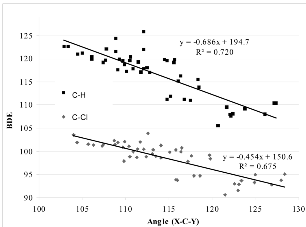
Figure 12. Bond angle vs. C-Cl BDE of chloro heterocycles and C-H BDE of heterocycles using G3B3. (Results for C-H BDEs from Feng et al. 18 )
