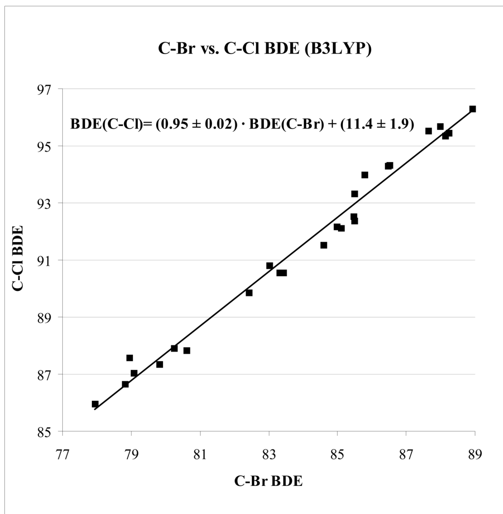
Figure 3. Comparison of C-Cl and C-Br BDEs using UB3LYP/6-31G(d); BDEs in kcal/mol. The correlation coefficient is R^2 = 0.992 \pm 0.002 .
