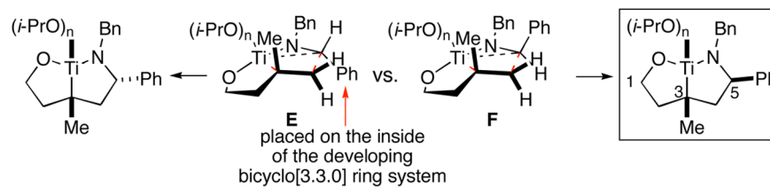
Figure 3. A model for stereoselection in imine–alkene cross coupling. 7, 8
