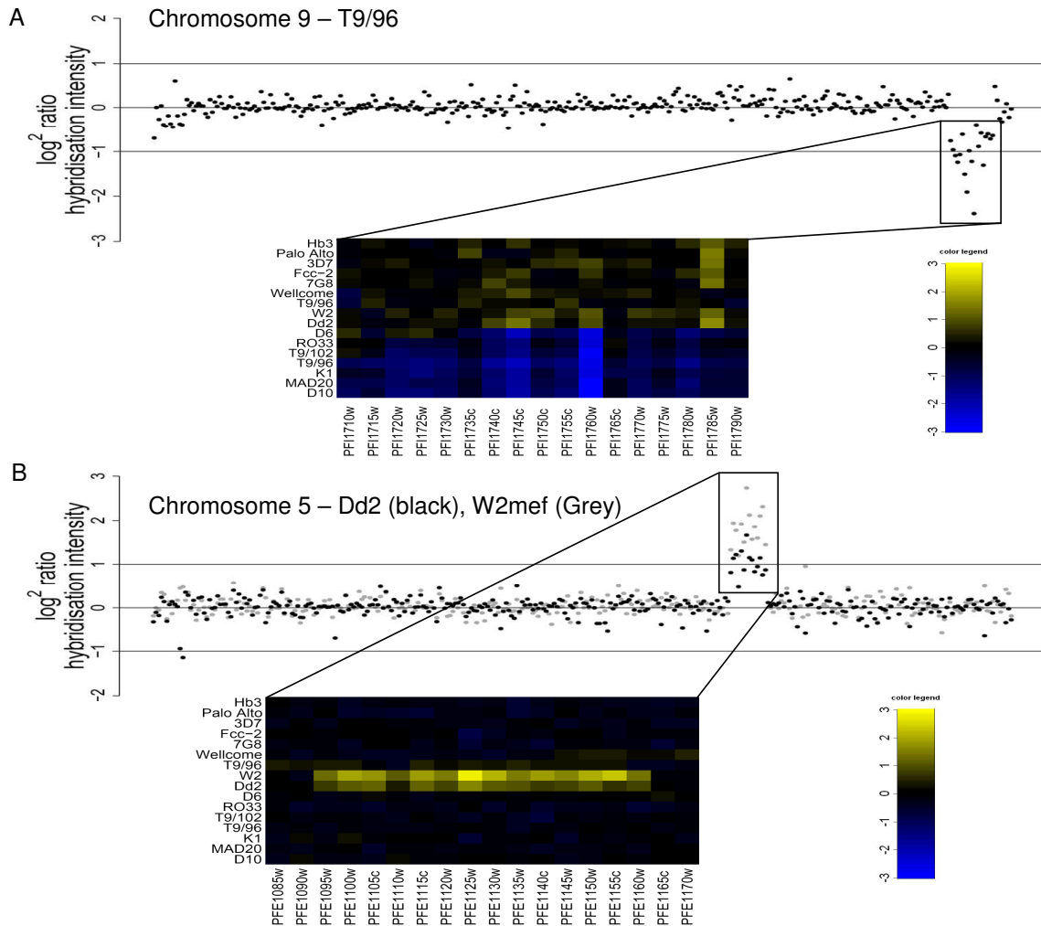
Figure 2 CNV regions in the P. falciparum genome. Detection of previously described multi-genic deletions and amplifications. Plots show \log_2 hybridisation signal of individual genes in physical order along chromosomal length with cut-offs for amplification/deletion of a gene shown by lines at \pm 1 respectively. Heatmaps show CNV regions at greater resolution for all hybridised strains with genes amplified or deleted as indicated by the colour key (yellow and blue respectively). A. Multi-genic deletion on chromosome 9. B. Multi-genic amplification on chromosome 5.
