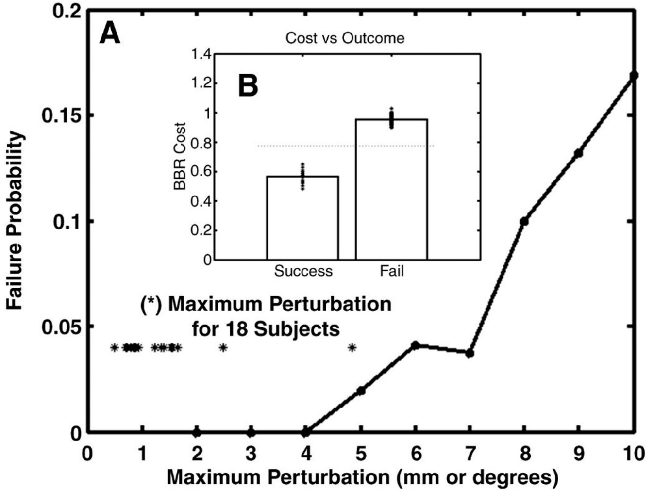
Figure 4. Robustness of BBR to random changes in initial position. Failure is defined as an inability to return to the original solution to within 0.100mm AAD. Panel A shows the probability of a failure as a function of maximum perturbation. The asterisks show the maximum perturbation for 18 subjects between their first fMRI run and their eighth within a scanning session. Panel B shows the value of the cost function for successes and failures (asterisks are individual data points) and demonstrates that the failures can be detected by a simple threshold.
