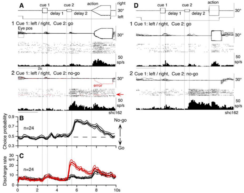
Fig. 6. No-go neurons. A and D, representative neuron during smooth pursuit (A) and saccade tasks (D). A1, go trials when cue 1 was rightward and leftward visual motions. A2, no-go trials. Red traces (arrows) highlight an error trial. B, CP time course for 24 no-go neurons during no-go and go- trials. C, time course of mean ( \pm SE) discharge of the 24 neurons during no-go (red) and go-(black) trials. D1 and D2, go trials and no-go trials for saccades, respectively.
