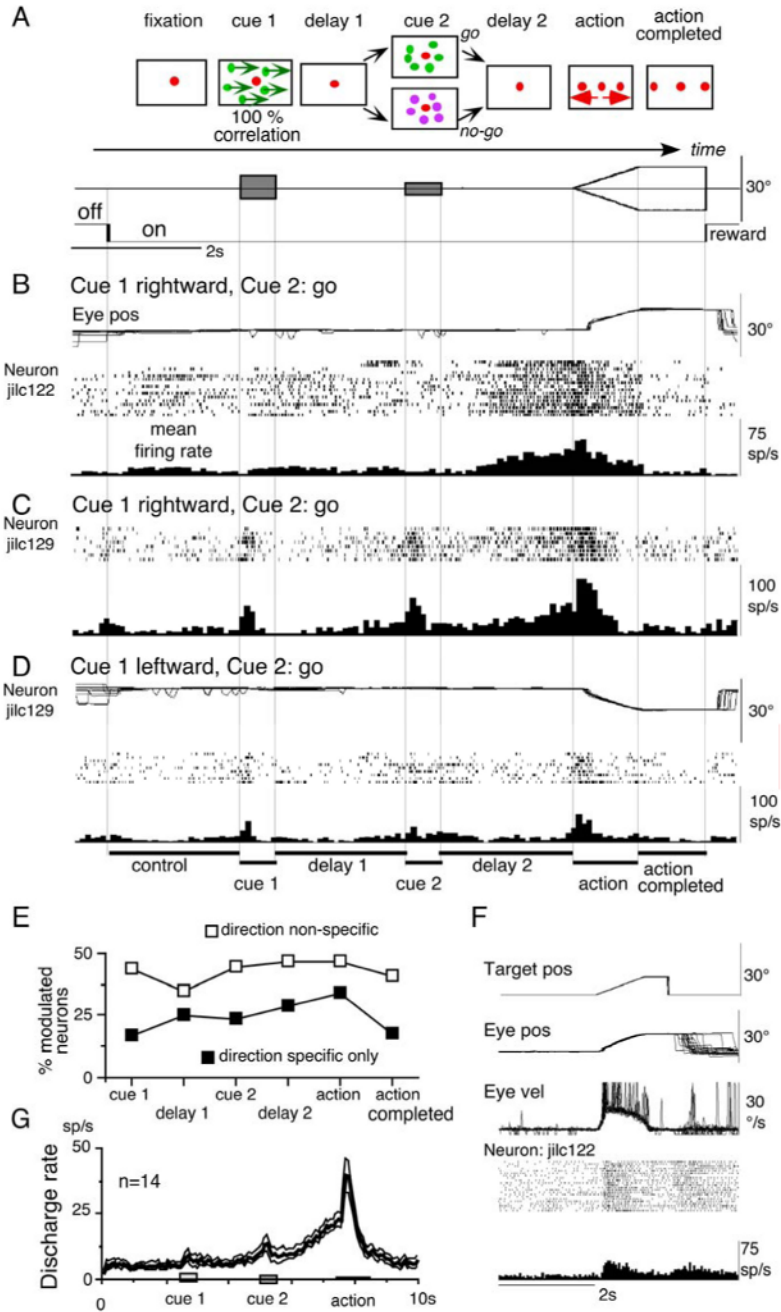
Fig. 1. Task conditions and discharge of SEF neurons. A, task conditions. B-D, spike rasters and averaged histograms of 2 SEF neurons during go trials as indicated. Top traces in B and D are superimposed eye position (eye pos). E, percentage of modulated neurons that preferred go trials during different task periods. F, discharge of the same neuron shown in B during a simple ramp-tracking task of a single spot. Saccade velocities (eye vel) are clipped. G, mean ( \pm SE) discharge of movement preparation neurons. See text.
