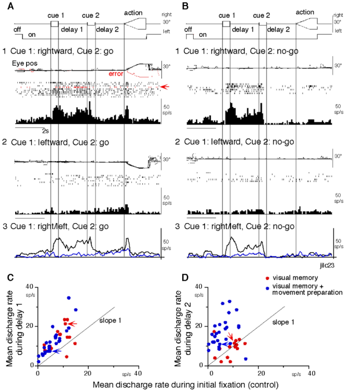
Fig. 2. Discharge of representative visual memory neuron and comparison with visual memory + movement preparation neurons during delay periods. A1-2, rightward (A1) and leftward (A2) visual motion go trials. B1-2, rightward (B1) and leftward (B2) no-go trials. Red traces pos and spike raster in A1 highlight an error trial. A3 -B3 compare mean discharge rightward (black) / leftward (blue) for cue 1 visual motion go- no-go trials, respectively. C, mean discharge of visual memory neurons (red) and visual memory + movement preparation neurons (blue) during delay 1 against initial fixation. D, mean discharge of visual memory neurons (red) and visual memory + movement preparation neurons (blue) during delay 2 against initial
