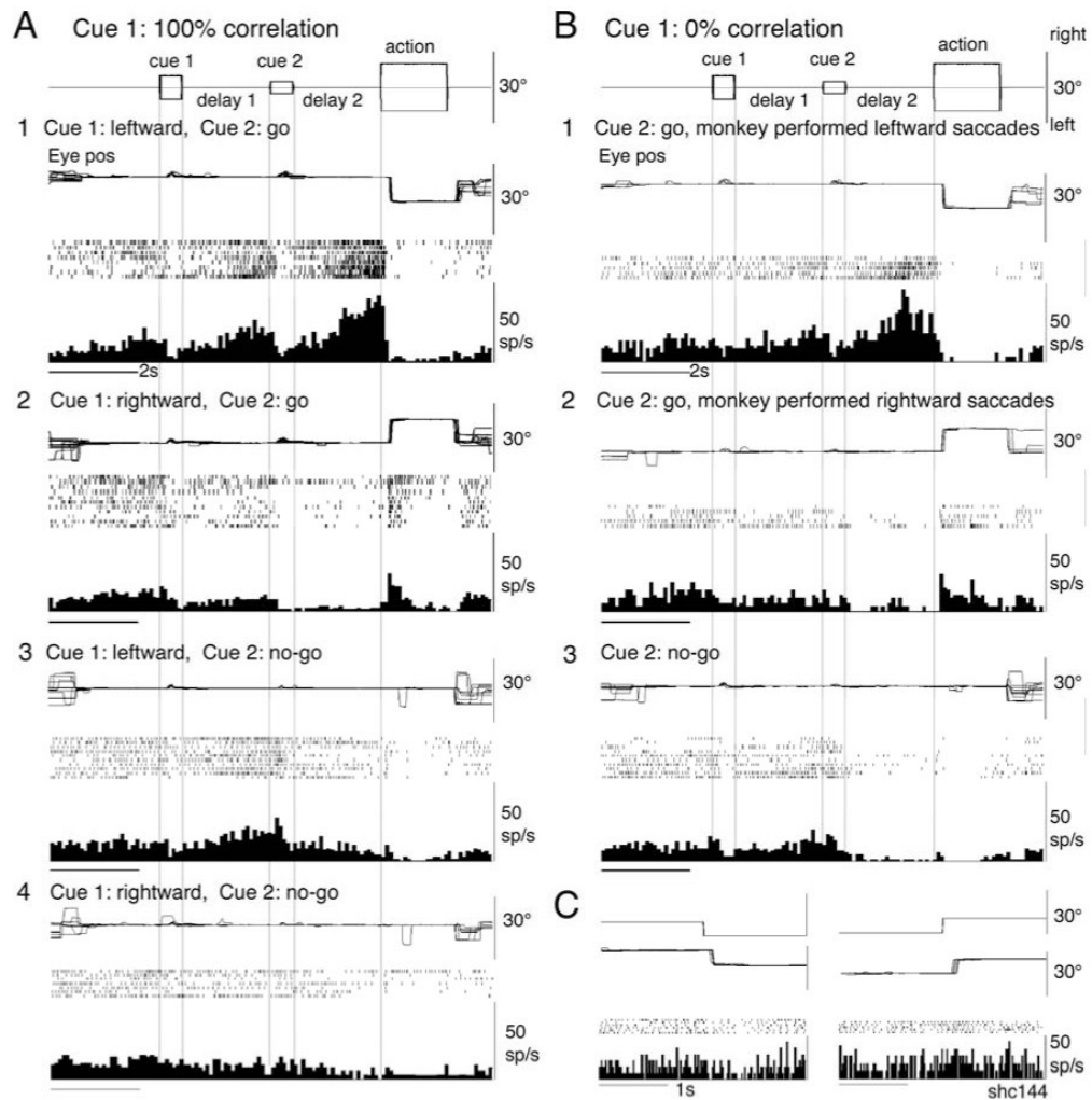
Fig. 5. Discharge of representative visual memory + movement preparation neuron during saccade task. A and B, cue 1 was 100 % and 0 % correlation, respectively. A1 and 2, go trials for saccades when cue 1 was leftward (A1) and rightward (A2) visual motion (100 % correlation). A3 and A4, no-go trials as indicated. B1 and B2, go trials for saccades, cue 1 was 0 % correlation. Traces were grouped into leftward saccades (B1) and rightward saccades (B2). B3, no-go trials. C, discharge during a visually guided saccade task with a single spot.
