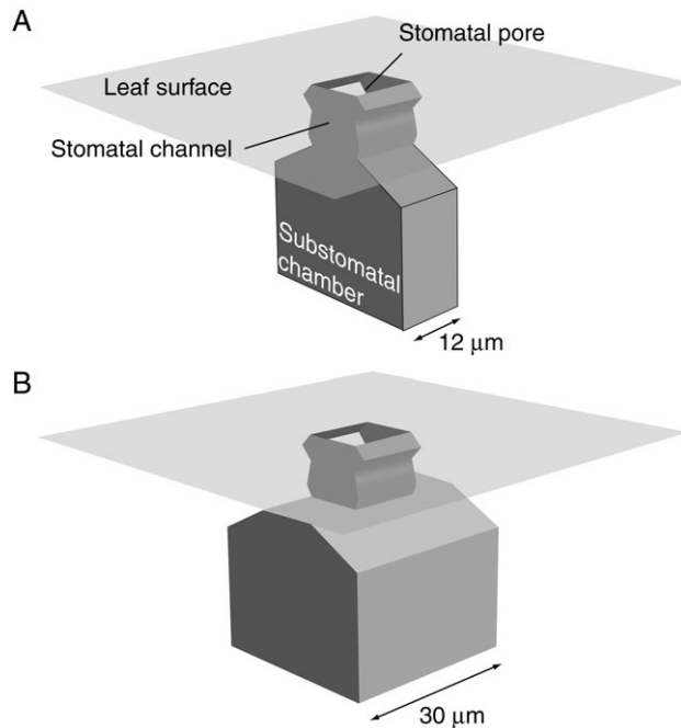
FIG. 1. Basic geometry of the three-dimensional model with a smaller (A) and a larger (B) substomatal chamber. It includes a stomatal porus which is connected to the chamber by a stomatal channel. The model also comprises an air layer adjacent to the leaf surface which has a thickness of 35 \mu\text{m} . The dimension of the pore is 10 \times 12 \mu\text{m} , the depth of the channel amounts to 10 \mu\text{m} . The smaller substomatal chamber has a length of 12 \mu\text{m} and the length of the larger chamber amounts to 30 \mu\text{m} . For the other model dimensions see text and the cross-sectional representations in Fig. 2.
