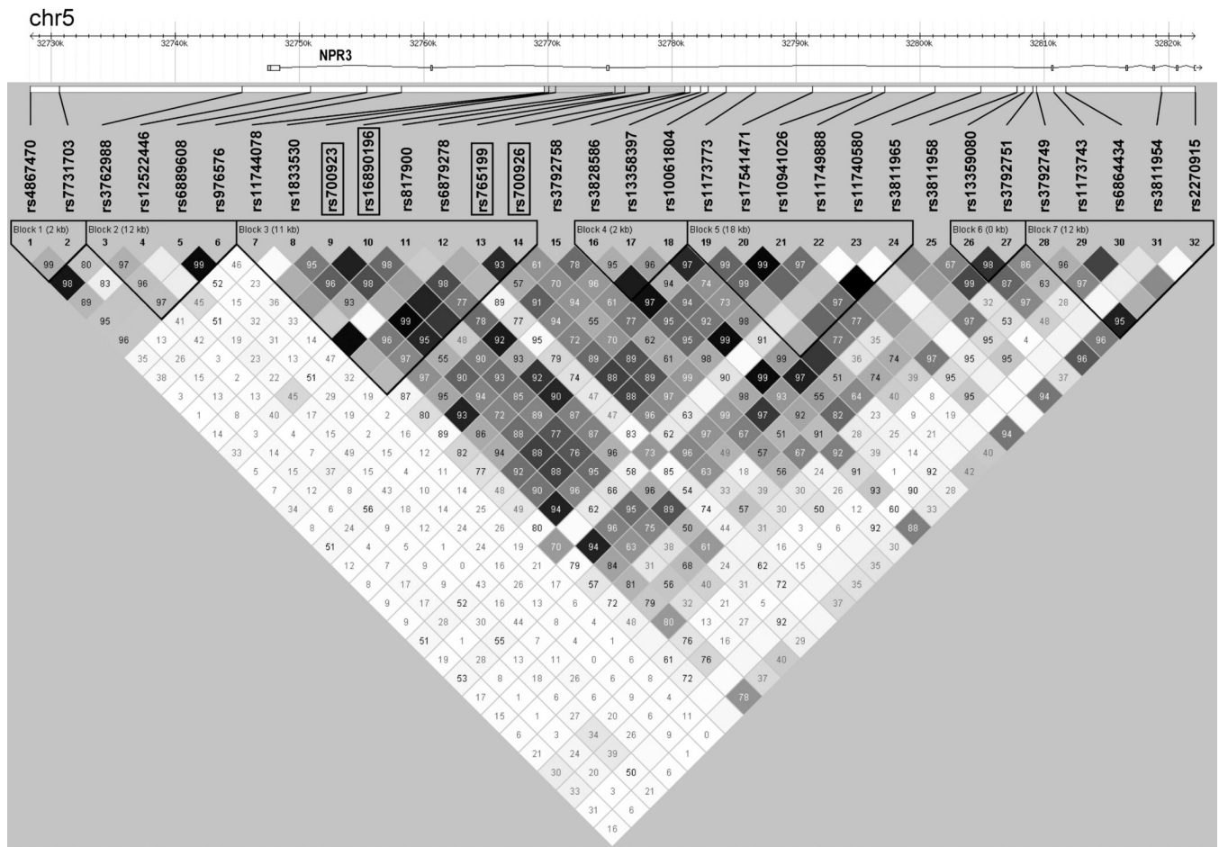
Figure 2. Block structure of linkage disequilibrium for the 32 successfully genotyped single nucleotide polymorphisms (SNPs) in the natriuretic peptide receptor C gene region ( NPR3 ) on chromosome 5p13.3. SNPs surrounded by boxes are the SNPs that were significantly associated with the ventricular dysfunction phenotype after adjustment for clinical covariates and multiple comparisons ( P < 0.05 ). Stronger correlations between SNPs are noted by darker color in the intersecting squares linking each pair of SNPs. Stronger correlation indicates a tendency for the minor allele of one SNP to be inherited with the minor allele of the other SNP that it is being linked with in this figure. Correlations and block structures were estimated using Haploview (version 4.1; The Broad Institute, Cambridge, MA). 30
