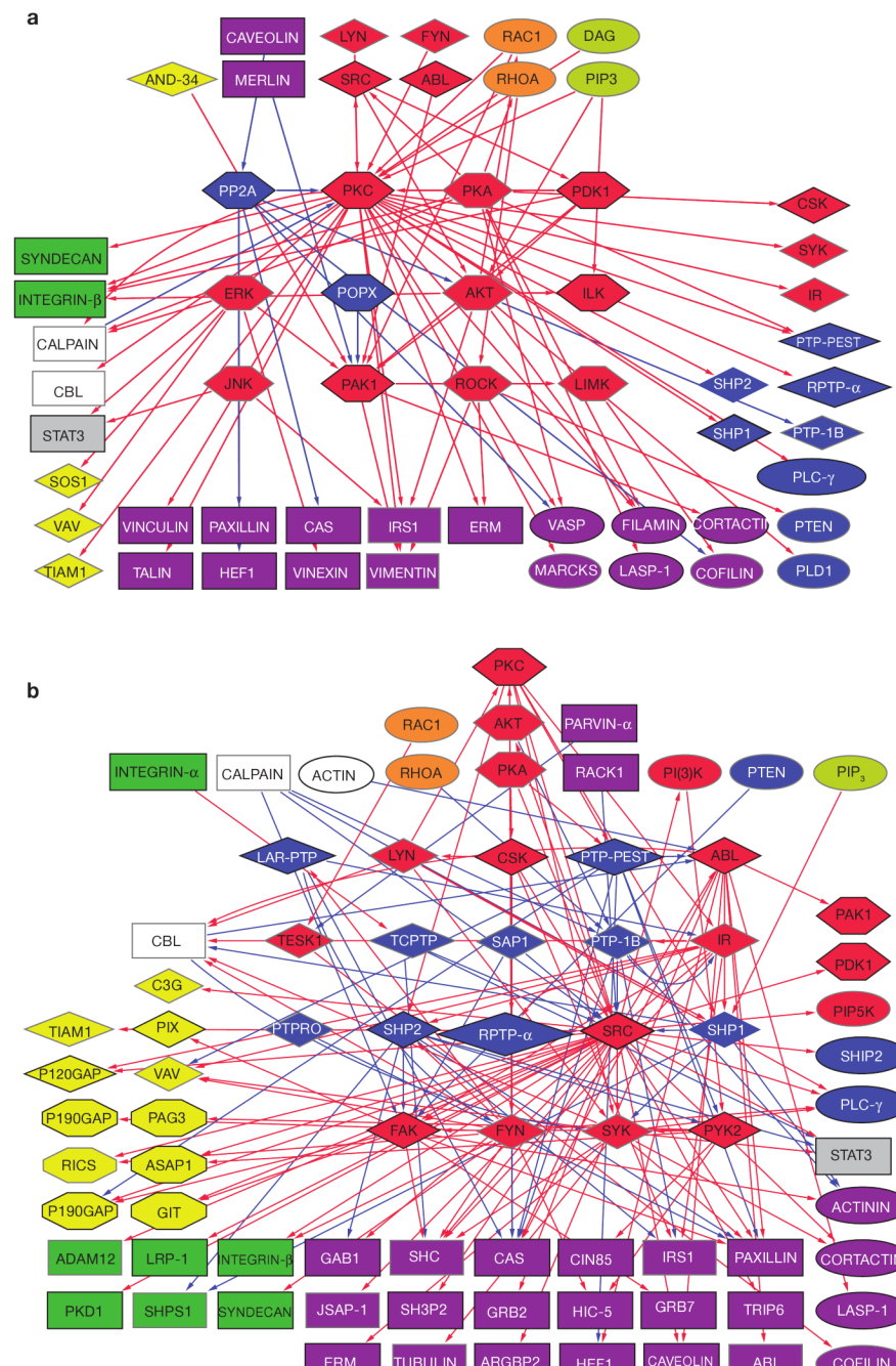
Figure 4. Phosphorylation subnets mapping serine/threonine kinases and phosphatases (a) and tyrosine kinases and phosphatases (b). The figure depicts the corresponding kinases and phosphatases (in the centre), their diverse substrates (bottom and sides) and their regulators (top). The schematic shows hubs of activities (for example, PKC, Src) and a wide variety of substrates. For details see supplementary information, S2.
