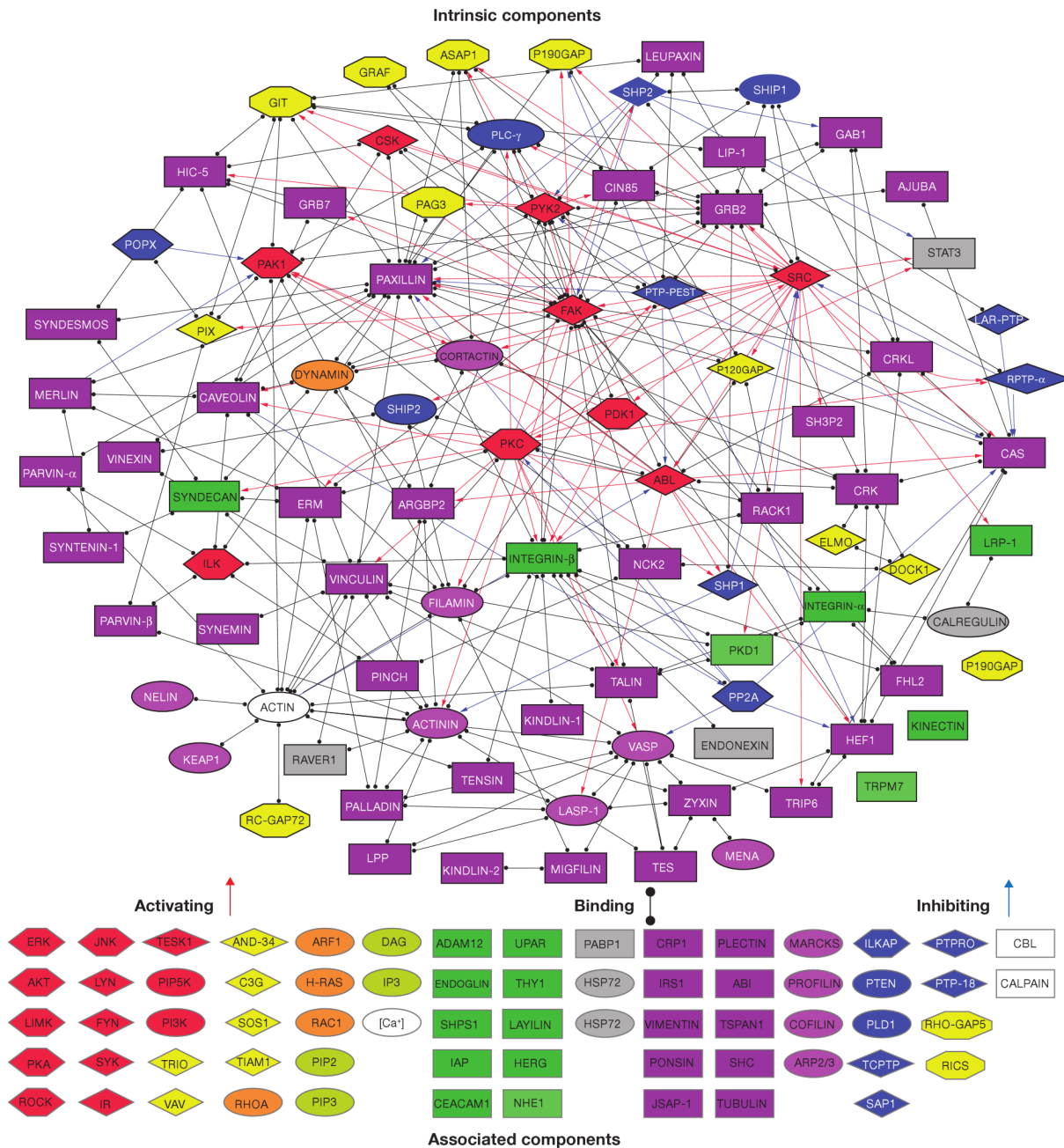
Figure 1. Interactions between all intrinsic components of the adhesome and a grouped list of the associated components. Black lines with full circles at their ends denote non-directional binding interactions, blue arrows represent directional inhibition (for example, dephosphorylation, G-protein inactivation or proteolysis) and red arrows represent directional activation (for example, phosphorylation or G-protein activation) interactions. The nodes are shape- and colour-coded according to the function of the proteins, as detailed in Fig. 2. Intrinsic components are surrounded by a black frame and associated components by a grey frame. For details see supplementary information, S2.
