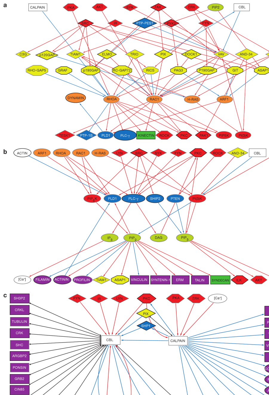
Figure 5. GTPase, lipid and proteolytic subunits. (a) The G-proteins associated with the adhesome (mainly RhoA and Rac1) are shown above their main substrates and below their direct positive (GEFs) and negative (GAPs) regulators. Regulators of the GEFs and GAPs are mainly kinases (top). (b) Signalling lipids are shown with their diverse substrates, the regulatory kinases and phosphatases and their regulators (mainly kinases and G-proteins). (c) The two proteolytic systems associated with the adhesome (Cbl and calpain) affect multiple substrates, and are affected mainly by tyrosine kinases (Cbl) or serine/threonine kinases (calpain). For details see supplementary information, S2.
