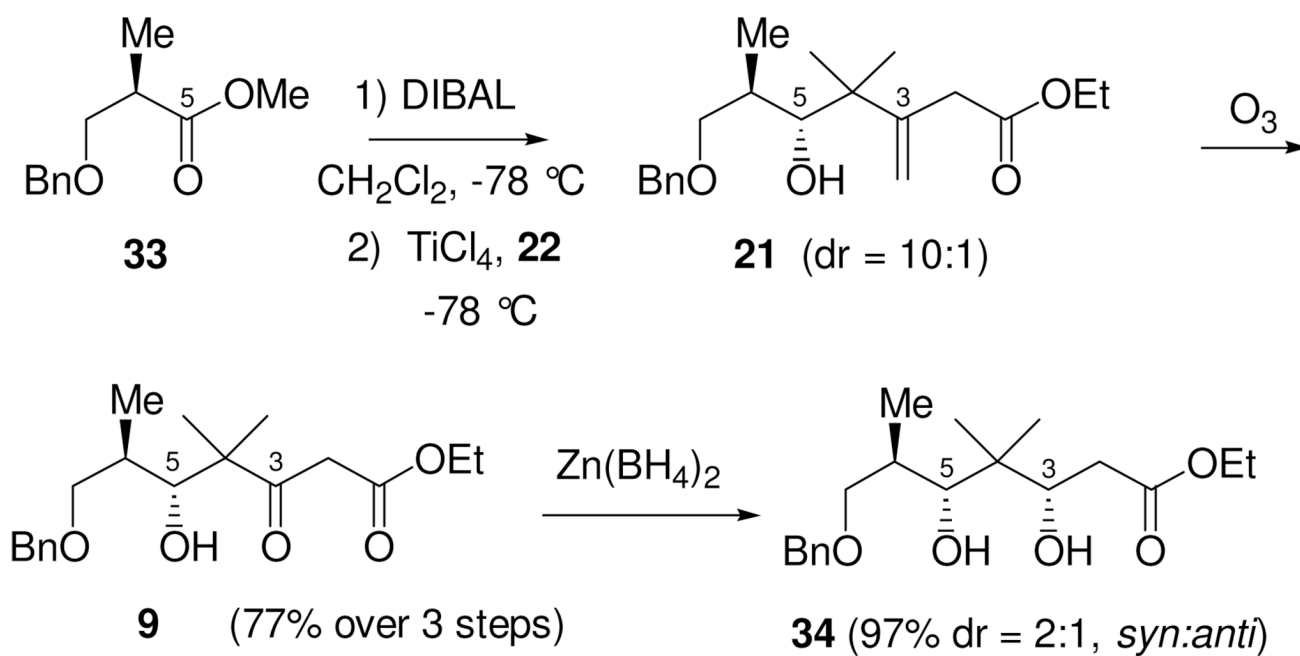
Scheme 9. Synthesis of C 1 -C 7 Diol 34 .
