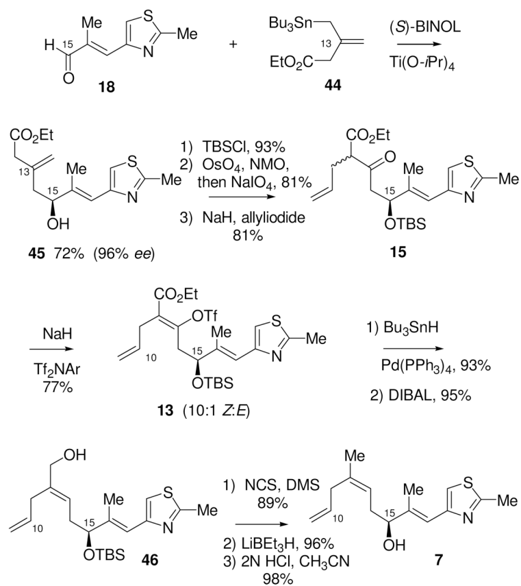
Scheme 14. Preparation of the C 10 -C 21 Alcohol 7
