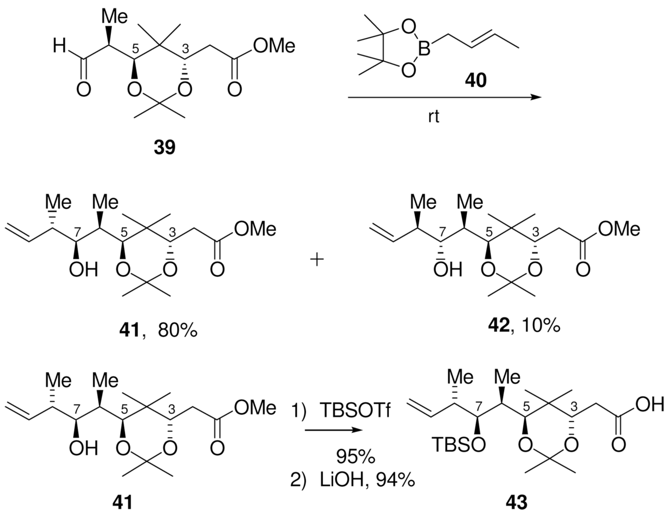
Scheme 13. Synthesis of C 1 -C 9 Acid 43
