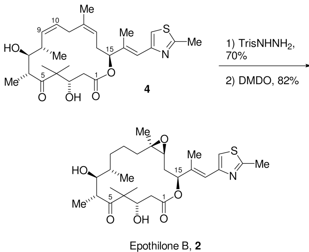
Scheme 27. Completion of the Synthesis of Epothilone B.
