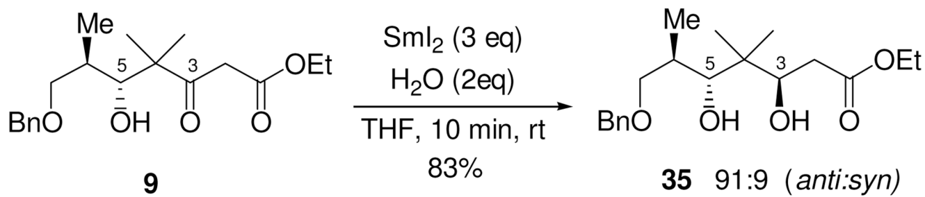
Scheme 10. SmI 2 mediated reduction of β-hydroxy ketone 9
