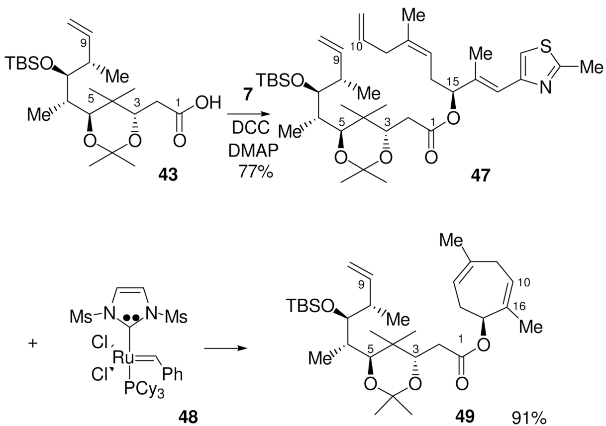
Scheme 15. Ester Coupling and Ring-Closing Metathesis
