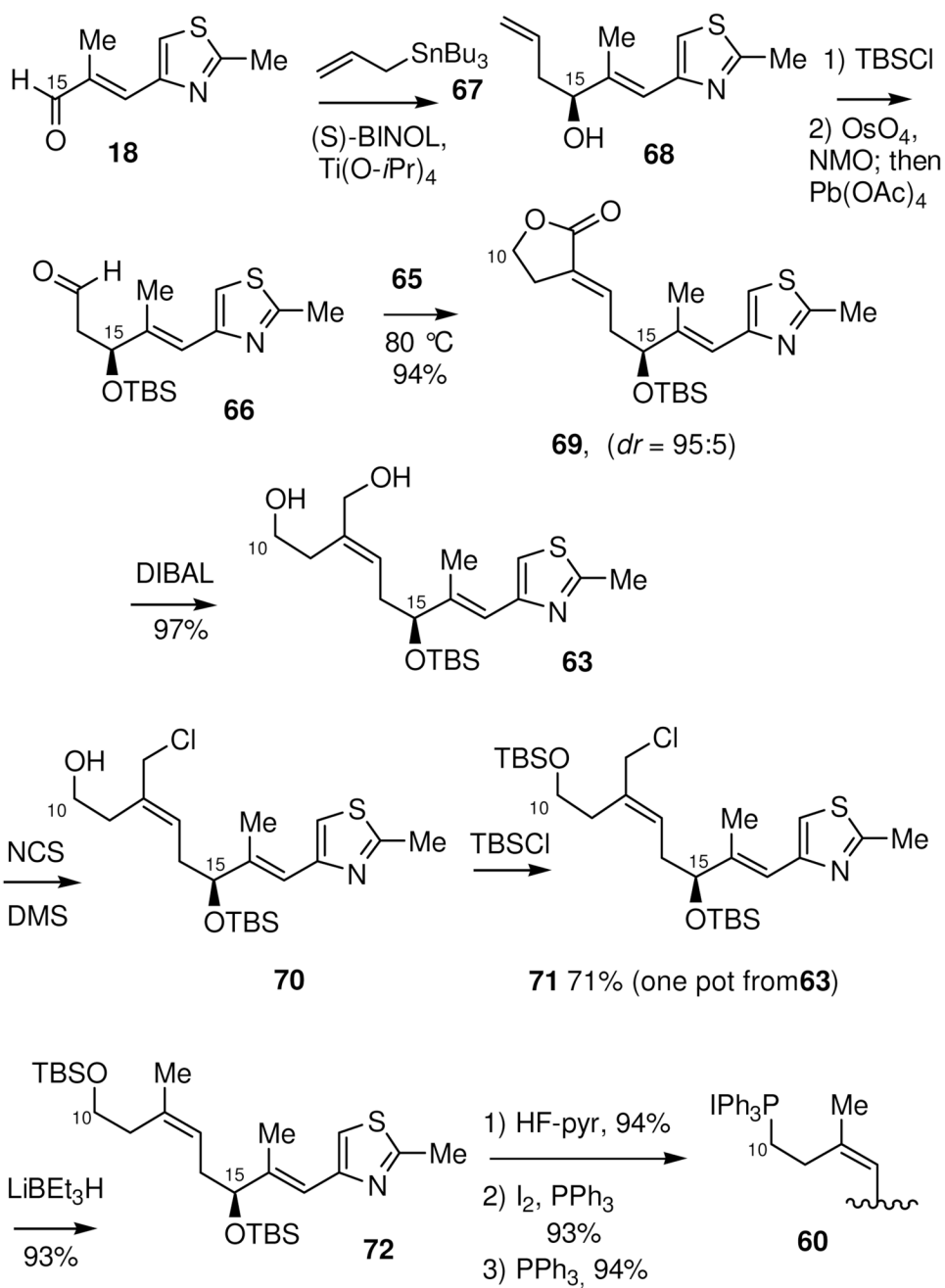
Scheme 20. Preparation of Phosphonium Salt 60
