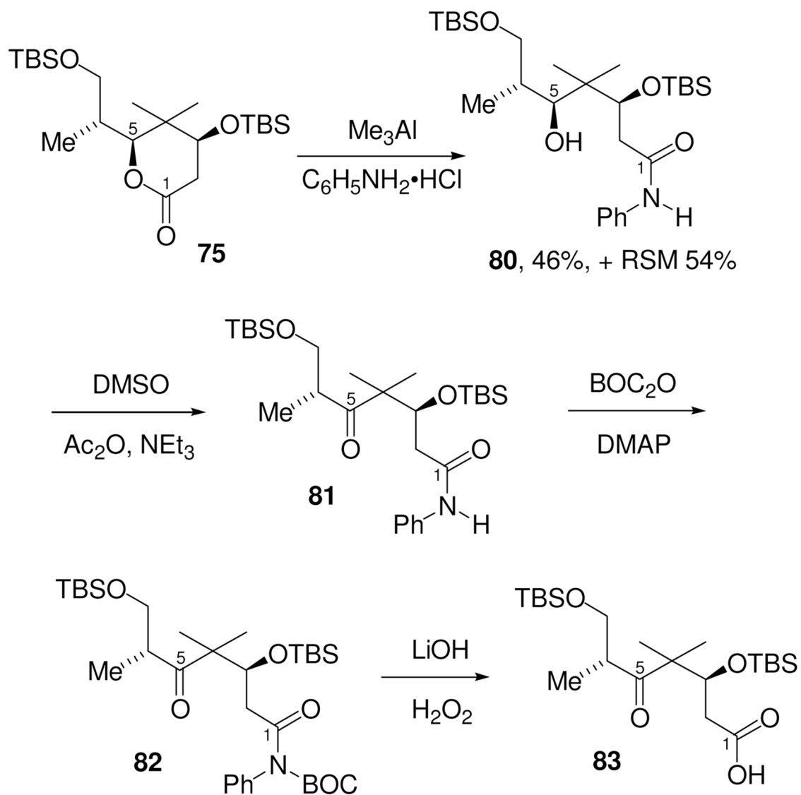
Scheme 24. Aniline Opening of Model Lactone 75
