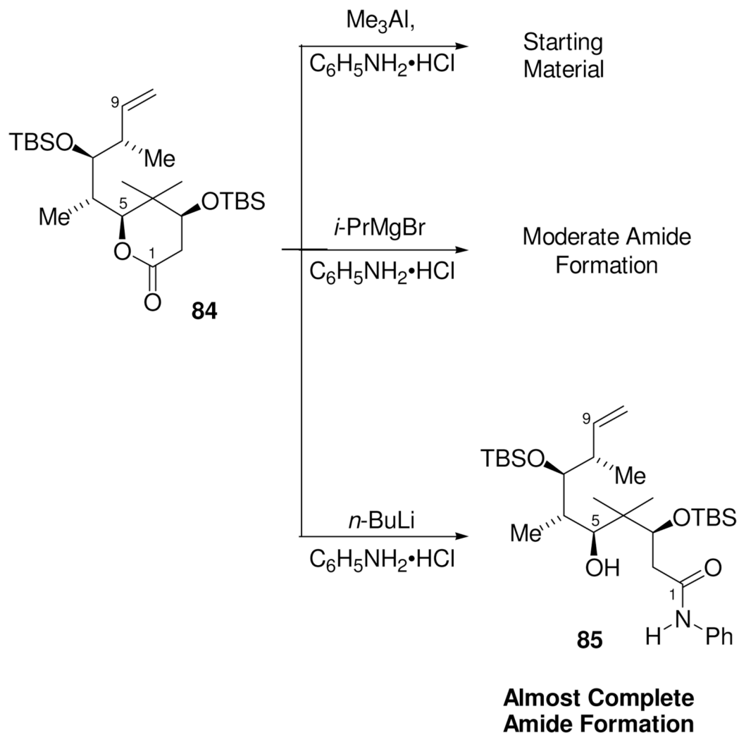
Scheme 26. Lactone Opening with Advanced Model 84 .
