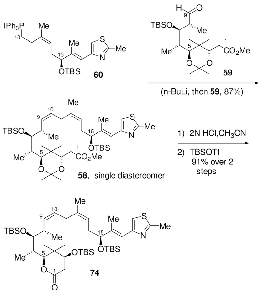
Scheme 22. Synthesis of Lactone 74
