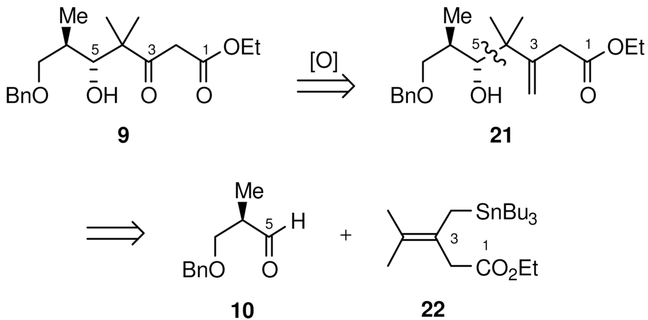
Scheme 5. Stannane Approach to \delta -hydroxy \beta -keto esters
