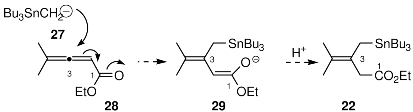
Scheme 7. Approach to Stannane 22
