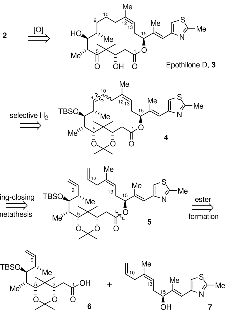
Scheme 1. Retrosynthetic Analysis of RCM Route to Epothilone.
