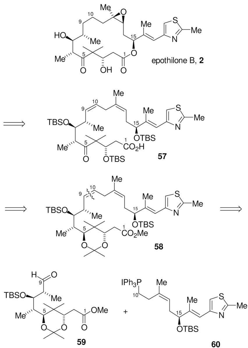
Scheme 17. Revised Retrosynthetic Analysis of Epothilone B.
