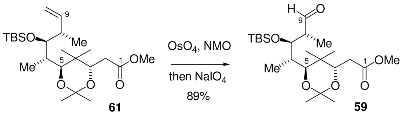
Scheme 18. Preparation of Aldehyde 59
