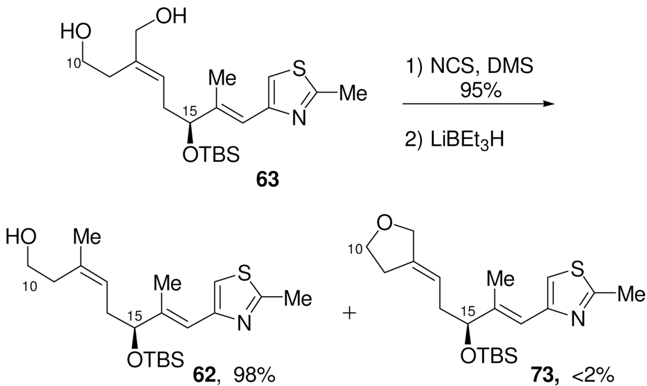
Scheme 21. Selective Allylic Chlorination
