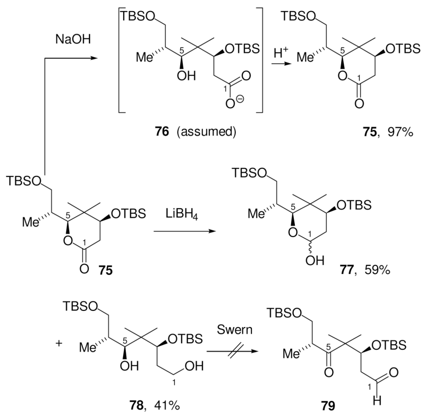
Scheme 23. Attempted Opening of Model Lactone Substrate 75
