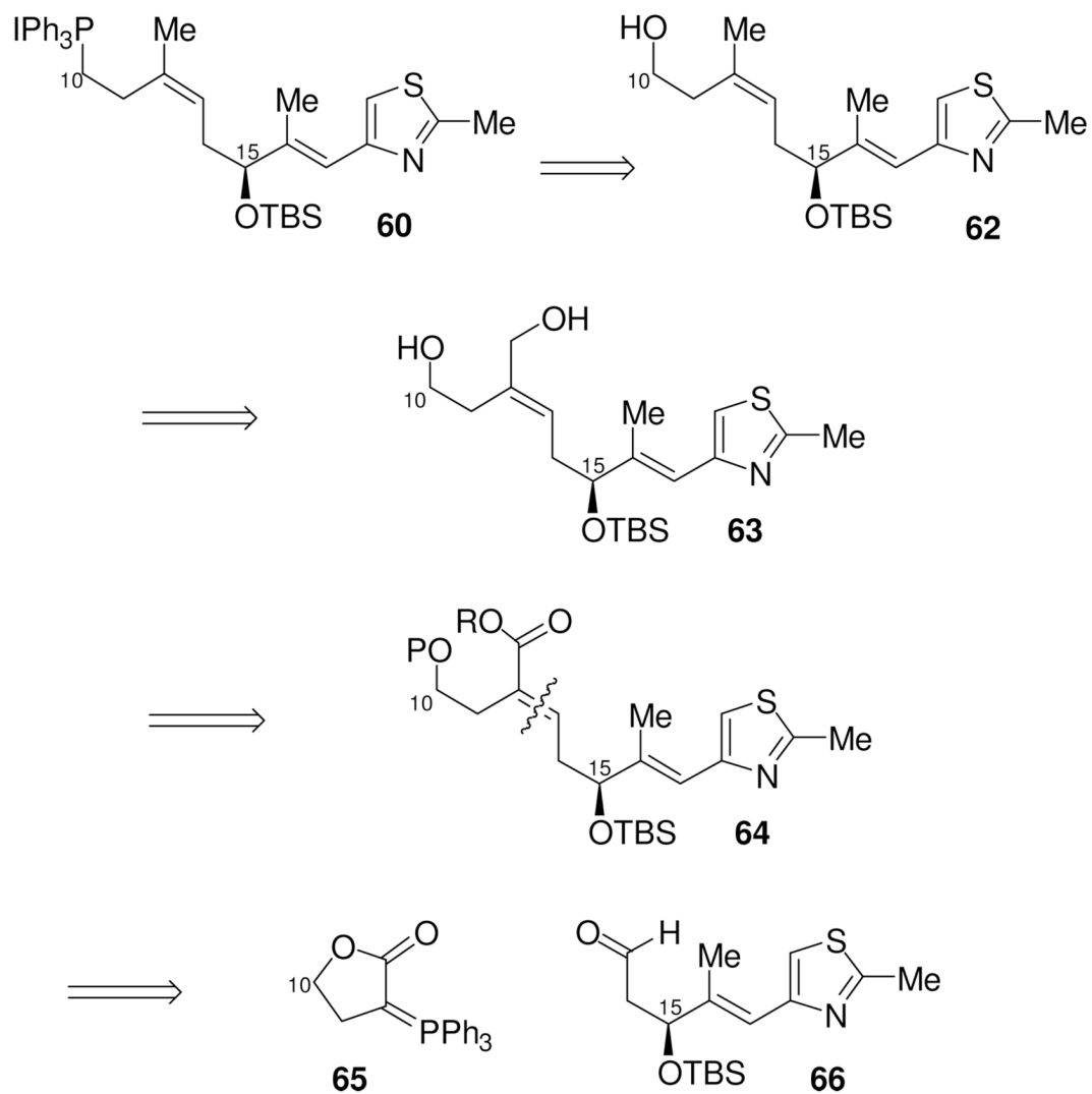
Scheme 19. Retrosynthetic Approach to Phosphonium Salt 60
