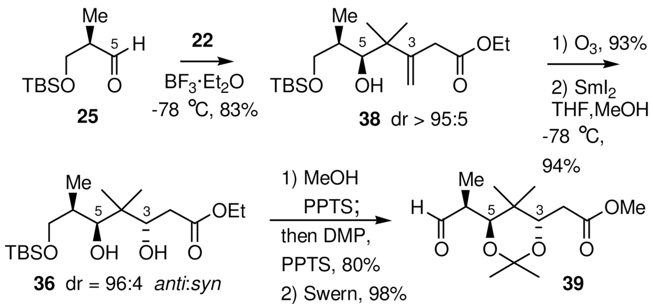
Scheme 12. Synthesis of Aldehyde 39
