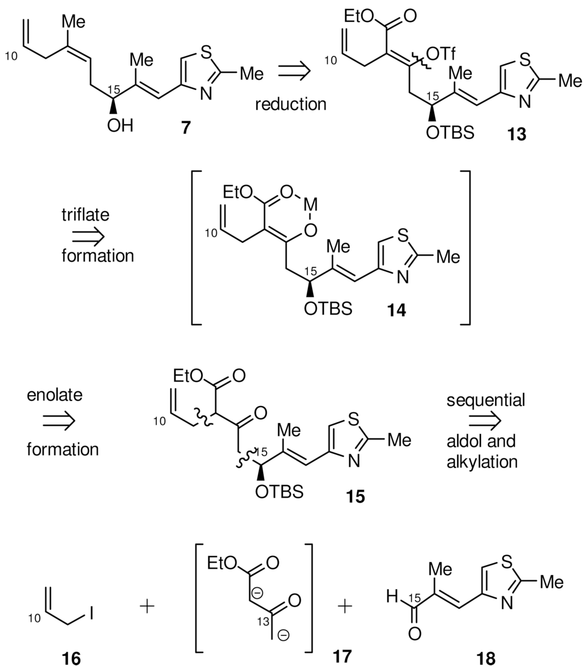
Scheme 3. Retrosynthetic Analysis of the C 10 -C 21 Subunit
