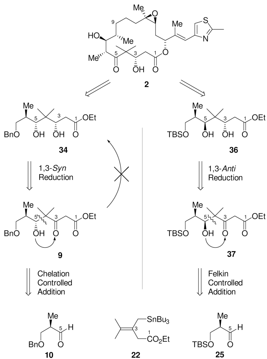
Scheme 11. Second Generation C 1 -C 9 Retrosynthetic Analysis
