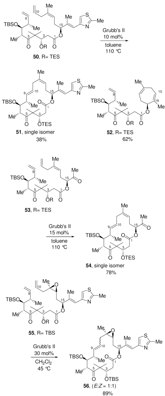
Scheme 16. Other Epothilone RCM Results
