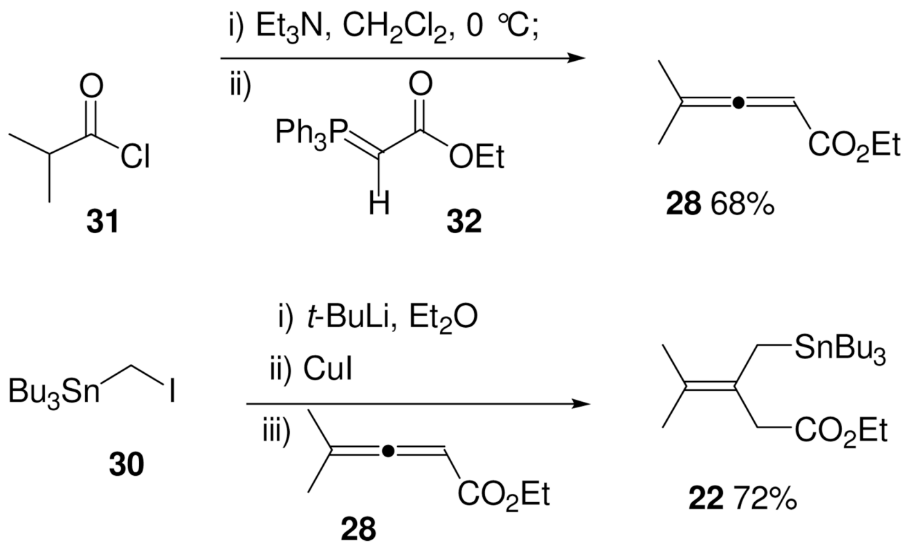
Scheme 8. Synthesis of Stannane 22
