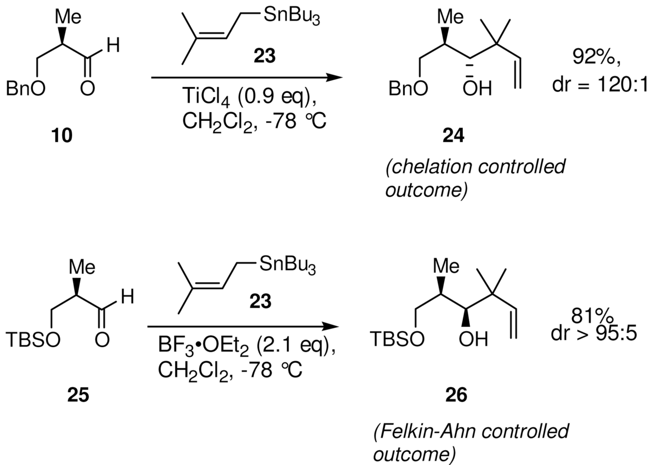
Scheme 6. Prenyl Stannane Additions
