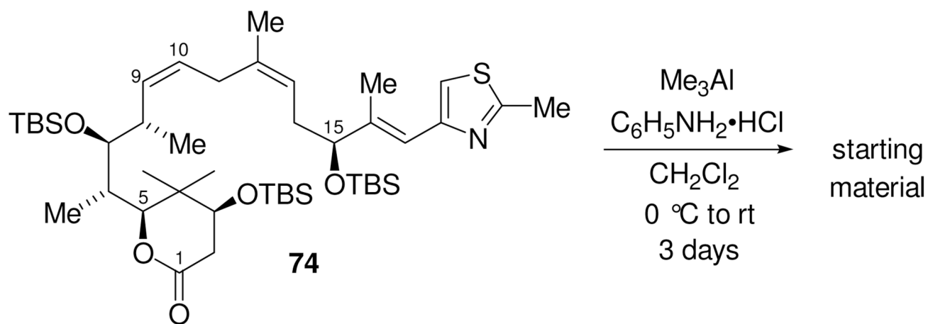
Scheme 25. Attempted opening of lactone 74
