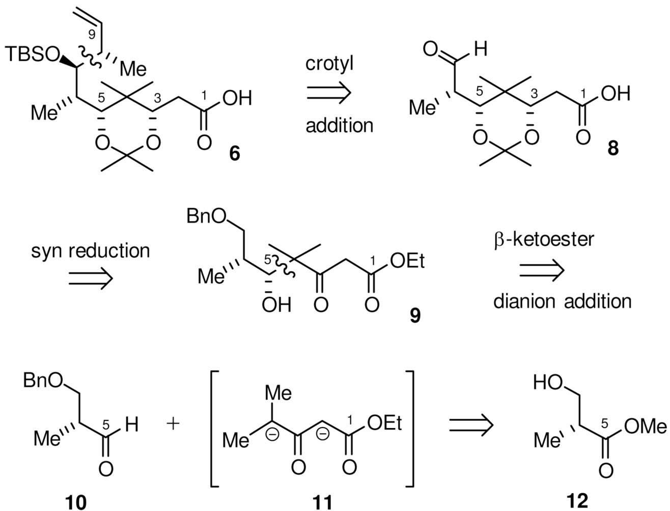
Scheme 2. Retrosynthetic Approach to Acid 6
