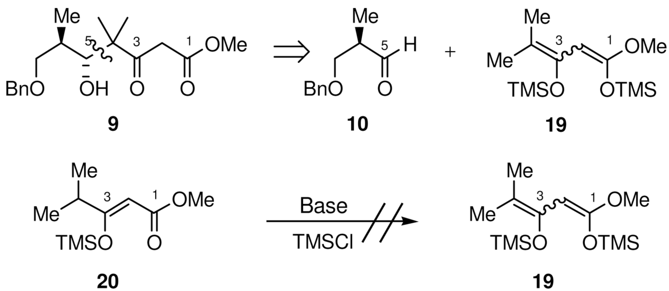
Scheme 4. Potential Chan's Diene Approach
