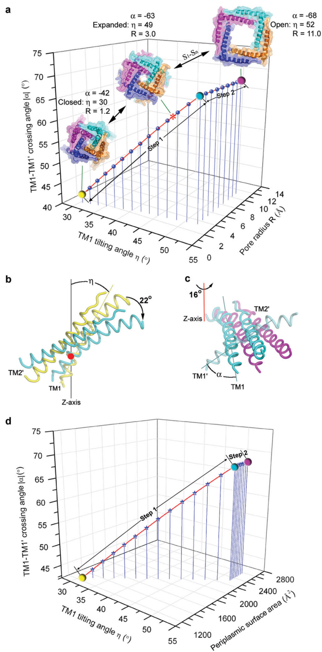
Figure 4. The two-step helix-pivoting model of SaMscL gating
