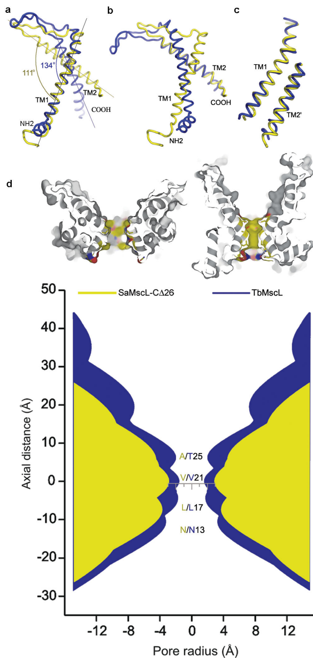
Figure 3. Alignment of SaMscL-C 26 (yellow) and TbMscL (blue)
