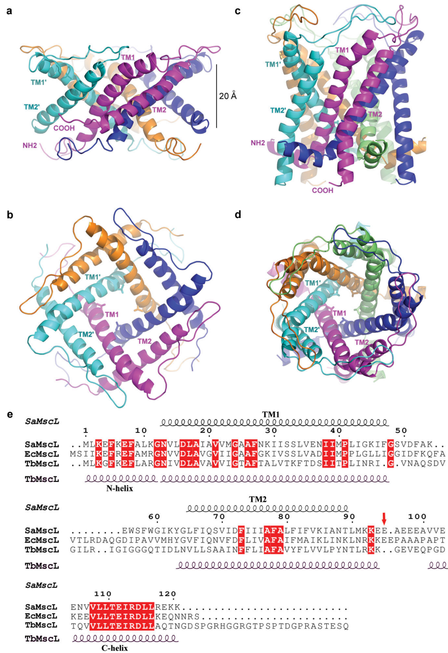
Figure 2. Structures of SaMscL-C 26 and TbMscL
