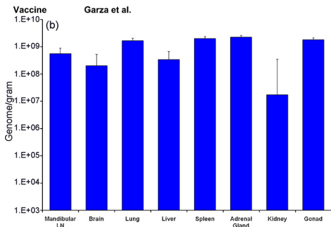
Fig. 3. The changes in whole blood viral load and tissue viral load of rabbits challenged with aerosolized RPXV. (a) Blood samples were collected on day –1, day 2 post-aerosol exposure and every other day through day 14. DNA was isolated from whole blood and used for real-time PCR assay. The graph shows the average whole blood viral load from each group of rabbits, LOD: limit of detection. (b) Necropsies were performed on all of the rabbits that had succumbed to the disease. Selected tissues were collected, processed, and DNA was isolated and used for real-time PCR assay. The graph shows the average tissue viral load from the control group (group 1).
