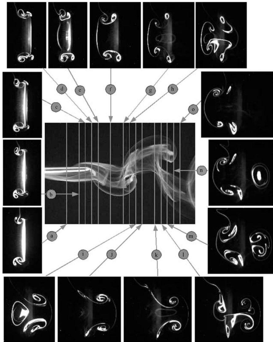
Figure 6. Illuminated (y, z) -planes in the near wake revealing interactions of streamwise vorticity ( \varphi = 22.5^\circ ). Vortex interactions occurring between horseshoes 5 and 6 in planes (a)–(d), horseshoes 4 and 5 in planes (e)–(g), horseshoes 3 and 4 in planes (i)–(k), and horseshoes 2 and 3 in planes (m)–(o). A colour version of this figure may be found at http://gasdyn.princeton.edu .
