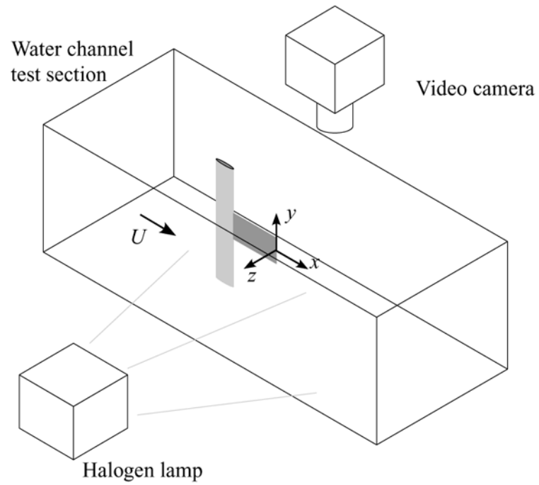
Figure 3. Experimental setup: white-light flow visualization.
