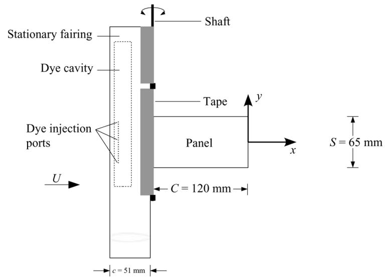
Figure 2. Geometry of panel and fairing assembly.
