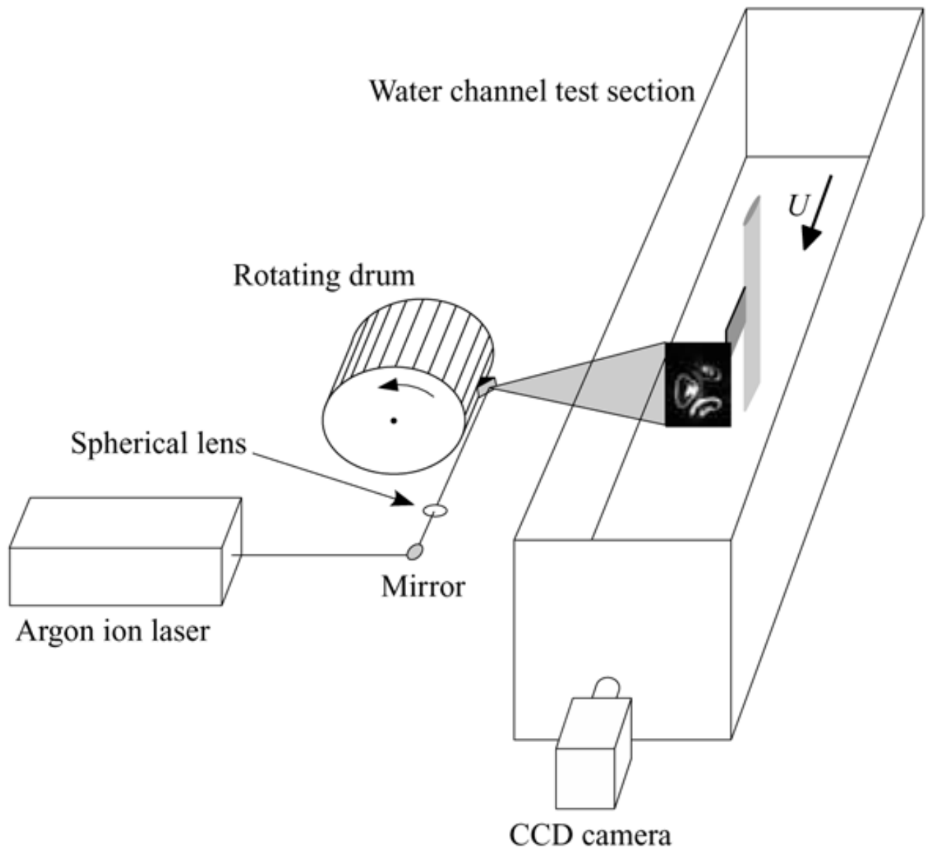
Figure 4. Data acquisition setup with scanning laser beam.
