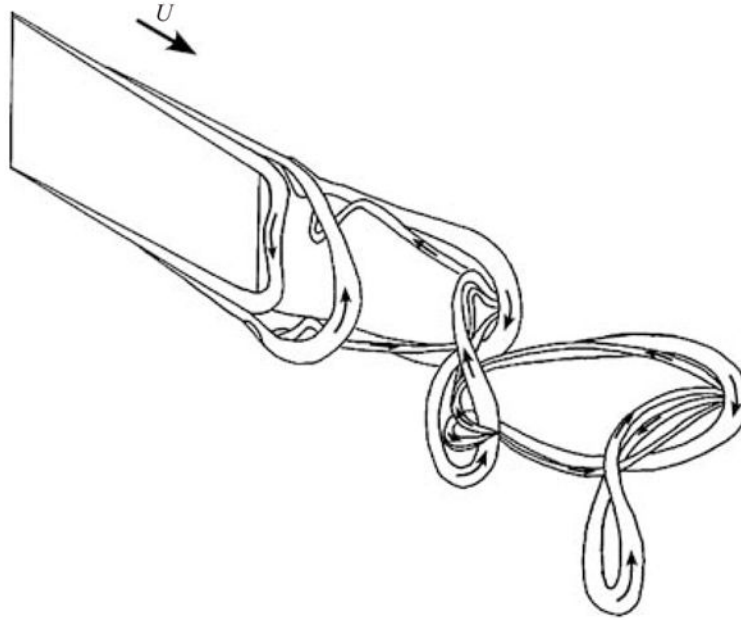
Figure 9. Vortex skeleton model of the wake.
