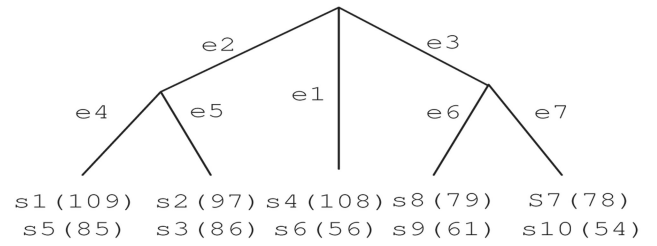
(b) Tree T_{1,8}
