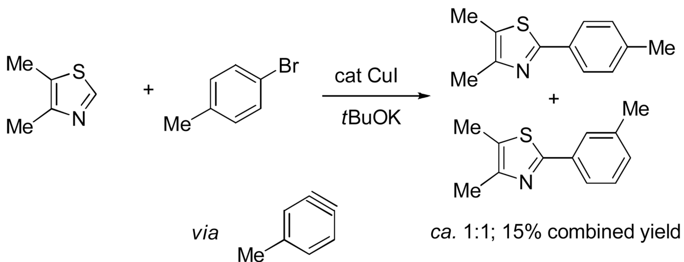
Scheme 3. Benzyne Mechanism
