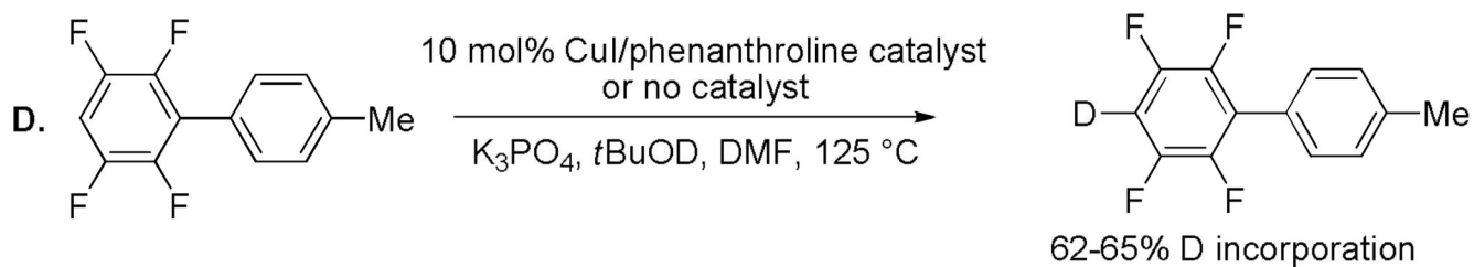
Scheme 4. H/D Exchange Experiments.
