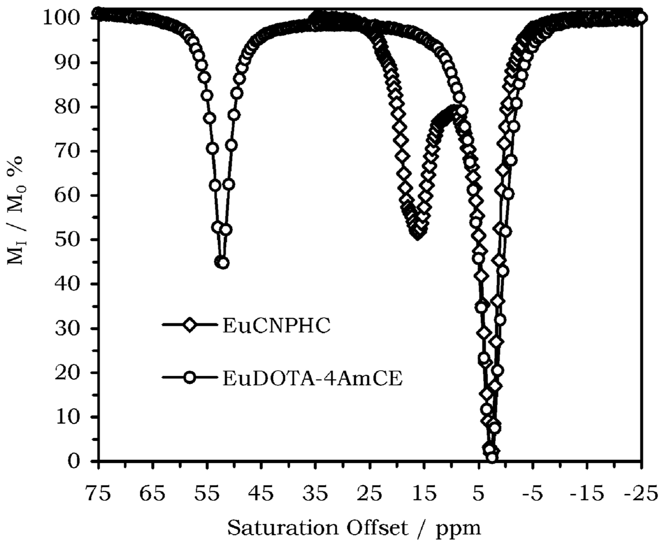
Figure 6. CEST spectra of \text{EuCNPHC}^{3+} (open diamonds) and \text{EuDOTA-4AmCE}^{3+} (open circles) acquired under identical conditions: B_0 = 270 MHz, B_1 = 86 Hz, [\text{H}_2\text{O}]/[\text{EuL}] = 29.25 , T = 296 K, irr. time = 2 s.
