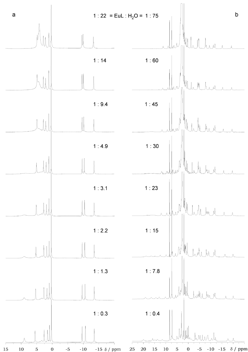
Figure 2. Extended spectral width ^1\text{H} NMR spectra of (a) a 110 mM solution of \text{EuS-THP}^{3+} in dry d_3 -MeCN with progressive addition of \text{H}_2\text{O} and (b) a 35 mM solution of \text{EuCNPHC}^{3+} in d_3 -MeCN with progressive addition of \text{H}_2\text{O} to the solution. The concentration of water in each sample is shown alongside the spectrum.
