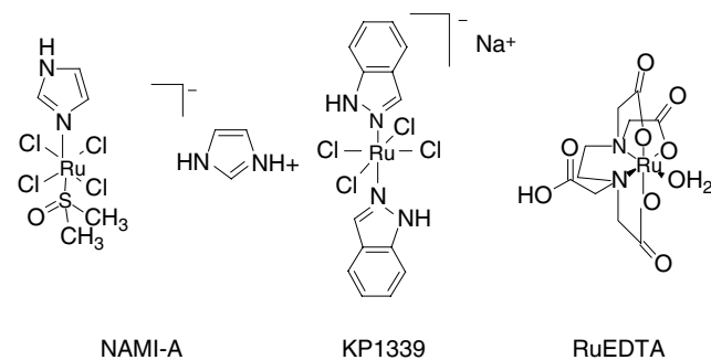
Figure 1 Schematic representation of the chemical structure of NAMI-A, KP1339 and RuEDTA as derived from crystallographic data. Notably, all complexes are characterised by the presence of at least one labile ligand.
