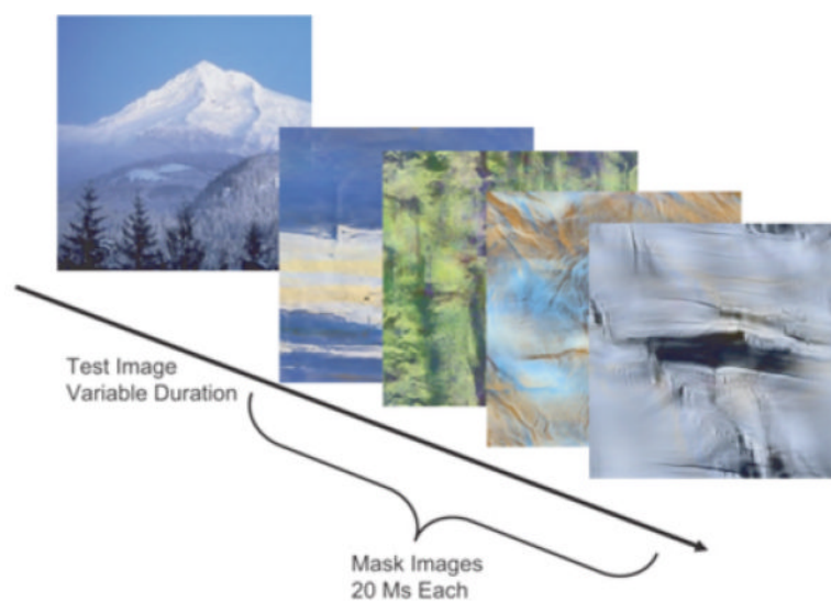
Fig. 2. Illustration of an experimental trial. The presentation duration of each test image was determined using a linear 3-up/1-down staircase, with the first trial of each block presented for 50 ms. Test images were dynamically masked using four colored textures.
