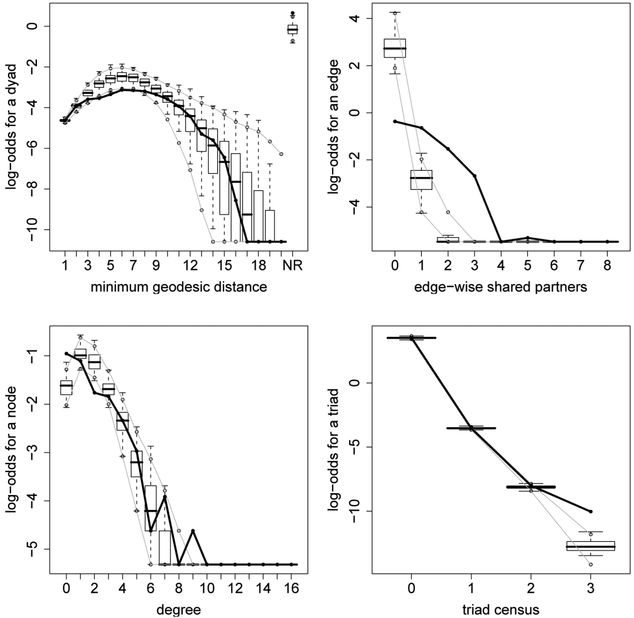
Figure 5. The solid line in each plot represents the observed statistics for the faux.mesa.high network, and the boxplots summarize the statistics for the simulated networks resulting from the MLE.
