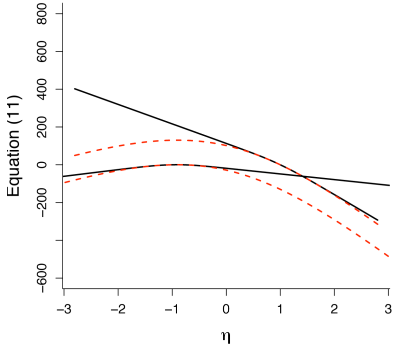
Figure 2. For a simplistic model with g(y) equal to the number of edges, the dotted curves show \ell(\theta) - \ell(\theta_0) for two different values of \theta_0 , namely \theta_0 = 1 (upper curve) and \theta_0 = -1 (lower curve). The solid curves are the corresponding approximations using Equation 11. The true MLE, \hat{\theta} = -0.9072 , is easily derived in this case. Note that \theta_0 = -1 appears to give a good approximation to the loglikelihood near \hat{\theta} , whereas \theta_0 = 1 gives an approximation that cannot even be maximized.
