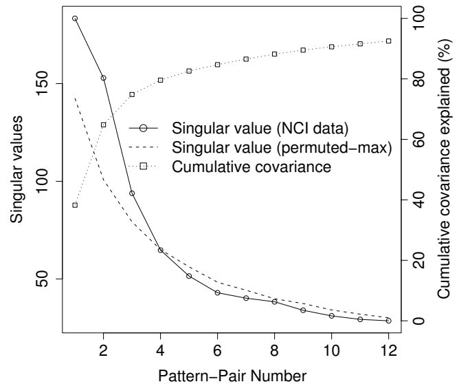
Figure 5 Plots to determine the number of pattern-pairs of the NCI data analysis using CFA. The observed singular values from the NCI data (solid line with circles), maximum singular values from 1000 permutations (broken line) and cumulative covariance (dotted line with squares) profiles of the 1-th to 12-th pattern-pairs.
