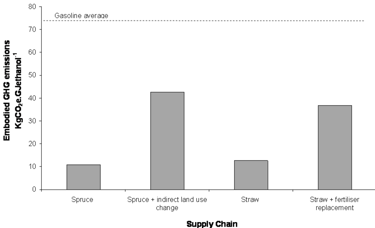
Figure 8 Greenhouse gas emissions for supply chains including consequential impacts (indirect land use change and fertilizer replacement). The example shown assumes an enzymatic hydrolysis process, EU 27 electricity, and that emissions are allocated to ethanol and surplus solid fuel in proportion to their energy content.
