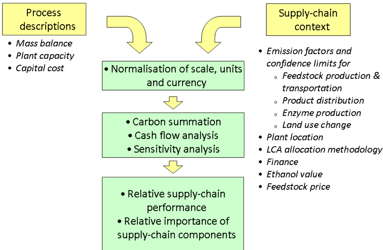
Figure 1 Combined greenhouse gas and cost model schematic.
