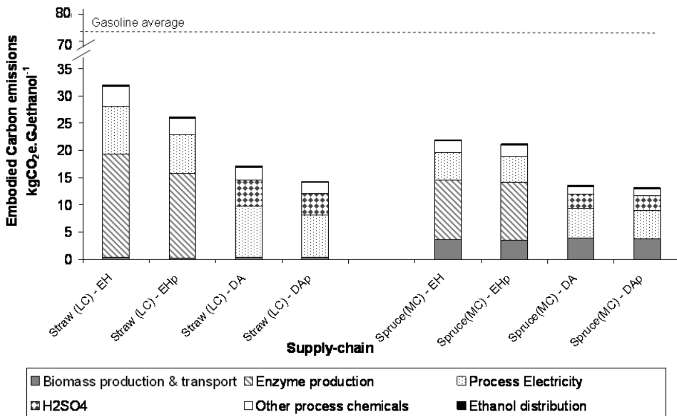
Figure 4 Carbon emissions from ethanol production for base-case supply chains. Greenhouse gas emissions arising from the use of fossil fuels, fertiliser, and so on, are apportioned between ethanol and solid fuel on the basis of energy content.
