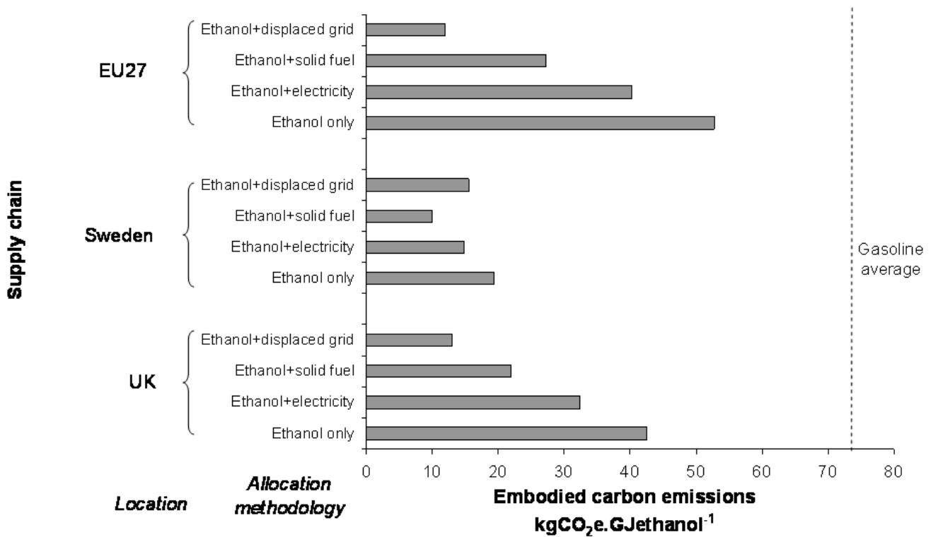
Figure 5 The variation in embodied carbon emissions estimates for alternative allocation methods and locations. The example shown is for the spruce enzymatic hydrolysis supply chain (Spruce-EH).
