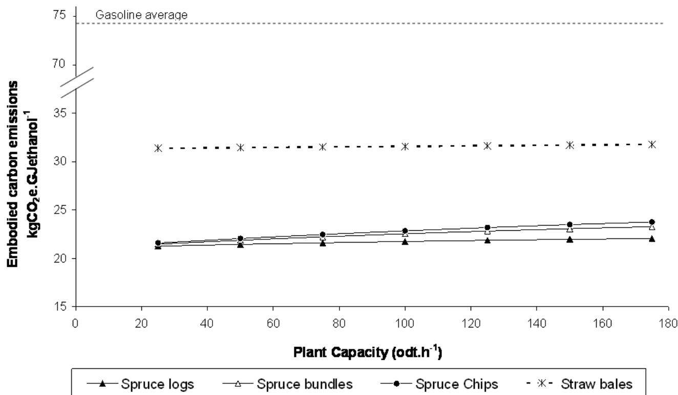
Figure 7 The variation in supply chain greenhouse gas emissions owing to increased transport distances due to increasing plant capacity. The example shown is for the enzymatic hydrolysis process, all fossil carbon emissions are allocated to ethanol and solid fuel in proportion to their energy content.
