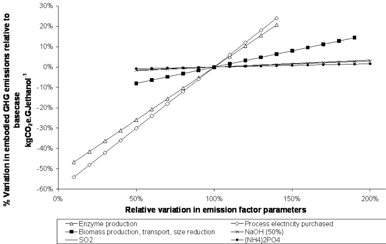
Figure 9 The sensitivity of supply chain greenhouse gas performance to variations in emission factor assumptions – soft-wood enzymatic process. The example shown assumes EU27 electricity, and that emissions are allocated to ethanol and solid fuel in proportion to their energy content.
