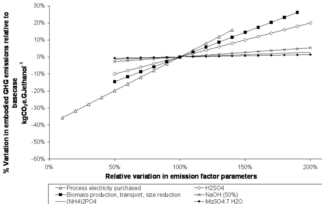
Figure 10 The sensitivity of supply chain greenhouse gas performance to variations in emission factor assumptions – soft-wood dilute acid process. The example shown assumes EU27 electricity, and that emissions are allocated to ethanol and solid fuel in proportion to their energy content.
