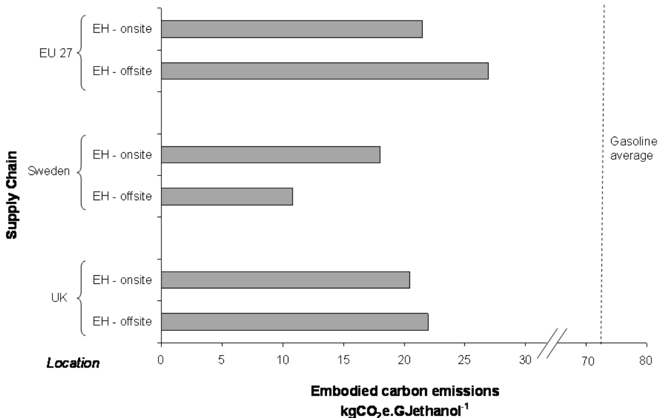
Figure 6 The variation in embodied carbon emission estimates for alternative locations and onsite versus offsite enzyme production. The example shown is for the spruce enzymatic hydrolysis supply chain (Spruce-EH); all fossil carbon emissions are allocated to ethanol and residual solid fuel in proportion to their energy content.
