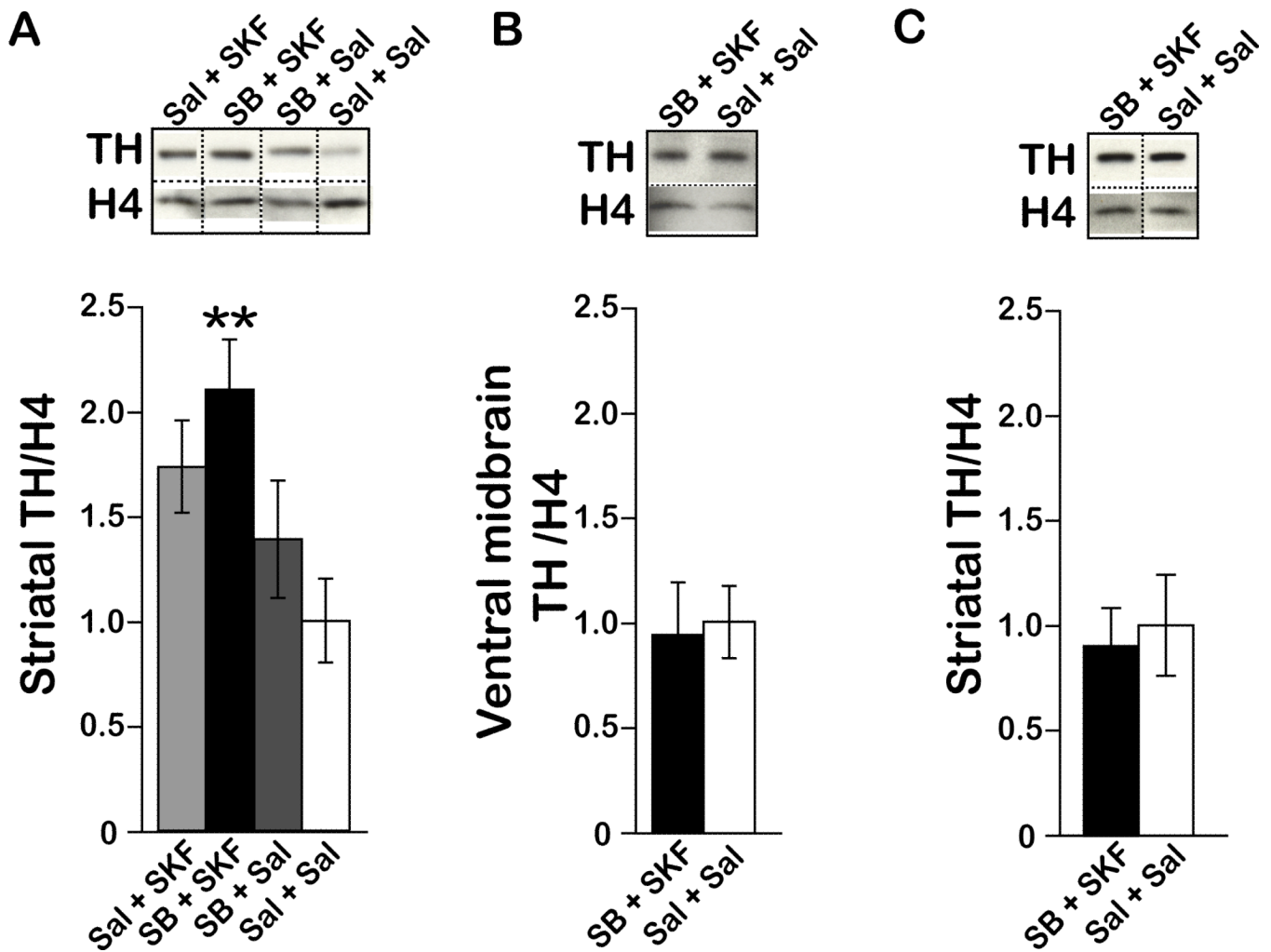
Fig. 3. A transient increase in striatal TH after exposure to D 1 -agonist and HDACi
