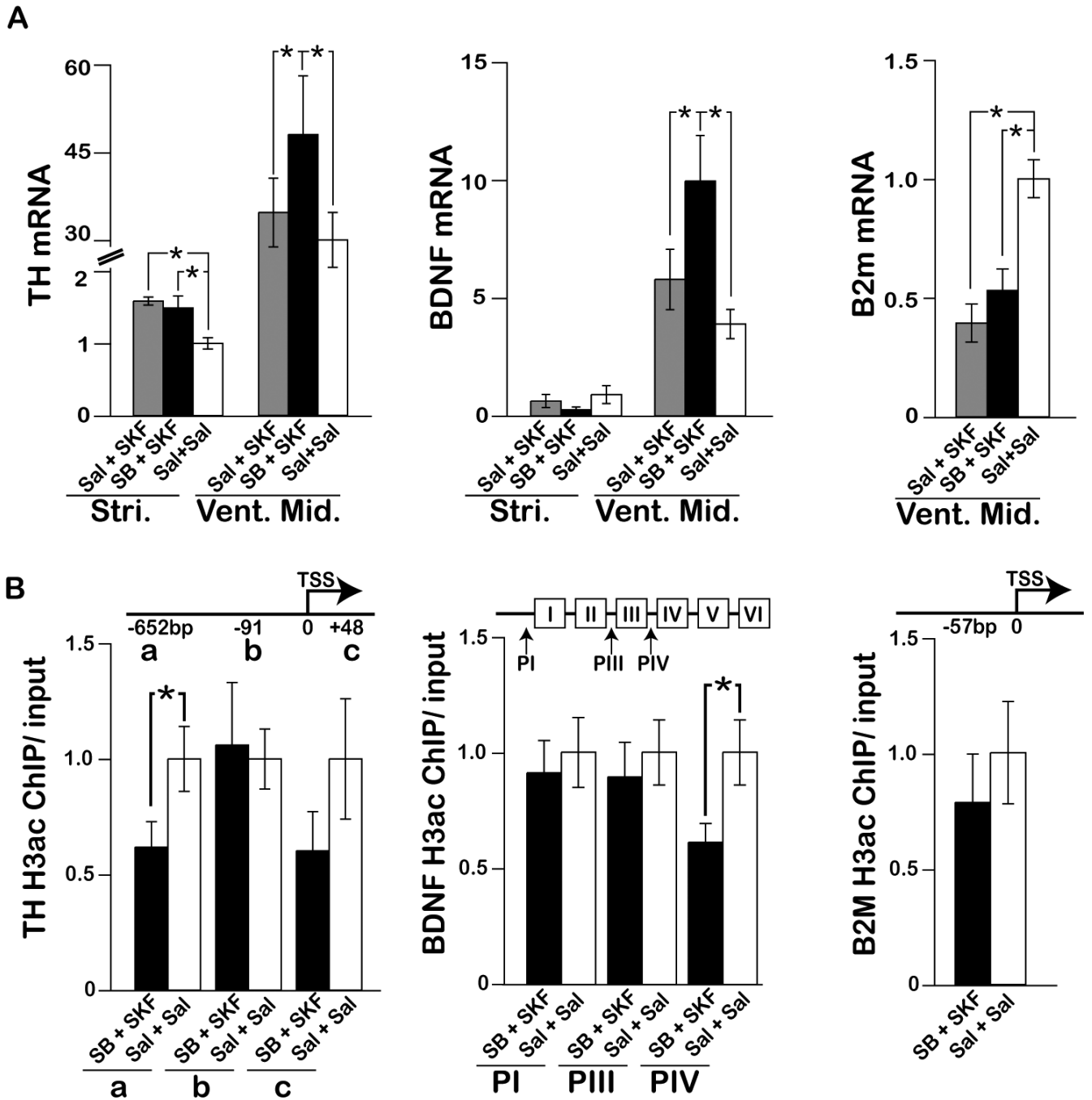
Fig. 2. Treatment with D 1 agonist and HDACi is associated with increased gene expression in ventral midbrain and chromatin remodeling at selected promoter sequences (A) mRNA levels for Th , Bdnf , and B2m from striatum (Stri.) and ventral midbrain (Vent. Mid.) of animals treated for 10 days with Sal+SKF or SB+SKF or SB+Sal or Sal+Sal and sacrificed 30min after last injection. Data from qRT-PCR expressed as mean \pm S.E.M. after normalization to 18S rRNA. Notice that ventral midbrain of animals treated with SB+SKF shows significant increases in Th , Bdnf transcripts compared to Sal+SKF and Sal+Sal. In contrast, ventral midbrain B2m levels were significantly decreased in SKF+/-SB mice. N=5/group/brain region, *, p<0.05; **, p<0.01. (B) Top, schematic presentation of positioning of primer pairs used for ChIP studies at Th , Bdnf and B2m promoters (left graph: Th promoter,
