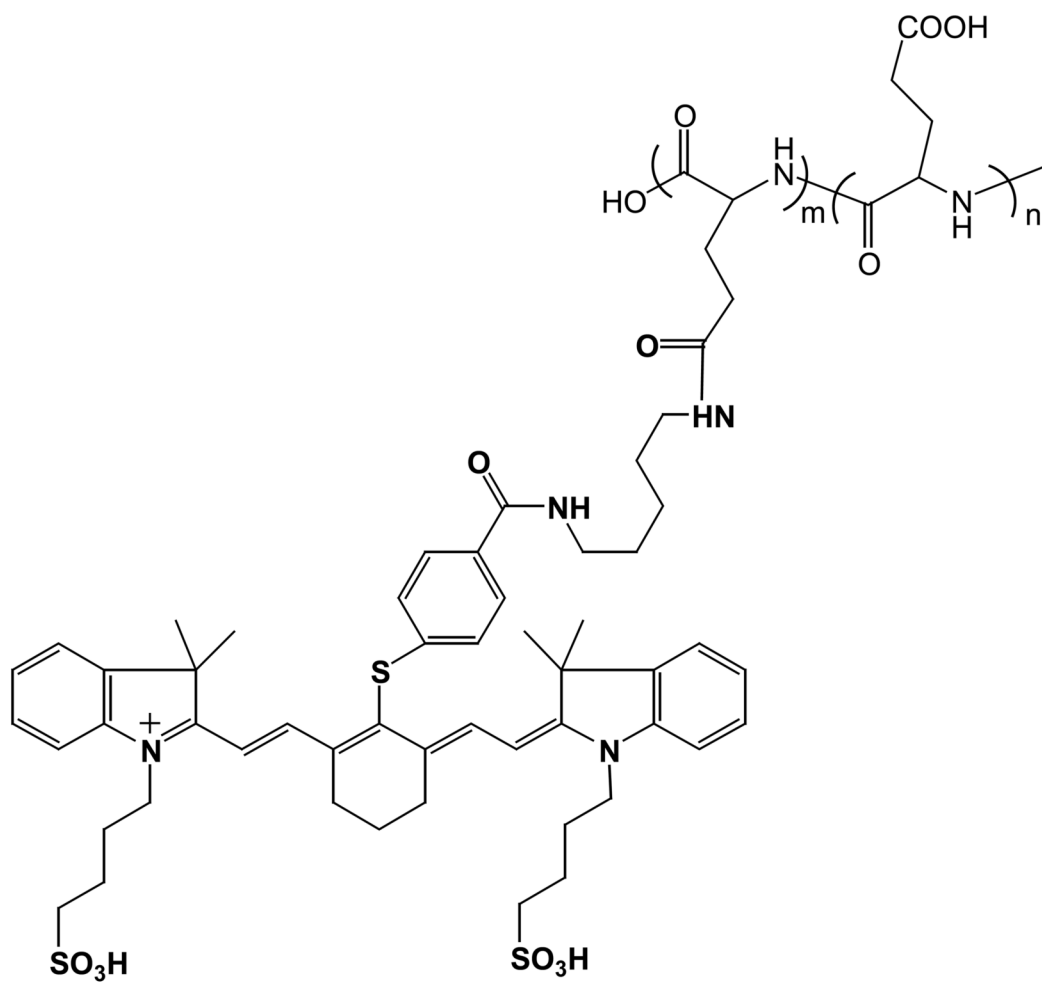
Fig. 1. Structures of PG-NIR813.
