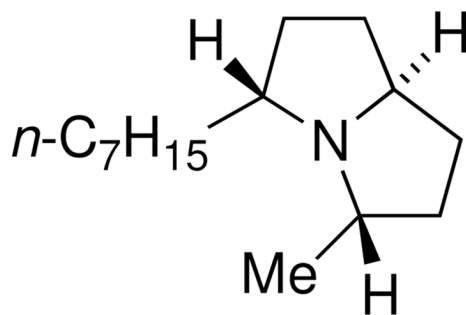
(-)-xenovenine
