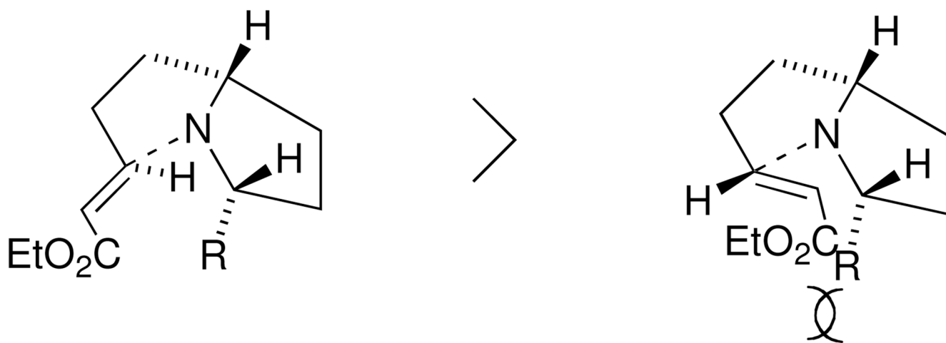
Figure 2. Kinetic control on pyrrolizidine formation
